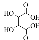
Tartaric acid
