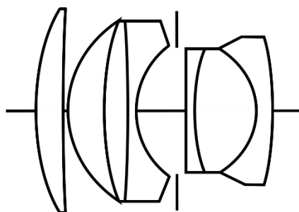
Zeiss Sonnar 50mm f/1.5, 1932
