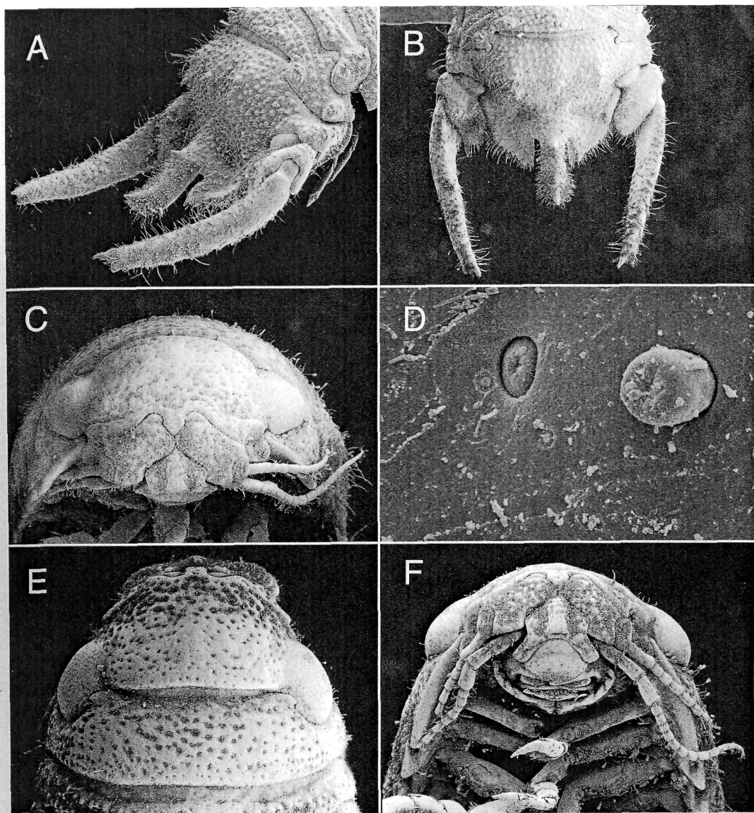
Fig. 4. Discereis kensleyi . Scanning Electron Micrographs: A, male pleotelson, oblique angle; B, male pleotelson; C, frons; D, detail of integument on pleotelson (sensory papillae?); E, cephalon, dorsal view; F, cephalon and frontal lamina, ventral view.
