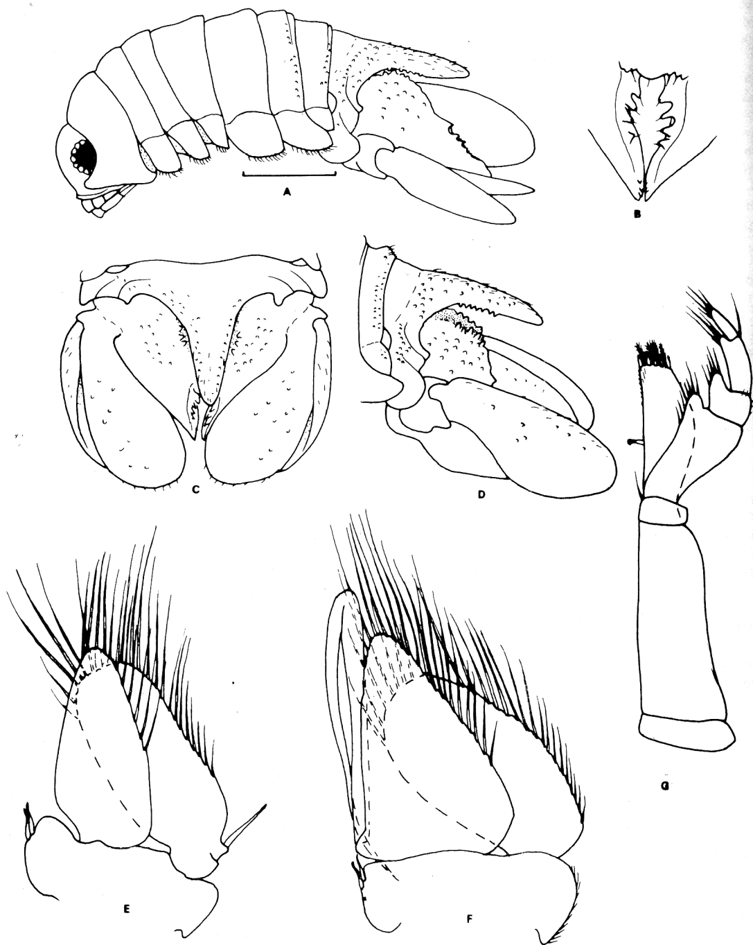
FIG. 1. Dynoides barnardi . (a-c) syntype, 4.6 mm, (d-g) syntype, A.M. P8948 (a) lateral view, (b) pleotelsonic sinus, (c) dorsal view, pleotelson, (d) lateral view, pleotelson, (e) pleopod 1, (f) pleopod 2, (g) maxilliped. Scale line represents 1.0 mm (setules omitted).
