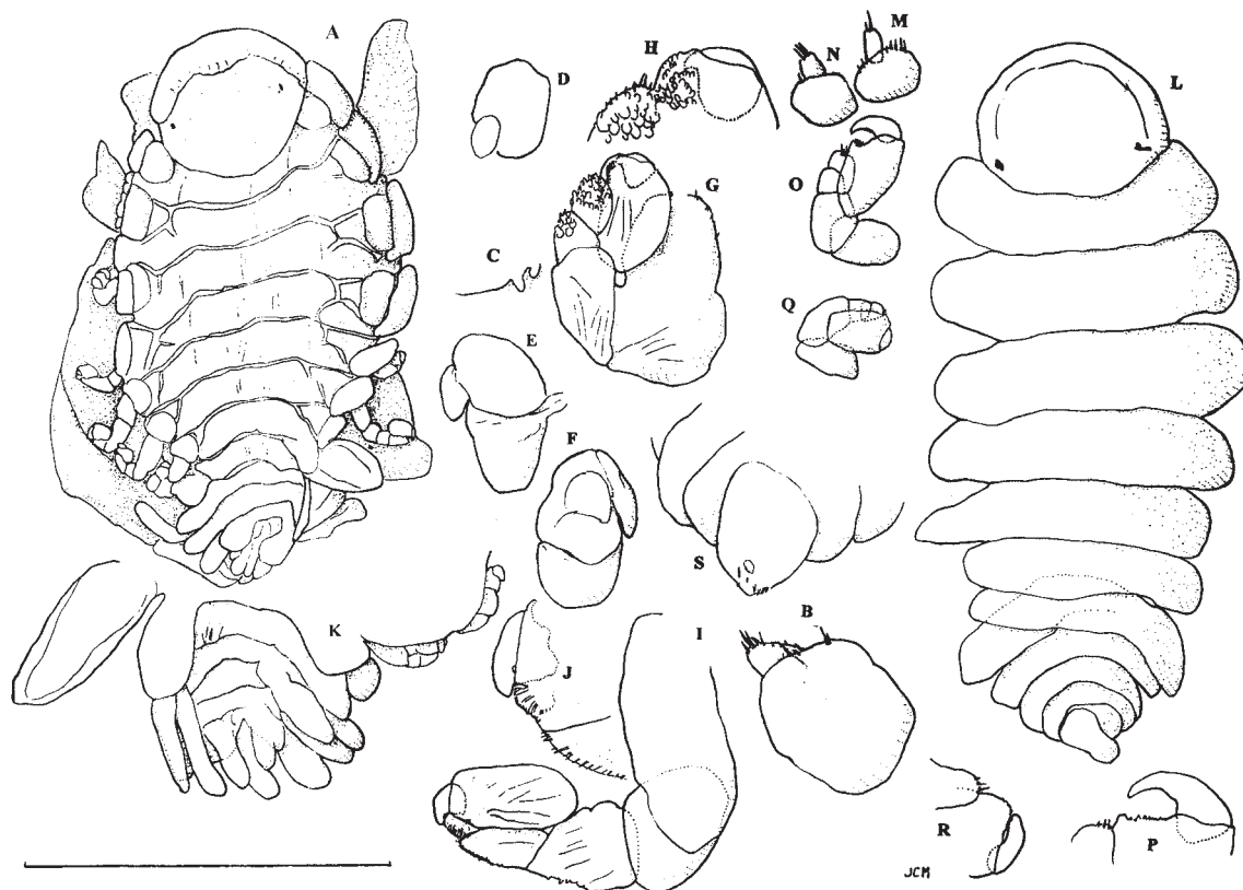
FIG. 1. Anuropodione australiensis Bourdon, 1976. A-K female; L-R male, QM-W10272 A, dorsal view. B, right antenna 1. C, left side of barbula. D, right maxilliped, external view. E, right oostegite 1, external. F, same, internal. G, right pereopod 1. H, distal region of same. I, right pereopod 7. J, distal region of same. K, pleon, ventral. L, dorsal view. M, right antennae. N, left pereopod 1. O, distal region of same. P, left pereopod 7. Q, distal region of same. R, posterior end of pleon, ventral. Scale: 1.84 mm for A, C-F; 1 mm for K; 0.32 mm for B, G, I, L, O, Q; 0.16 mm for H, J, M, N, P, R, S.
