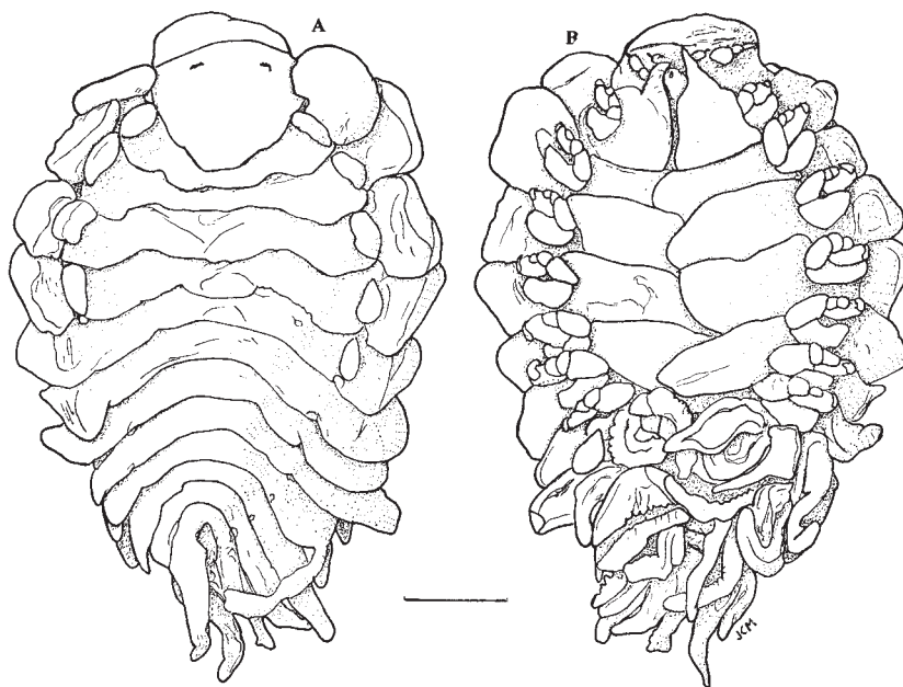
FIG. 25. Parapenaeon expansa Bourdon, 1979, immature female, QM-W10442. A , dorsal view. B , ventral view. Scale: 2.0 mm.
