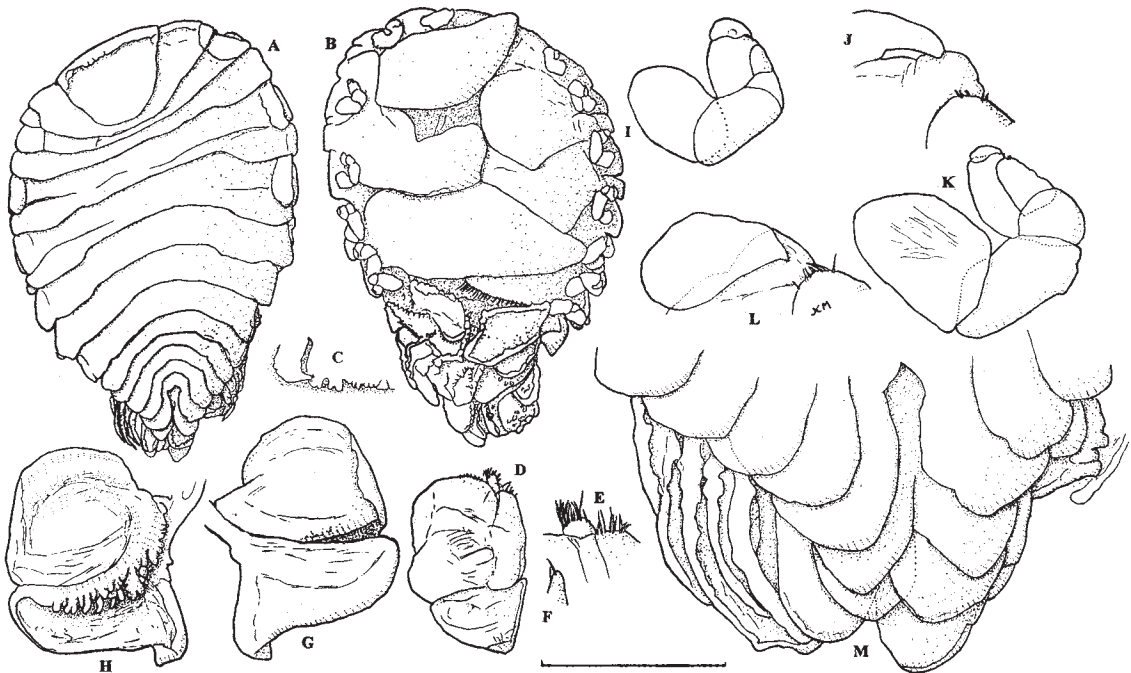
FIG. 22. Parapenaeon expansa Bourdon, 1979, female, QM-W17450. A, dorsal view. B, ventral view. C, left side of barbula. D, right maxilliped. E, palp of same. F, plectron of same. G, right oostegite 1, external. H, same, internal. I, right pereopod 1. J, distal edge of same. K, right pereopod 7. L, distal edge of same. Scale: 4.35 mm for A, B; 2.0 mm for C, D, G, H; 1.1 mm for E, F, I, K; 1 mm for M; 0.18 mm for J, L.
