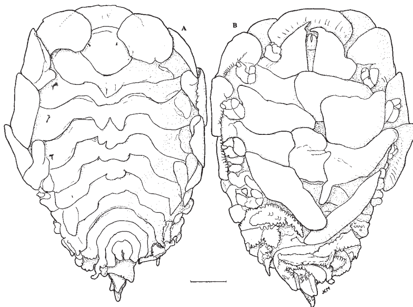
FIG. 23. Parapenaon expansa Bourdon, 1979, female, QM-W12031. A, dorsal view. B, ventral view. Scale: 2.0 mm.
