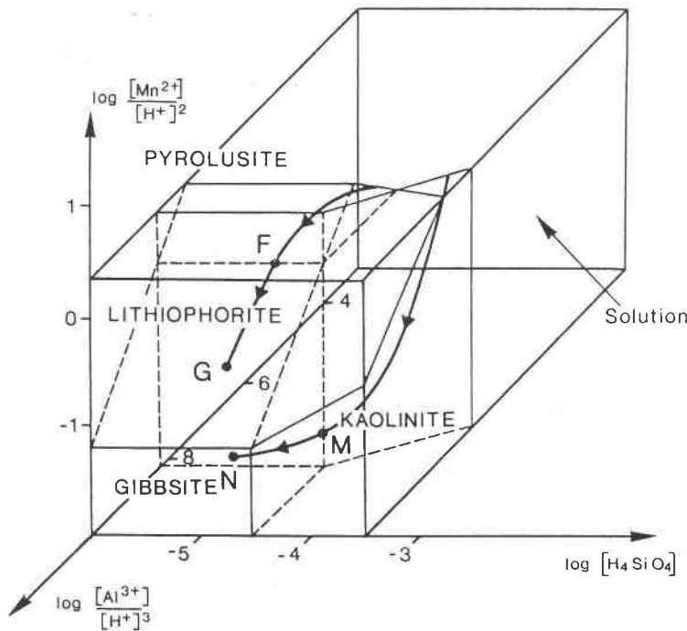
Fig. 8. Three-dimensional stability-field diagram ( \log[Mn^{2+}]/[H^+]^2 vs. \log[H_4SiO_4] and \log[Al^{3+}]/[H^+]^3 ) for pyrolusite, lithiophorite, gibbsite, and kaolinite at 25 °C and \log f_{O_2} = -0.68 , using the following solubility products: \log K_{py} = 0.02 , for pyrolusite; \log K_{li} = 15.5 , for lithiophorite; \log k_{gi} = 8.205 , for gibbsite; \log K_{ka} = 7.41 , for kaolinite. The arrows show two different pathways that represent common chemical evolution of natural solution.
