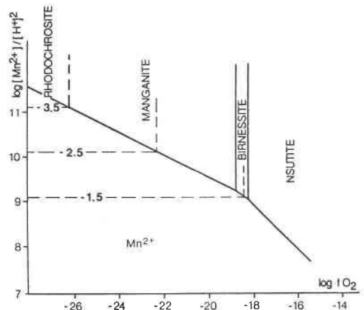
Fig. 6. Stability fields of nsutite ( Mn_{0.95}^{IV}Mn_{0.05}^{III}O_{1.95}(OH)_{0.05} ) and birnessite ( Mn_4^{IV}Mn_3^{III}O_{13} \cdot 5H_2O ) at 25 °C and 1 atm (for \log K_{nsu} = 0.68 and for \log K_{bir} = 8.63 ). The tie-lines represent the different limits of the rhodochrosite stability field as a function of \log f_{CO_2} .
