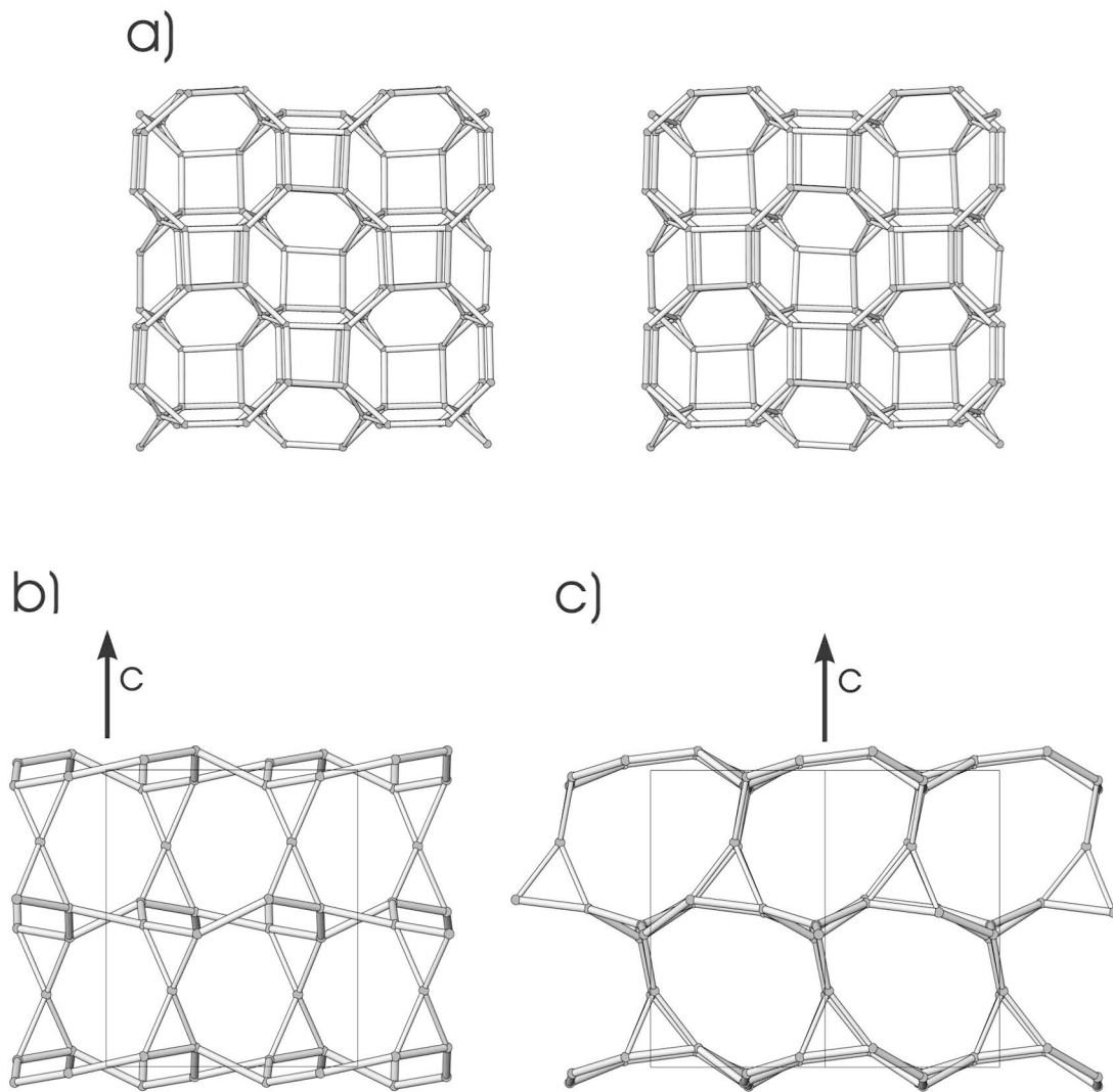
FIG. 6. Nabesite framework (a) in a stereographic view along [001], as well as in projections along (b) [100] and (c) [110].
