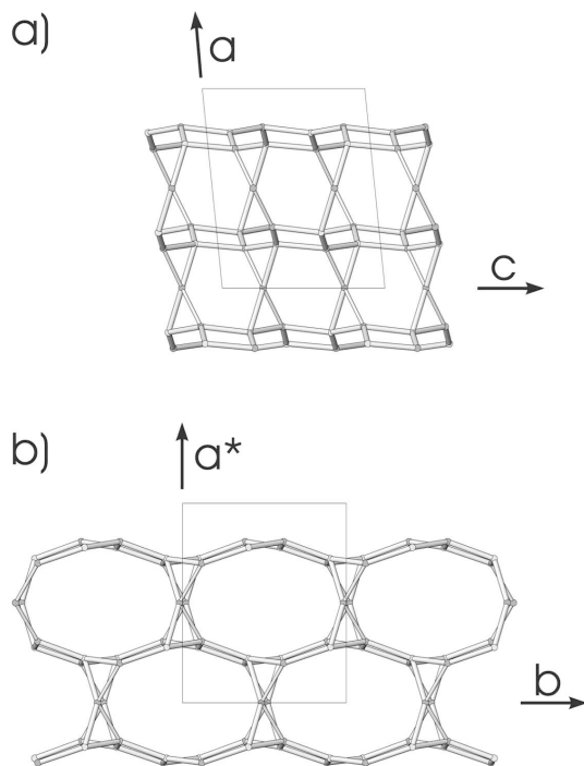
FIG. 7. The framework of weinebeneite in projections along (a) [010] and (b) [001].
