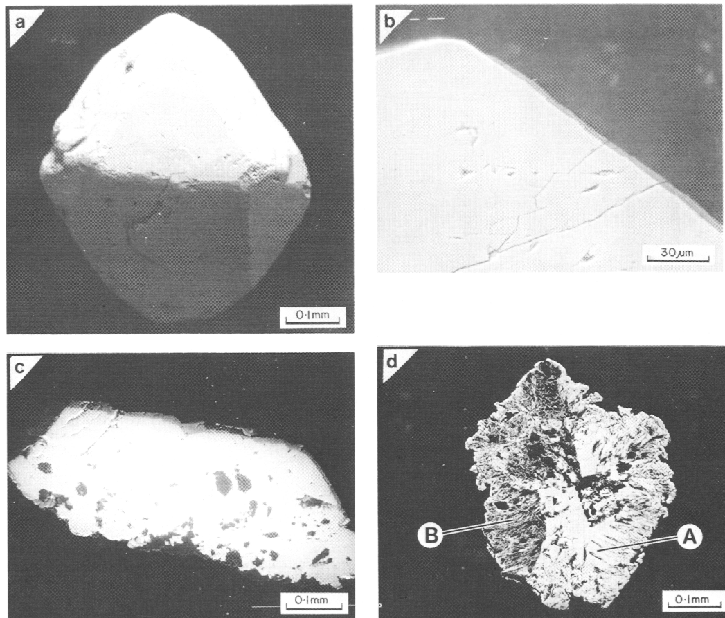
FIG. 1. SEM micrographs. (a) Euhedral crystal of arsenoflorencite-(Ce) from Locality 1. (b) Polished section of arsenoflorencite-(Ce) (light grey) with a thin coating of alunite (medium grey) from Locality 2. (c) Polished section of arsenoflorencite-(Ce) crystal (white) with abundant quartz inclusions (dark grey), and rimmed on the upper surface by florencite-(Ce) (light grey), from Locality 2. (d) Polished section of a complex grain consisting partly of arsenoflorencite-(Ce) (marked 'A') with linear inclusions of alunite (dark grey) and partly of an intimate intergrowth of alunite and the La analogue of arsenoflorencite-(Ce) (marked 'B'), from Locality 2.
