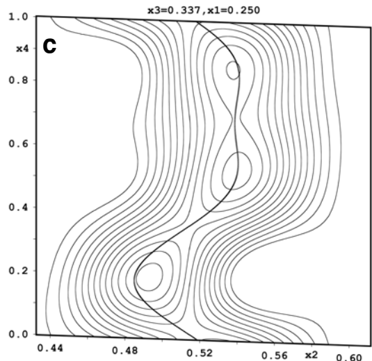
FIG. 7a–c. The y coordinate curves for “Pb” ( i.e. , M2 ) atom string in the crystal structures of gladiite, salzburgite and paarite, plotted on the background of Fourier maps of the internal space x_2 - x_4 .
