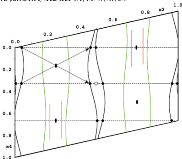
FIG. 4a. Action (x_1, -x_2 + \frac{1}{2}, x_3 + \frac{1}{2}, x_4 + \frac{1}{2}) of the c glide plane of the superspace group Pm\bar{c}n(0\beta 0)00s in the x_2 - x_4 section of gladiite (a three-fold superstructure) in which it “simulates” a symmetry centre at (\frac{1}{4}, \frac{1}{4}) , etc. Atom “strings” describe the modulation of atom positions in the x_2 - x_4 section of superspace (compare with Fig. 10a).
