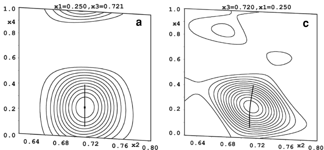
FIG. 10. The \Delta y coordinate curves for the string of Cu atoms in stoichiometric gladite, salzburgite and paarite, on the background of Fourier maps in the internal space x_2 - x_4 .
