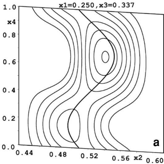
FIG. 7a–c. The y coordinate curves for “Pb” ( i.e. , M2 ) atom string in the crystal structures of gladiite, salzburgite and paarite, plotted on the background of Fourier maps of the internal space x_2 - x_4 .
