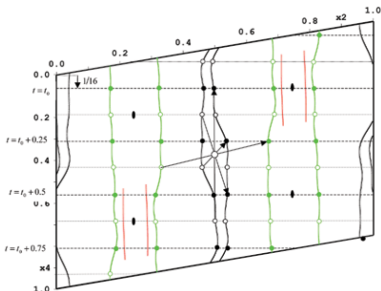
FIG. 4b. The centrosymmetric superspace group Pm\bar{c}n(0\beta 0)00s used for the description of the Pm\bar{c}2_1 structure of salzburgite (a four-fold superstructure). Note a shift of t_0 by 1/16 , the real t_0 + n/4 levels (dashed) and imaginary t_0 + n/8 levels (stippled), as well as the real (black) and imaginary (void) atoms on selected strings.
