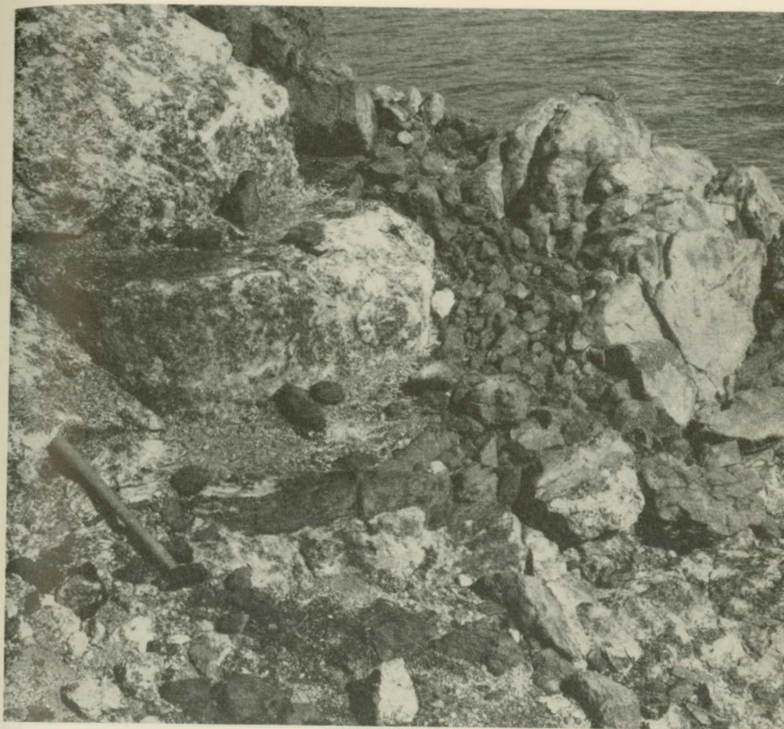
Fig. 21. Lujavrite wedging out in naujaite (H.5–6 plate 1). Towards the left, this vein is continued as a brown acmitic vein containing steenstrupine. The brown vein is not seen in the photograph.
