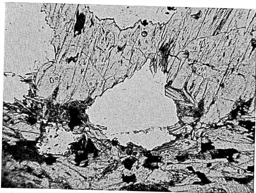
Fig. 31. 21017b. \times 30 , 1 nic. A large naujaite ægirine anhedral (upper part of the photograph) is substituted by ægirine felt along the contact with an acmite vein (lower part of the photograph). Small needles of ægirine can be seen in the latter zone. The white inclusions in the naujaite ægirine are of sodalite. The dark grains in the acmite zone are arfvedsonite and eudialyte pseudomorphs. The white area in this zone is a small microcline lath surrounded by analcime. (Igdlunguaq).
