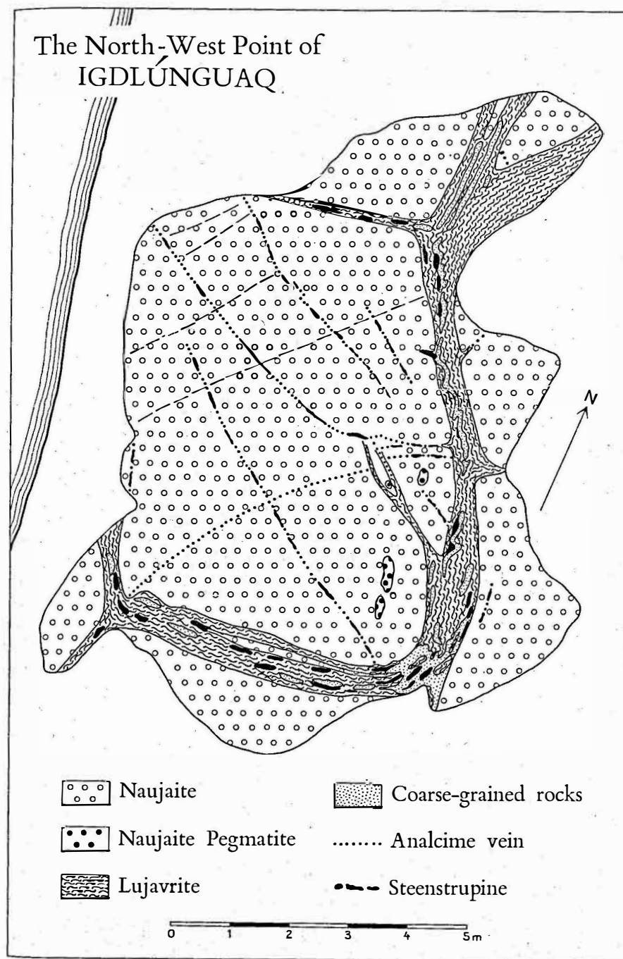
Fig. 23. Map of the small area on the west coast of Igdlúnguaq (cf. fig. 9). The analcime vein symbol also includes natrolite-bearing veins; the symbol indicating the coarse-grained rocks comprises the recrystallized inclusions of naujaite in lujavrite and the "dense" analcime rock. The white areas are covered by scree.
