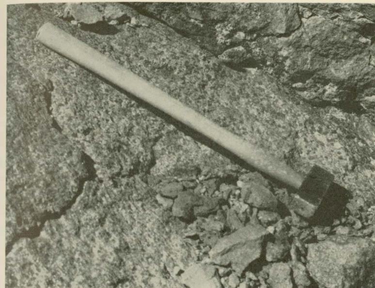
Fig. 30. Concentration of steenstrupine in lujavrite (see text p. 65).
