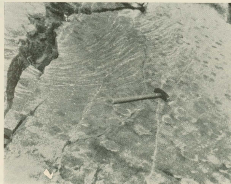
Fig. 12. White stringers and spheroids in the lujavrite to the north of the map area indicated by plate 1. These stringers are contiguous with the adjacent naujaite bands (see SØRENSEN, 1958, fig. 10).
