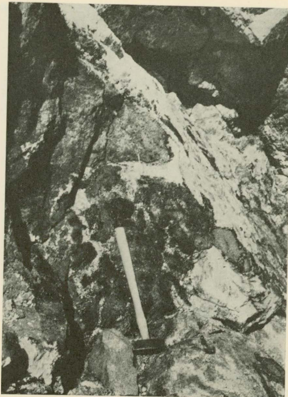
Fig. 15. Detail of fig. 14 showing veins of analcime branching out into the very dark lujavrite. These veins are too small to be indicated on the map of plate 1.
