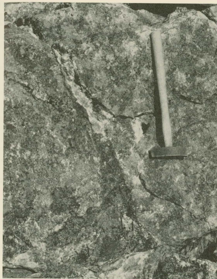
Fig. 22. Analcime-natrolite vein in naujaite (H. 2-3 plate 1). There are concentrations of steenstrupine along the borders of the vein (see the text p. 50).
