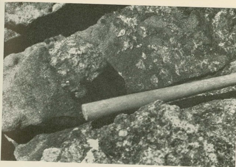
Fig. 19. Inclusions of felt-like ægirine in lujavrite (F.3 plate 1). The lujavrite is darkest around the inclusions. Naujaite occurs in the foreground.
