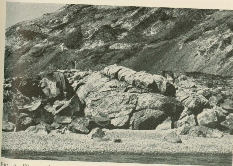
Fig. 8. The southwest point of Igdlunguaq as seen from the east. The distinct slightly inclined fracture in the centre of the photo is a brown vein in a naujaite lens (cf. plate 1). In the mountain wall behind Igdlunguaq naujaite inclusions in lujavrite can be seen.
