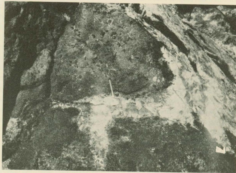
Fig. 16. Detail of fig. 15. Analcime vein with a concentration of steenstrupine and eudialyte pseudomorphs along the borders. The lujavrite is rich in poikilitic grains of steenstrupine (black).
