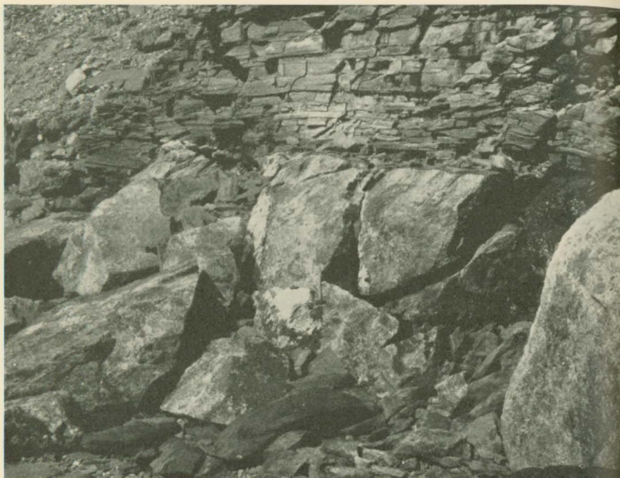
Fig. 28. Naujaite cut by two albititic veins and enclosed in schistose lujavrite (Tugtup agtakórfia).
