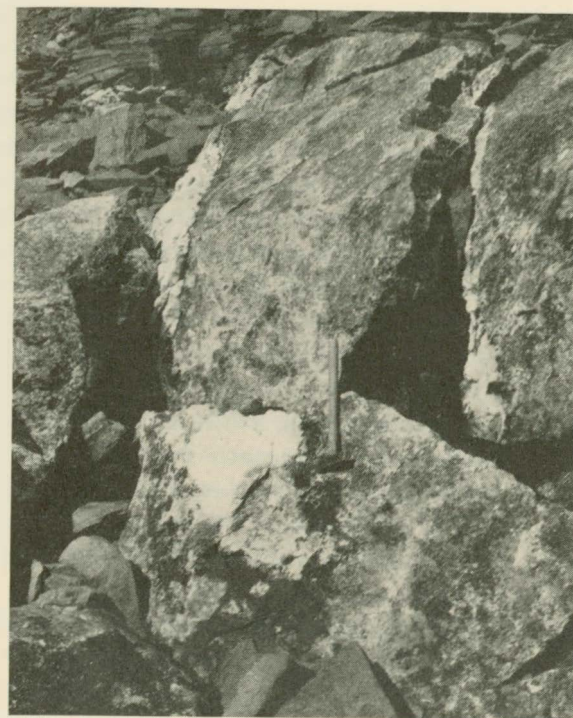
Fig. 29. Close up of the albititic veins seen in fig. 28. Note the dark borders of the vein on the left and its horizontal continuation in the upper border between naujaite and lujavrite (top left).
