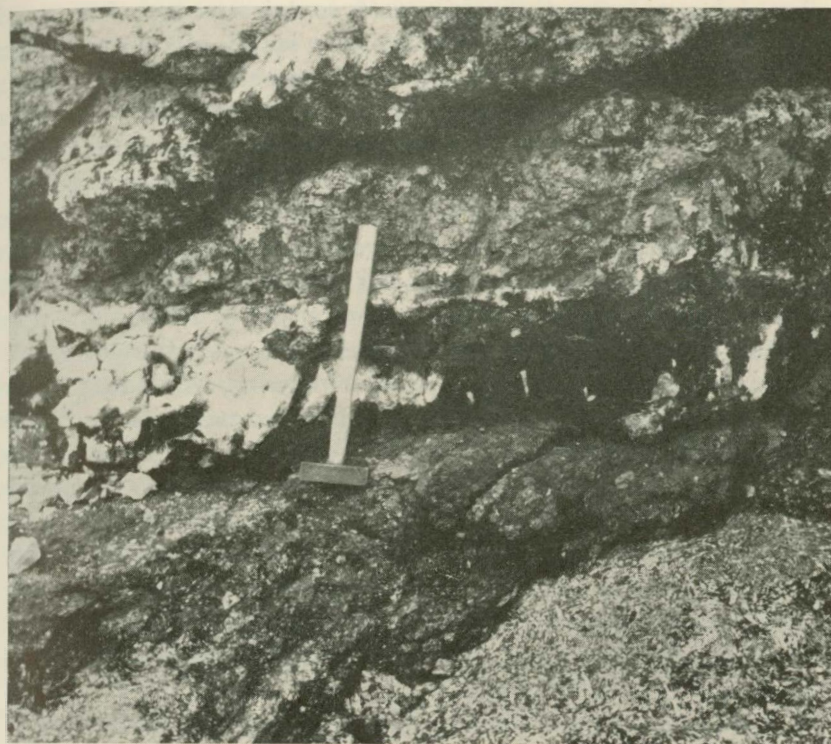
Fig. 6. Detail of fig. 5. The coarse-grained microcline rock occurs to the left of the hammer, the coarse-grained ægirine with rinkite to the right. The eudialyte zone is the dark rock below the head of the hammer. Bottom left: a gradual transition from the eudialyte zone into the underlying naujaite; top right: ægirine felt and the radioactive rock.
