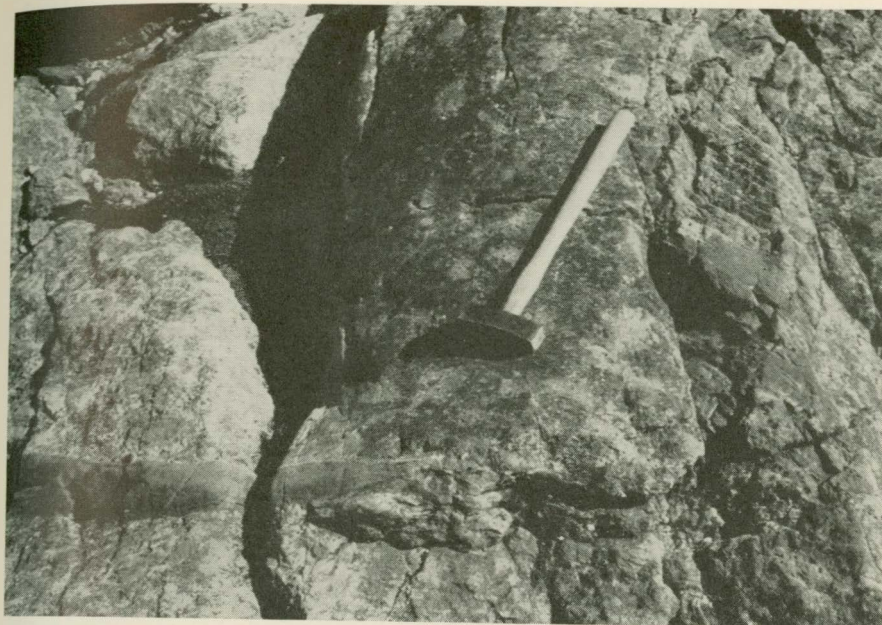
Fig. 17. In the bottom left part of the photograph a small lujavrite vein is seen (G. 2, plate 1). Just below the head of the hammer this vein is connected with the east-west zone of "dense" analcime rock. The internal folding of that rock may be faintly seen to the right of the hammer handle.
