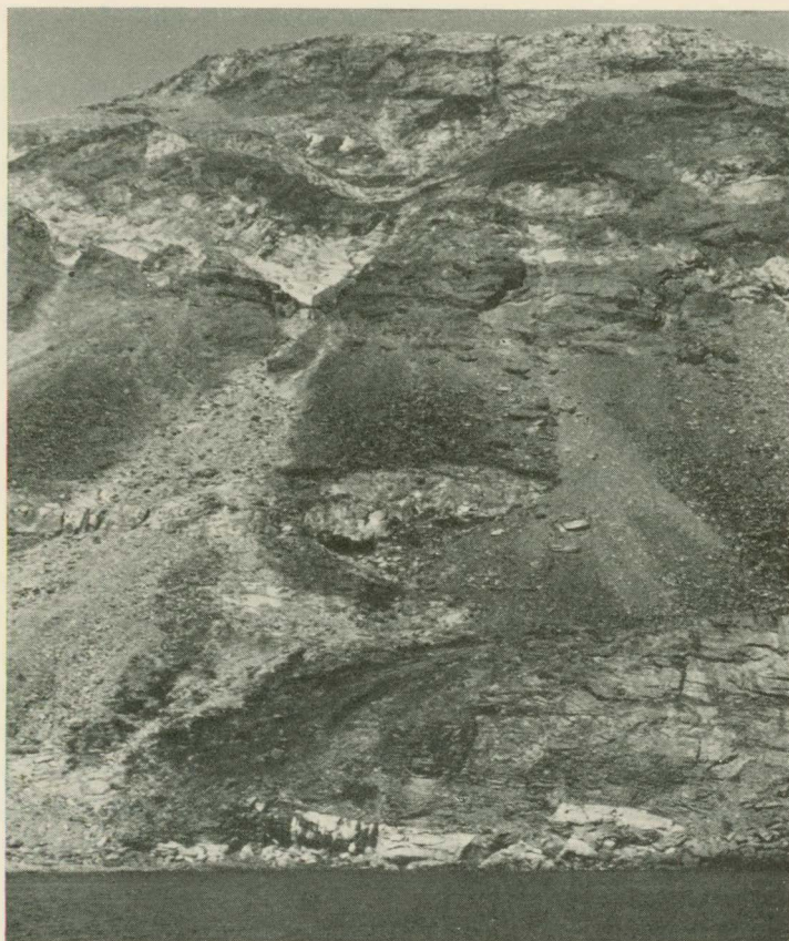
Fig. 26. View of Tugtup agtakôrfia from the fiord. The inclusion of naujaite studied in this paper is seen on the shore in the left part of the photograph. Note the horizons of naujaite inclusions in lujavrite in the mountain wall.
