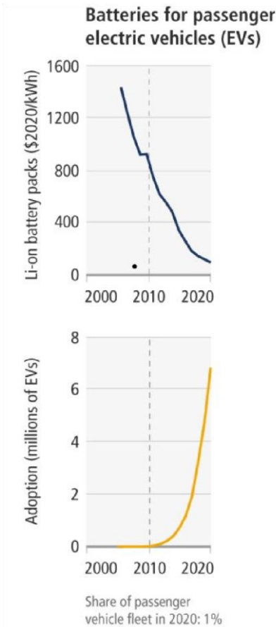
Figure 8.5 Adoption of EVs worldwide and the development of the Li-ion battery unit price
