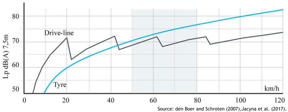
Figure 10.8 Correlation between velocity and noise emitted by car
