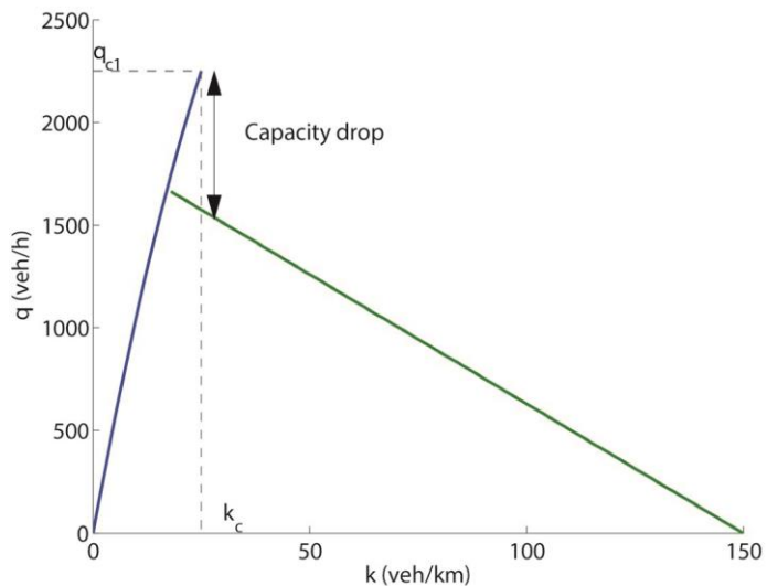
Figure 7.8 The capacity drop in the flow-density diagram
