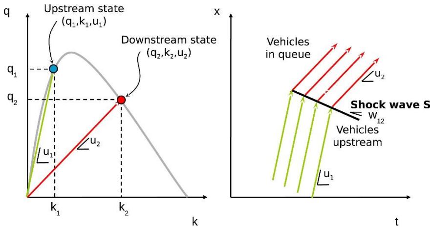
Figure 7.12 Graphical interpretation of shockwave speed
