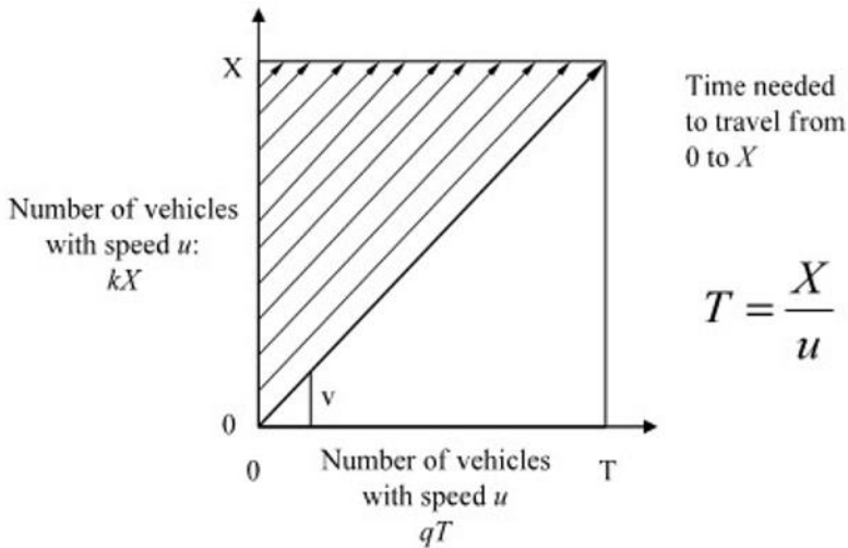
Figure 7.2 Vehicle trajectories and key microscopic flow characteristics
