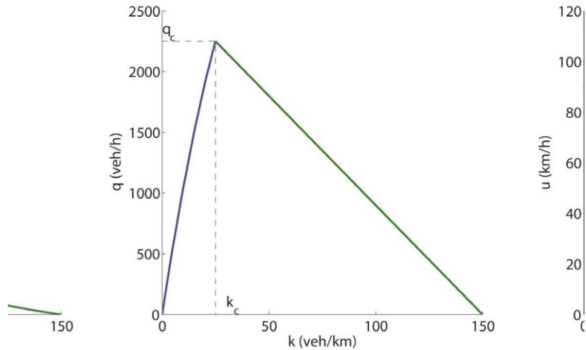
Figure 7.7 Example of fundamental diagram
