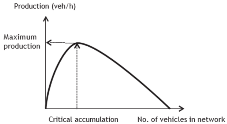
Figure 7.13 Example Network Fundamental Diagram
