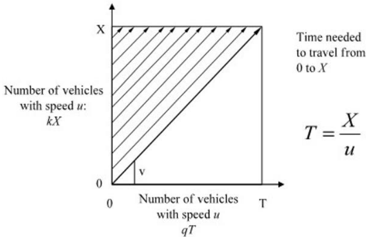
Figure 7.3 Derivation of the continuity equation
