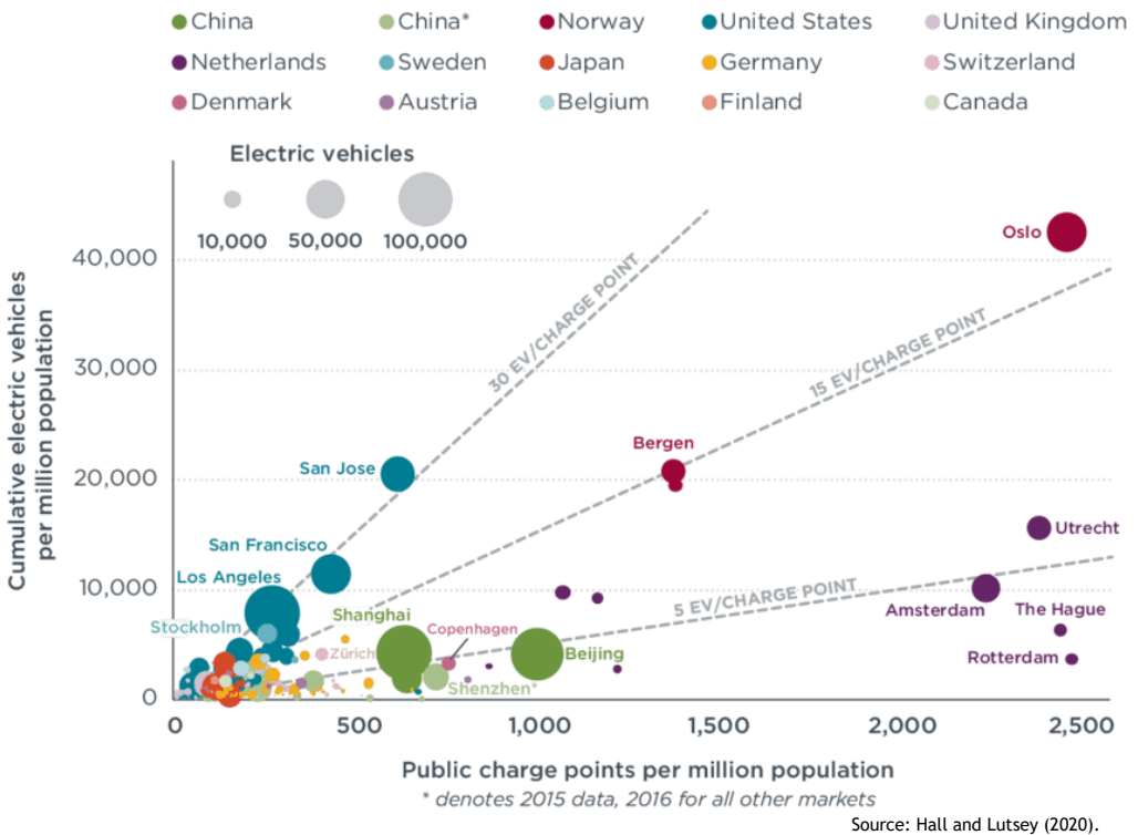
Figure 10.9 Public charging infrastructure and electric vehicle registration per million
