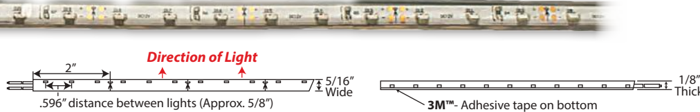
IP65 Edge of Light Provides Protection From Dust & Splashing Water, Not Submersible
