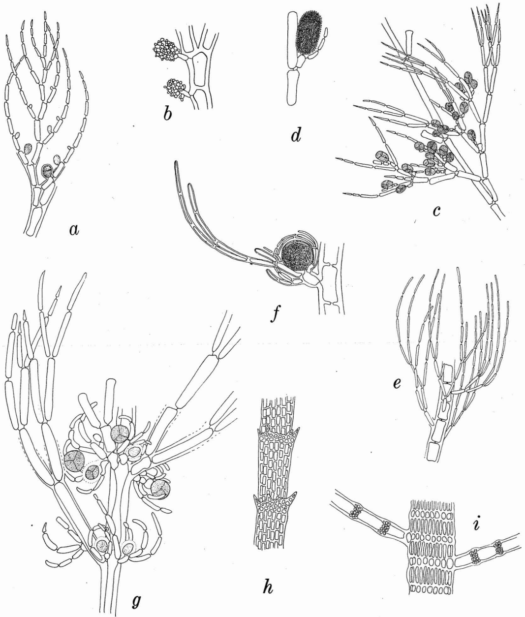
FIG. 54. a, b, Mesothamnion caribaeum : a , Upper portion of a tetrasporangial branch, \times 75 ; b , a small part of a male branch bearing two pedicellate antheridial clusters, \times 226 . c, d, Antithamnion sp.: c , Part of an erect, alternately branched secondary axis bearing tetrasporangia, \times 75 ; d , an antheridial branchlet, \times 171 . e, f, Callithamnion sp.: e , Upper portion of a percurrent axis with spirally arranged branchlets, \times 55 ; f , a sporangial structure, \times 93 . g, Wrangelia argus : A small part of a fertile axis showing the lateral branchlets and tetrasporangia, \times 96 . h, Centroceras clavulatum : A small part of a filament showing the arrangement of the cortical cells and the ring of spines at the nodes, \times 150 . i, Spyridia filamentosa : A small part of a main axis showing the cortication and the base of two determinate branchlets, \times 80 .
