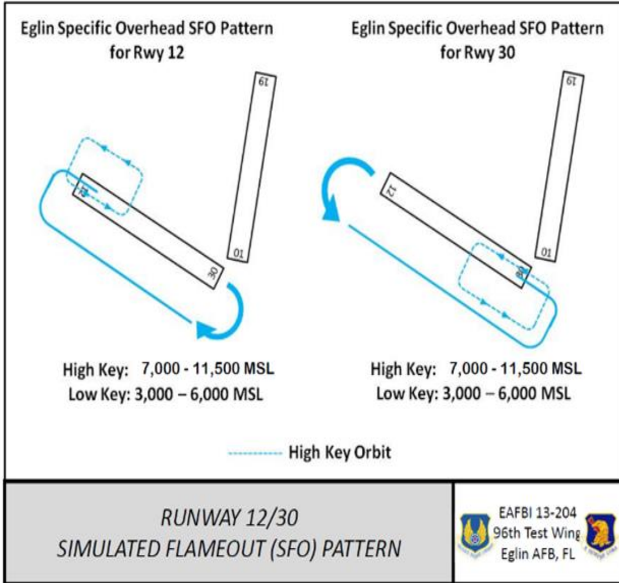
Figure A9.1. Runway 12/30 Simulated Flameout (SFO) Pattern.
