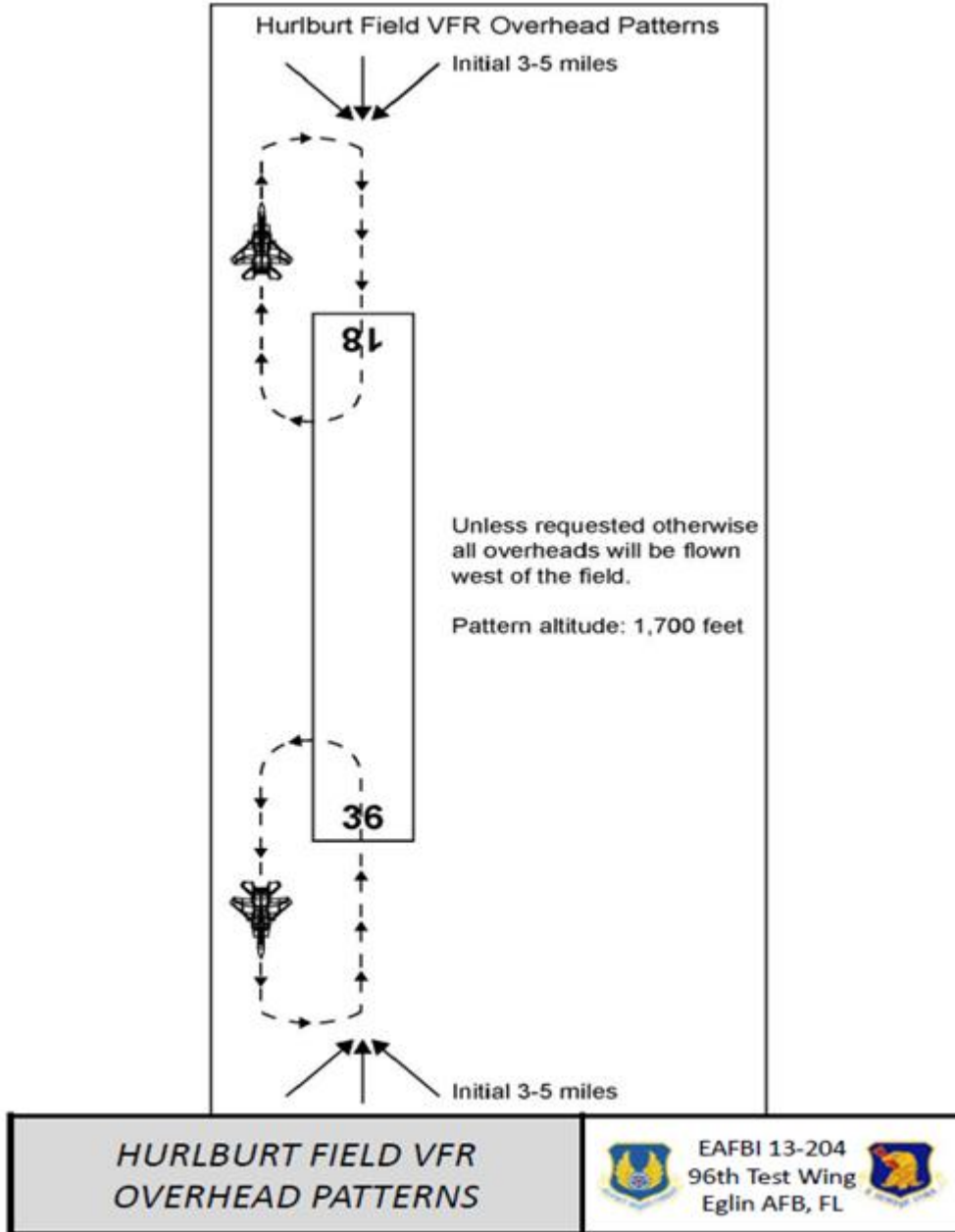
Figure A34.1. Hurlburt Field VFR Overhead Pattern.
