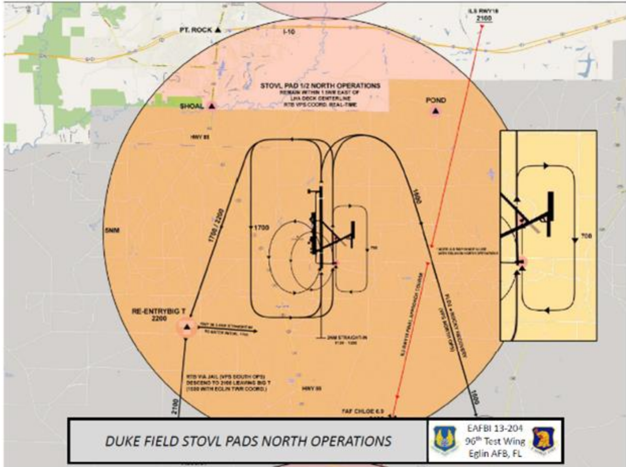
Figure A25.1. Duke Field STOVL Pads North Operations.
