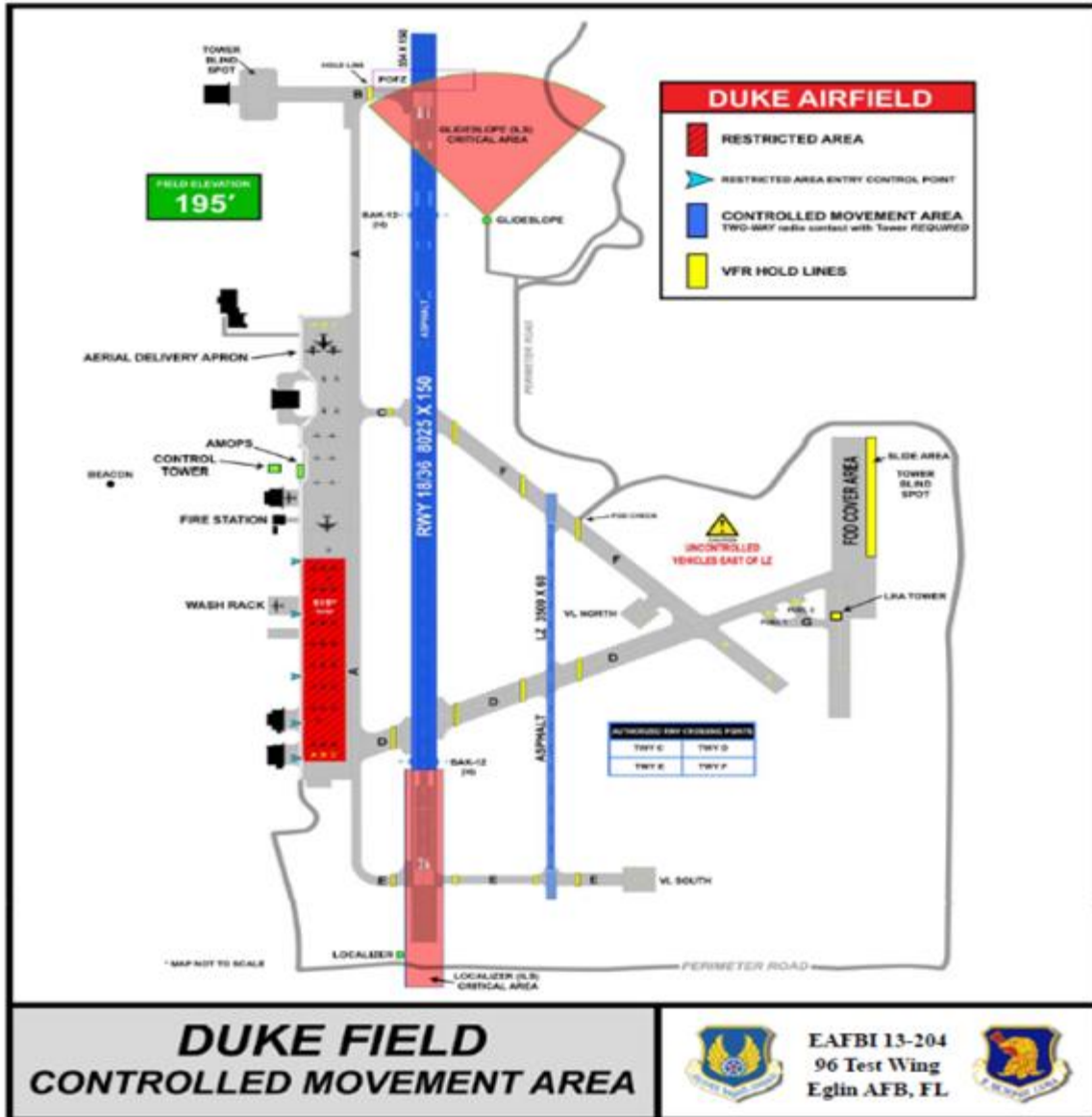
Figure A21.1. Duke Field Controlled Movement Area Diagram.
