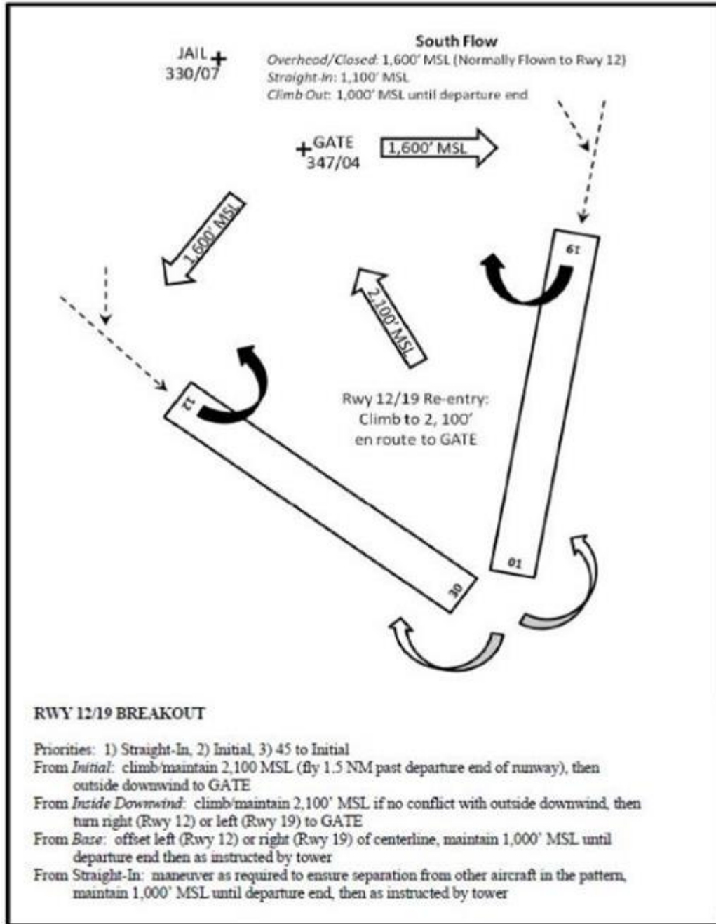
Figure A7.1. Eglin VFR Traffic Patterns Runways 12/19 Active.
