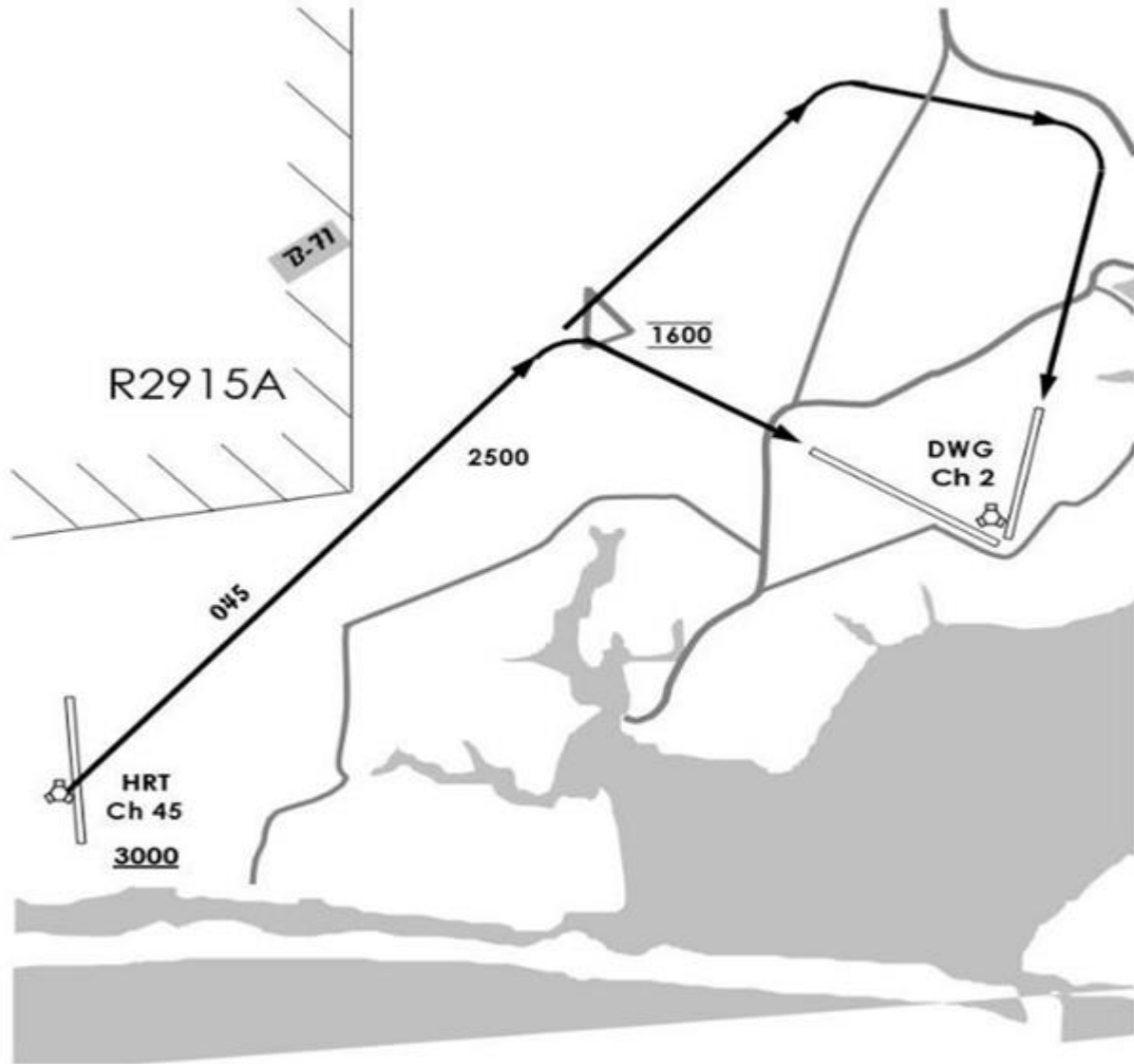
Figure A18.1. Whiskey Hotel Recovery.
