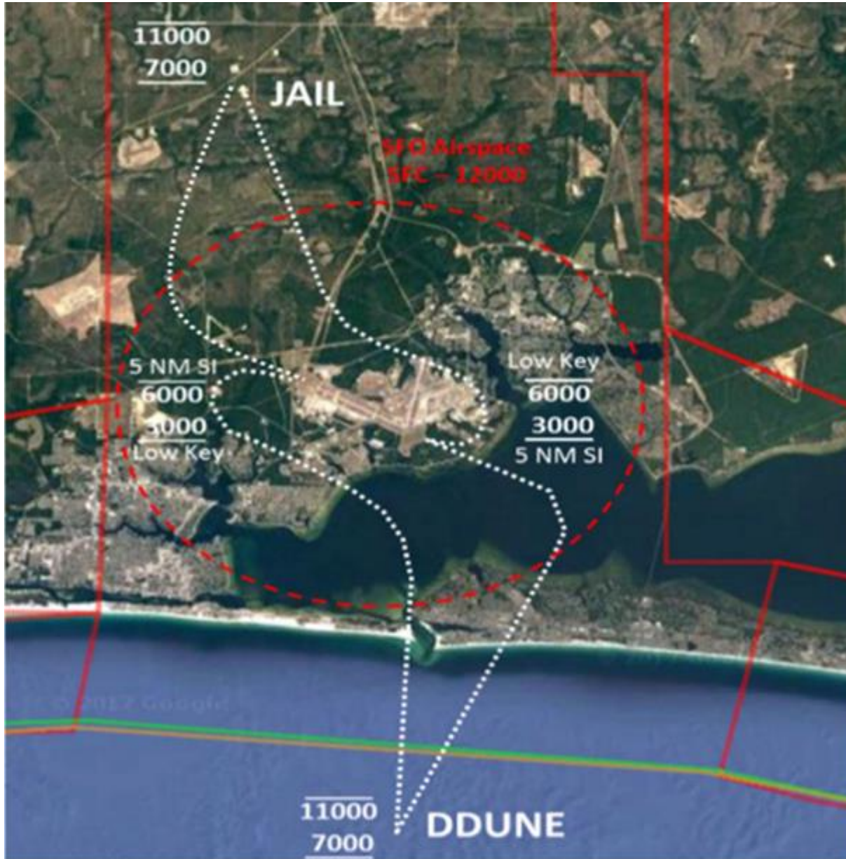
Figure A11.1. Rwy 12/30 Random Entry Simulated Flameout Pattern (RESFO) Procedures.
