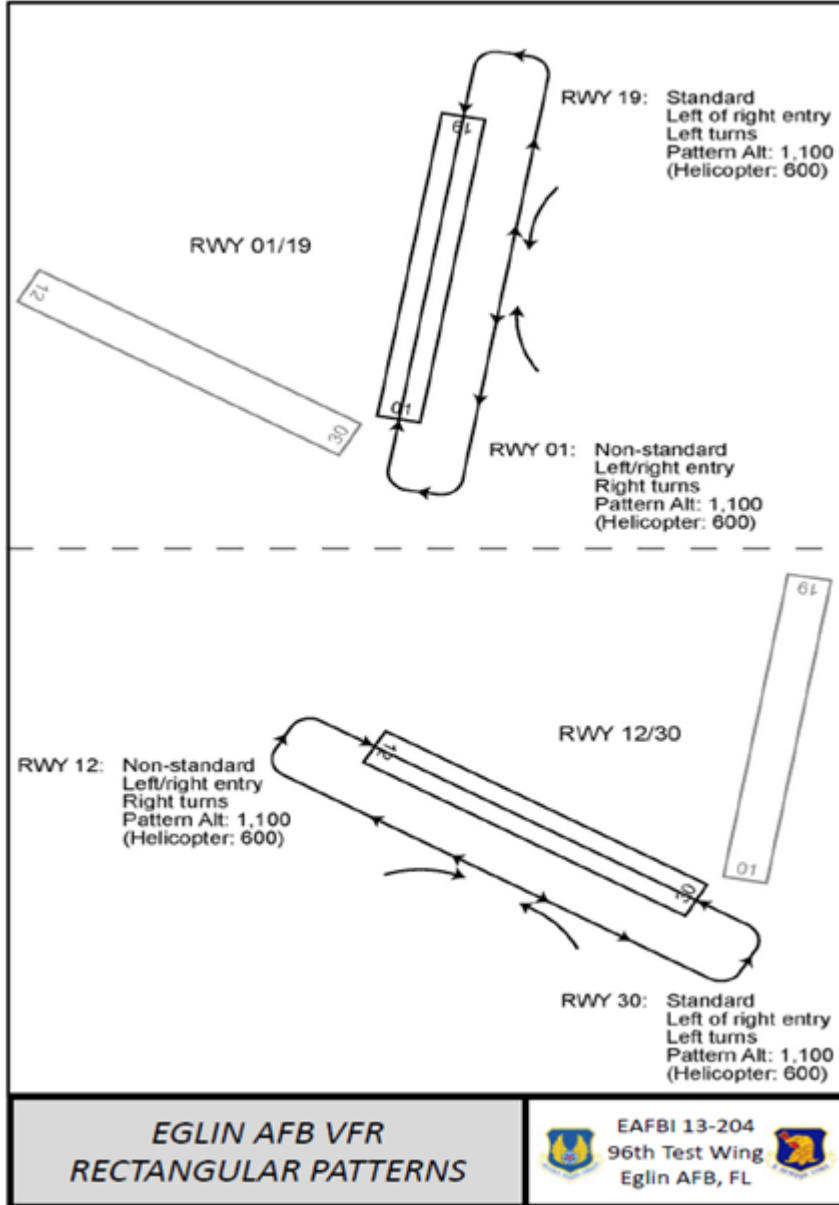
Figure A6.1. Eglin AFB VFR Rectangular Patterns.
