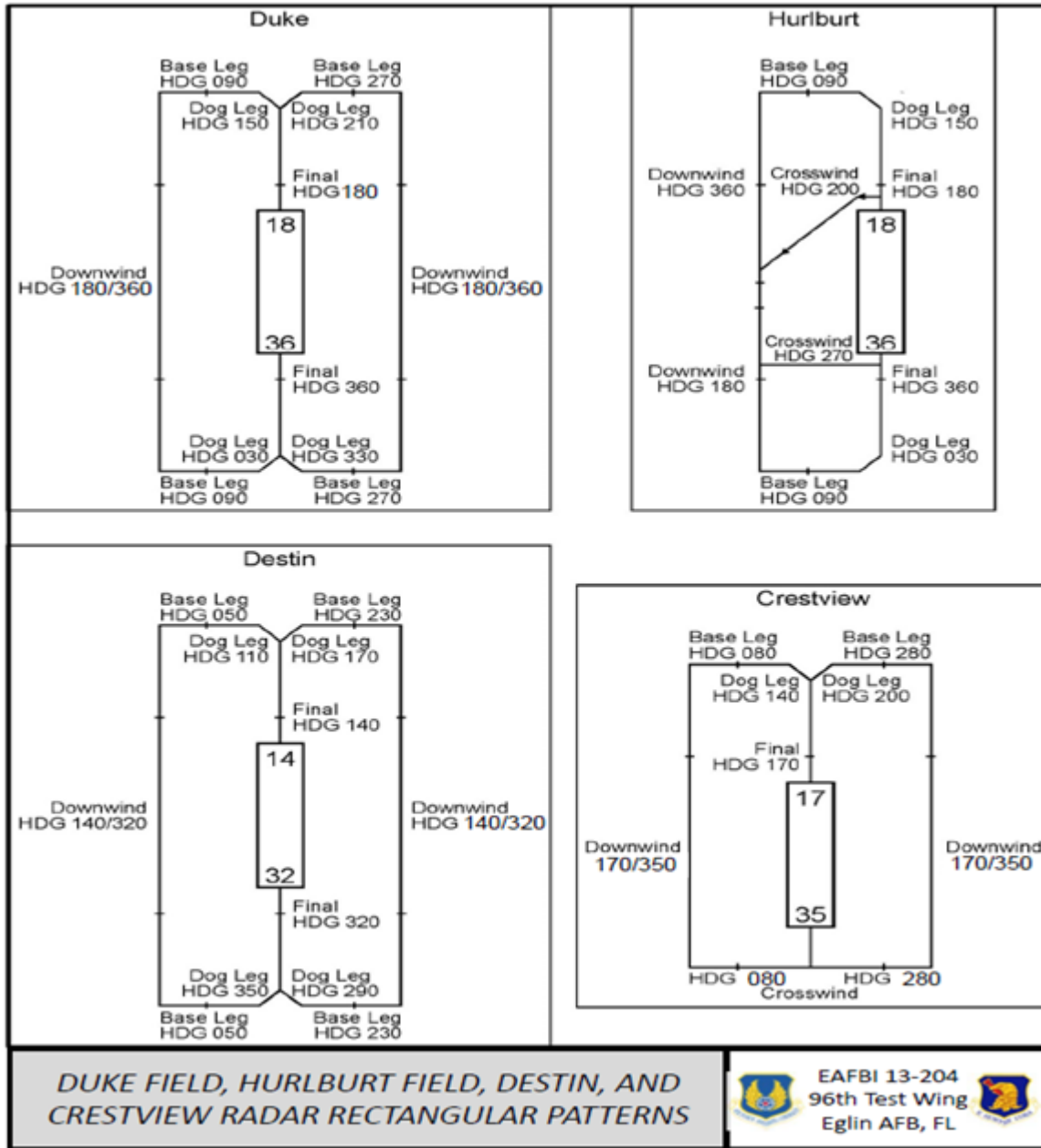
Figure A32.1. Duke Field, Hurlburt Field, Destin, and Crestview Radar Rectangular Patterns.
