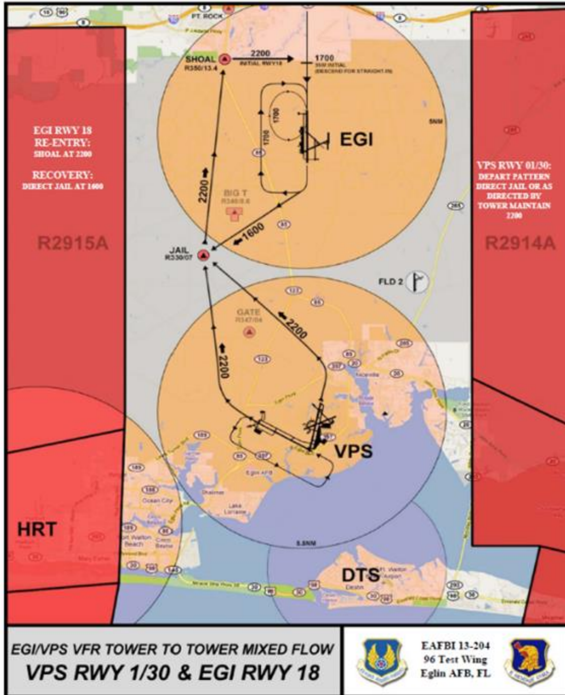
Figure A14.1. VFR Tower to Tower Procedures – Mixed Flow VPS RWY 1/30 & EGI RWY 18.
