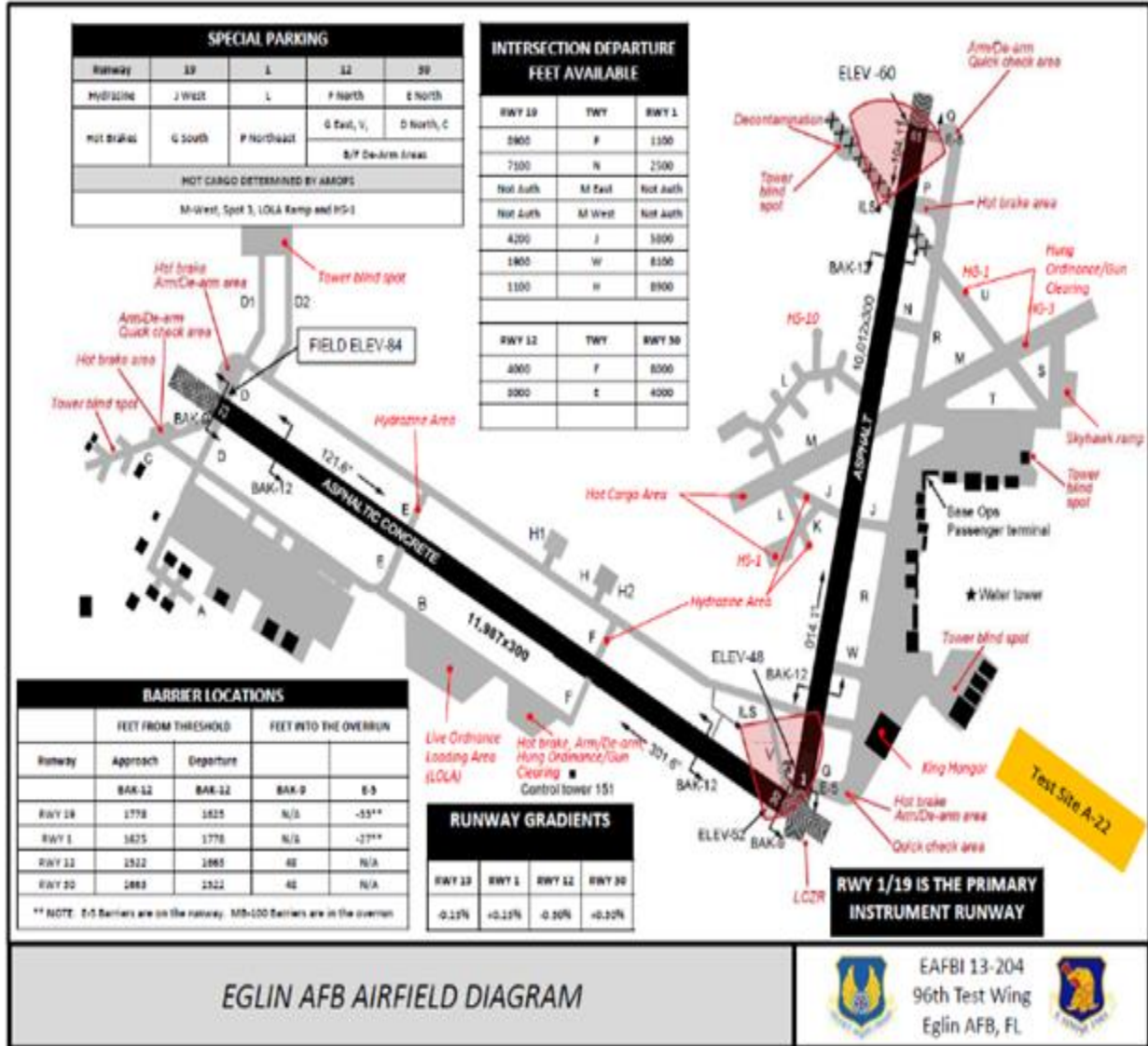
Figure A2.1. Eglin AFB Airfield Diagram.
