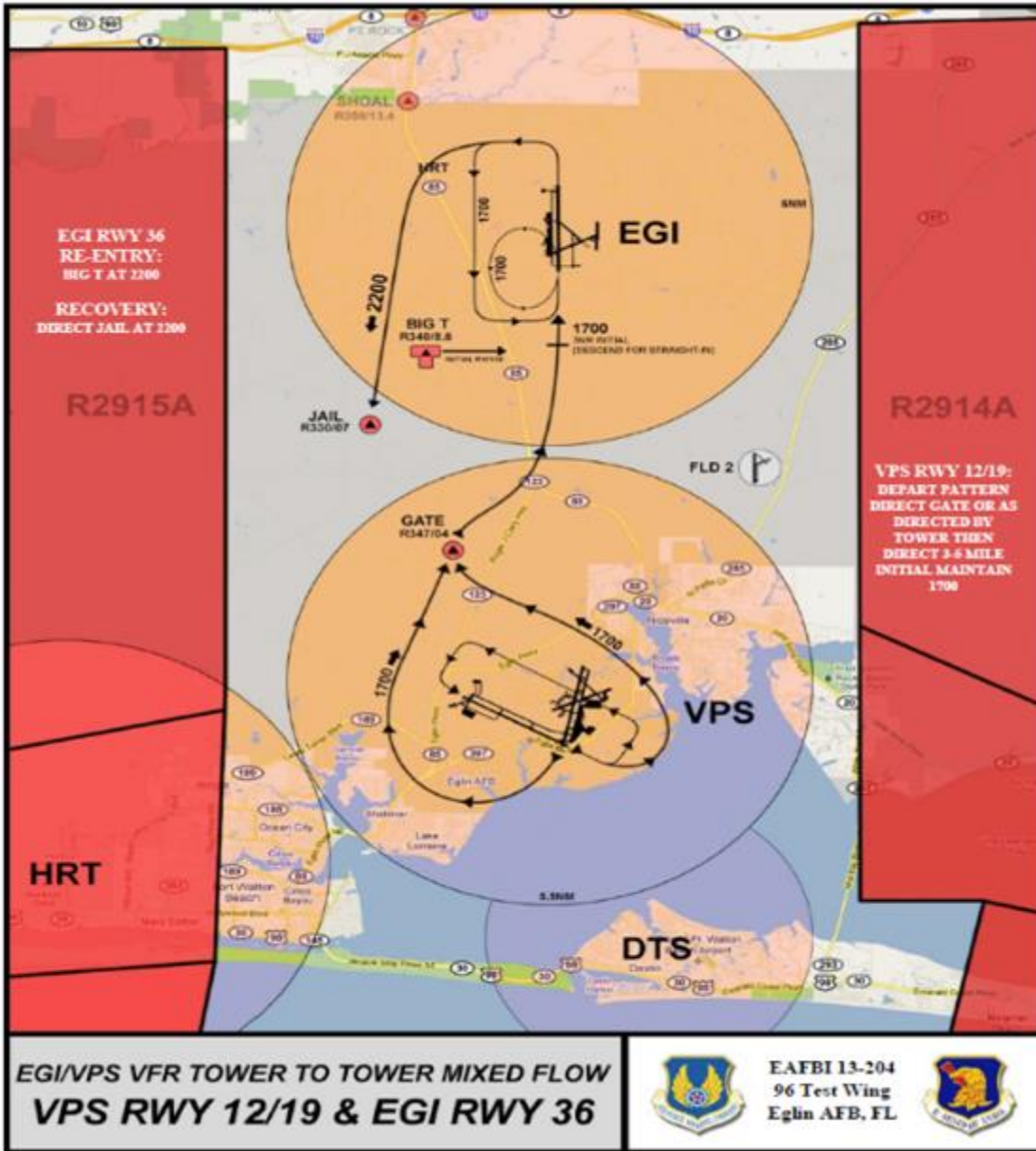
Figure A15.1. VFR Tower to Tower Procedures – Mixed Flow VPS RWY 12/19 & EGI RWY 36.
