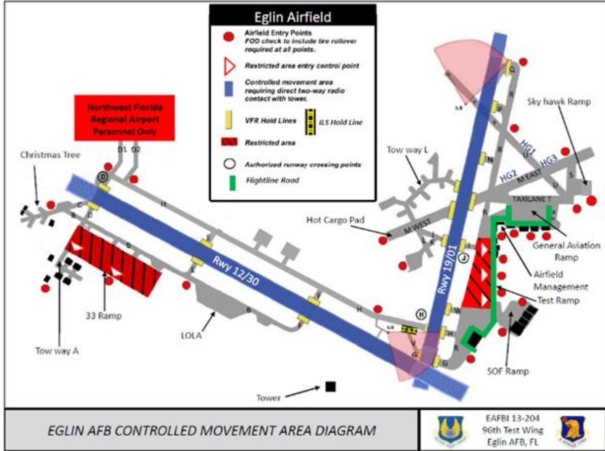
Figure A3.1. Eglin AFB Controlled Movement Area Diagram.
