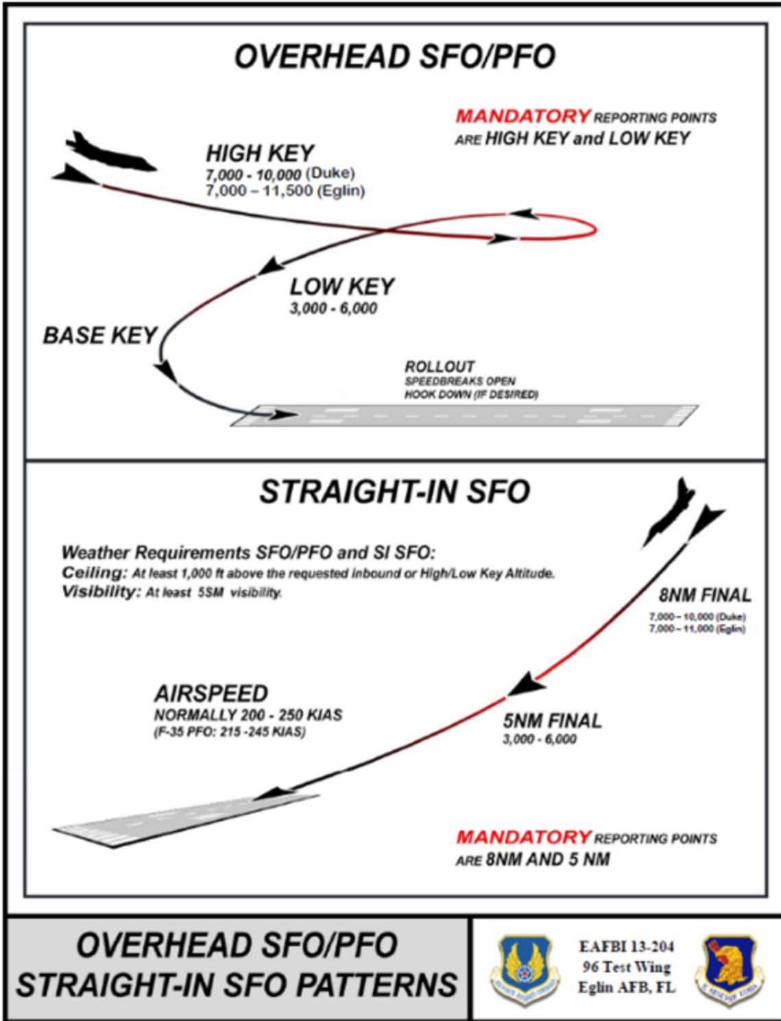
Figure A10.1. Overhead SFO/PFO and Straight-In SFO Patterns.
