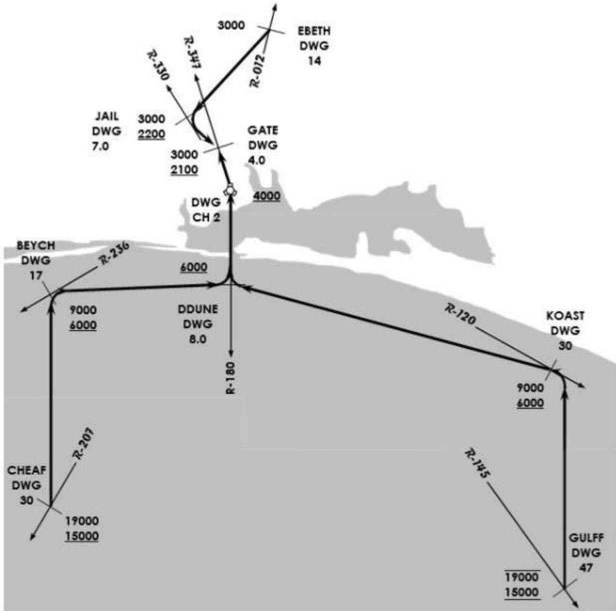
Figure A17.1. DDUNE Recovery.
