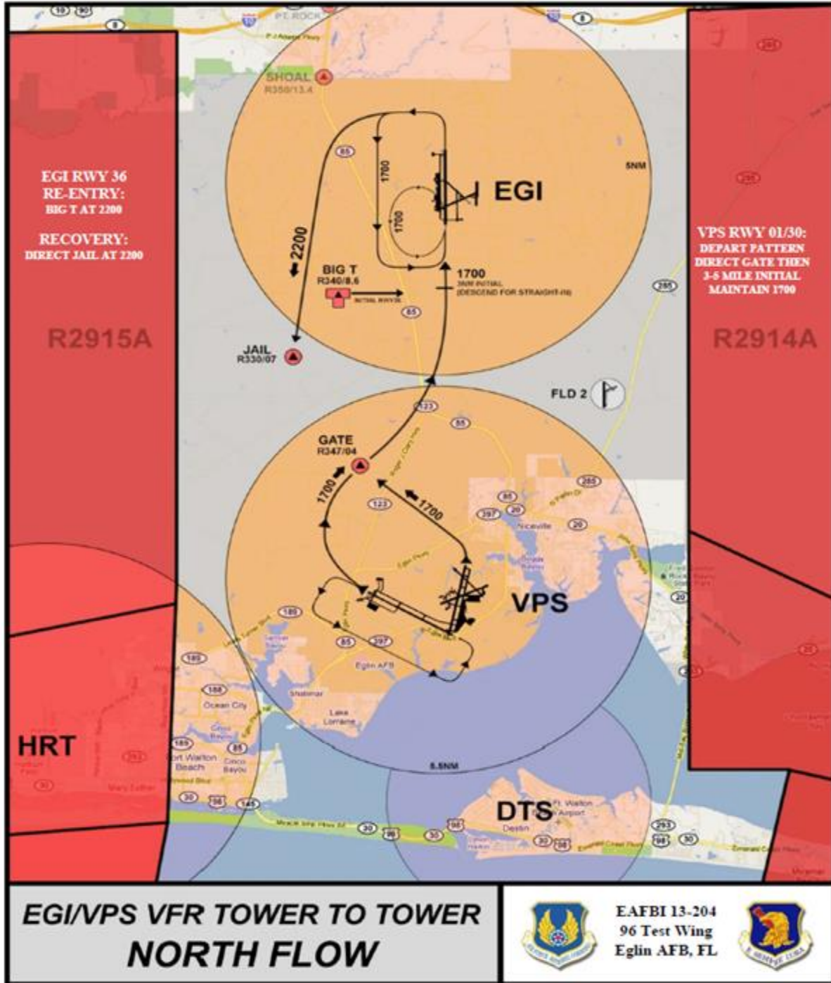
Figure A13.1. VFR Tower to Tower Procedures – North Flow.
