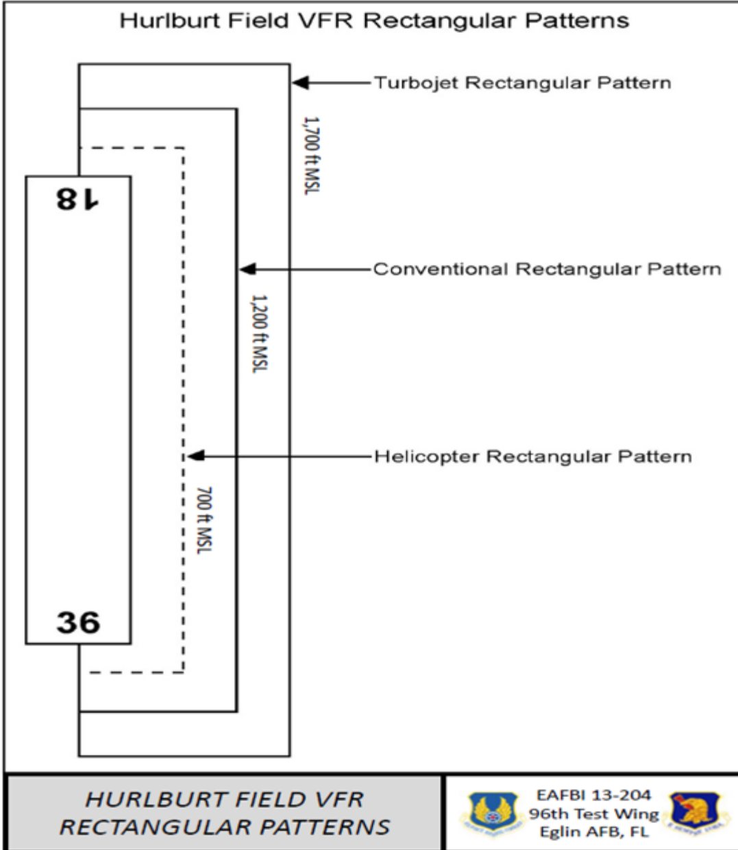
Figure A33.1. Hurlburt Field VFR Rectangular Patterns.
