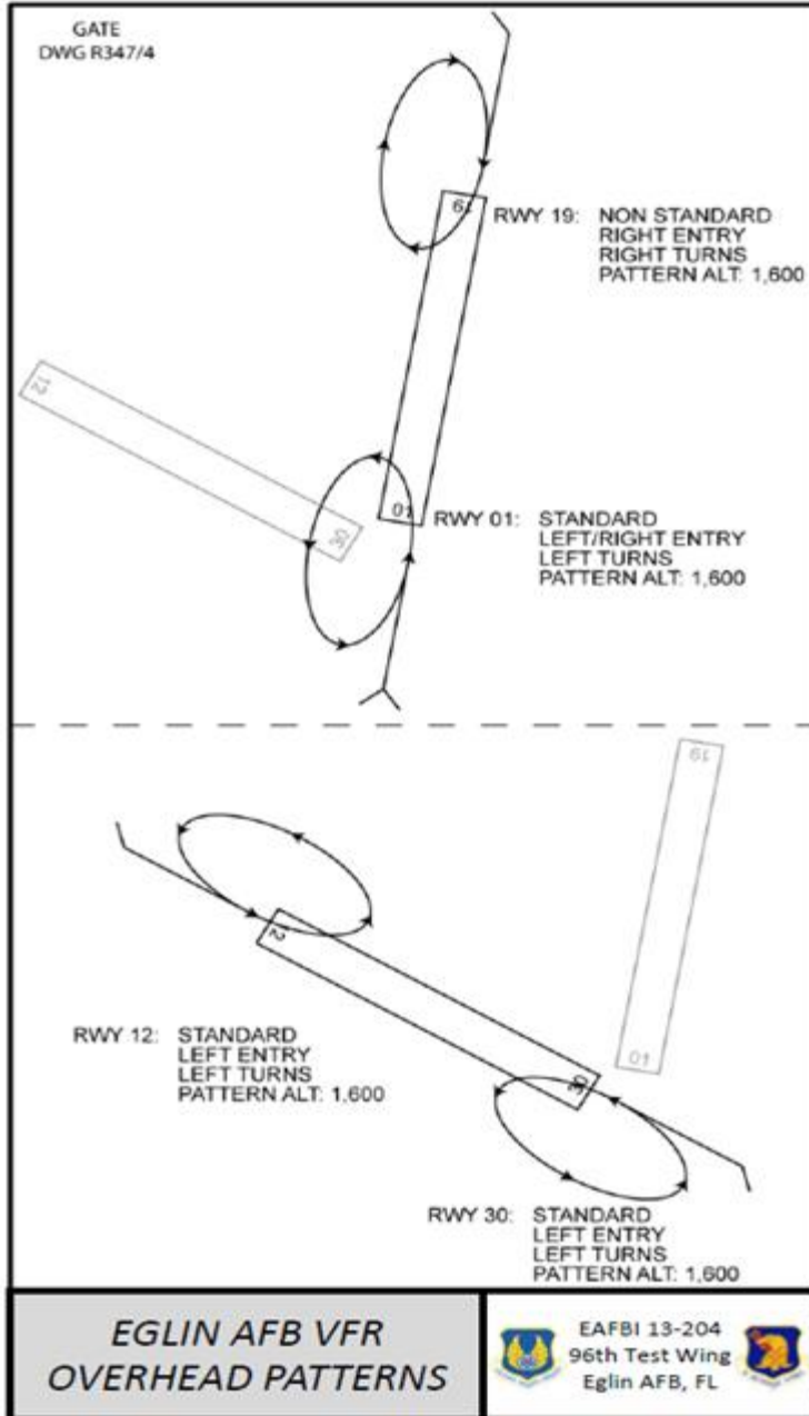
Figure A5.1. Eglin AFB VFR Overhead Patterns.
