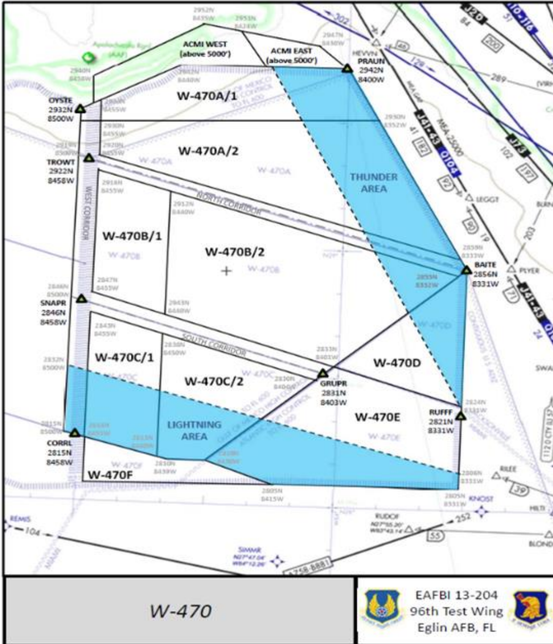
Figure A41.1. W-470.
