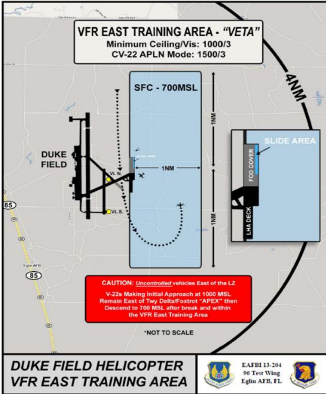
Figure A31.1. Duke Field Helicopter VFR East Training Area.
