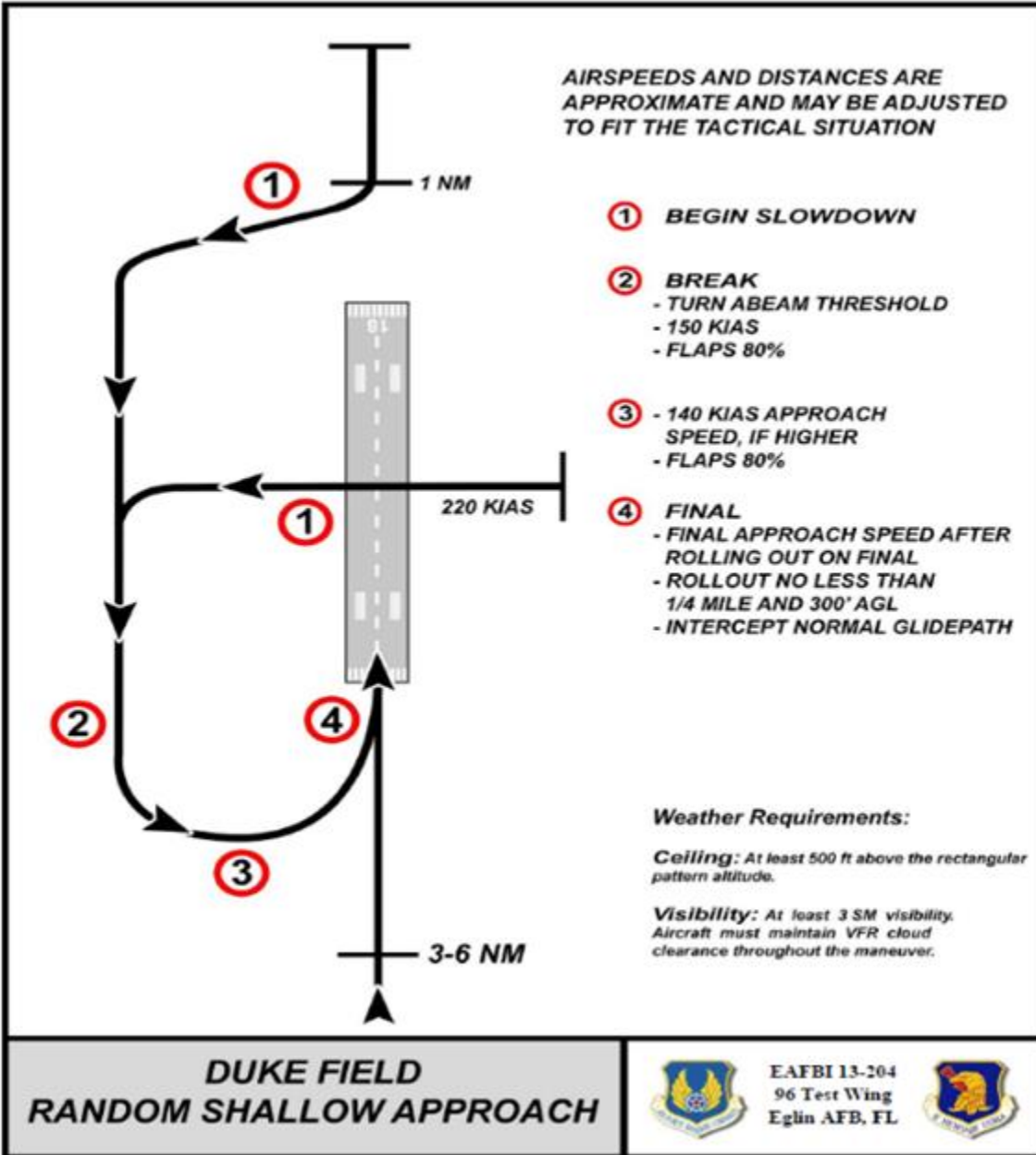
Figure A28.1. Duke Field Random Shallow Approach.
