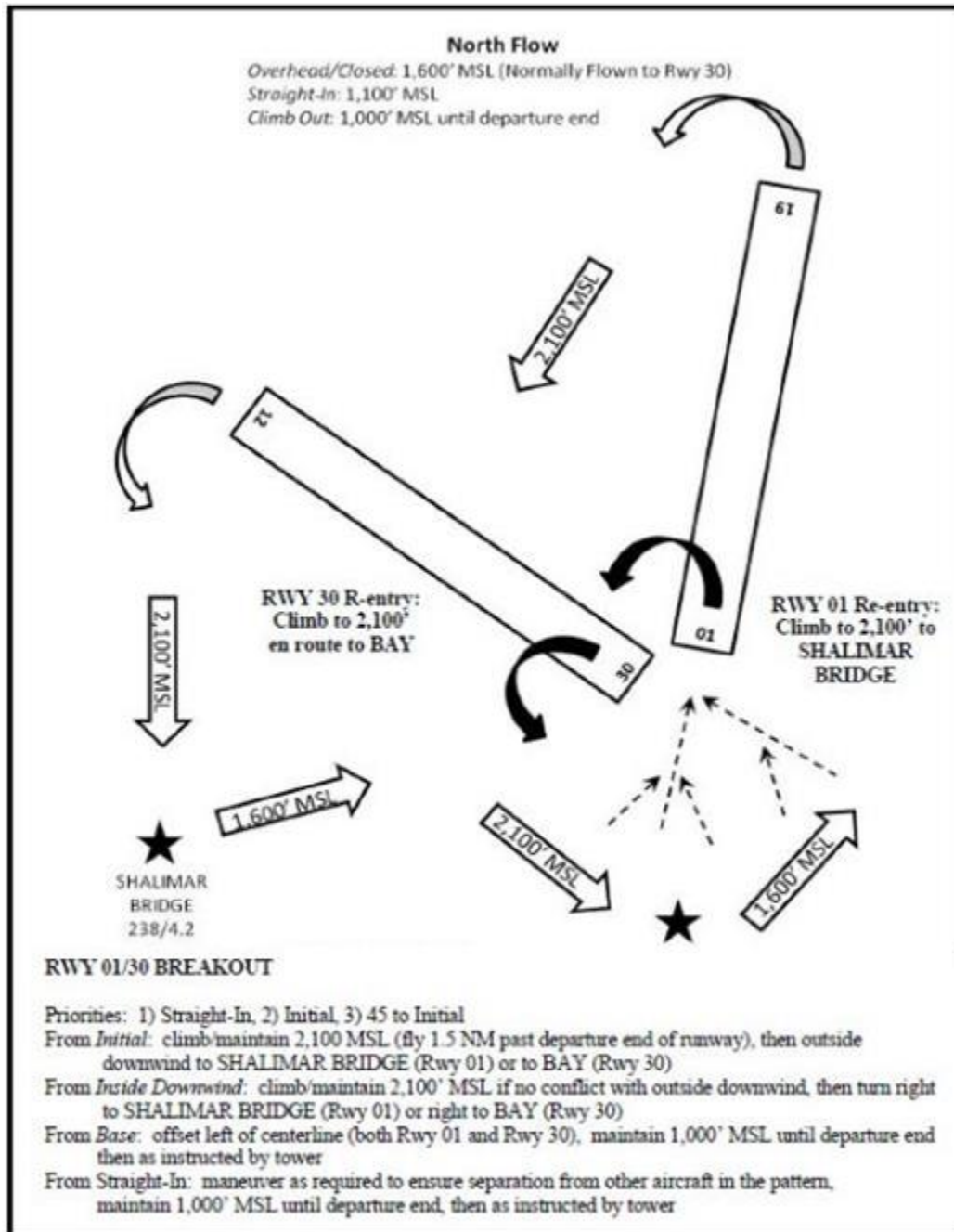
Figure A8.1. Eglin Traffic Patterns Runways 1/30 Active.
