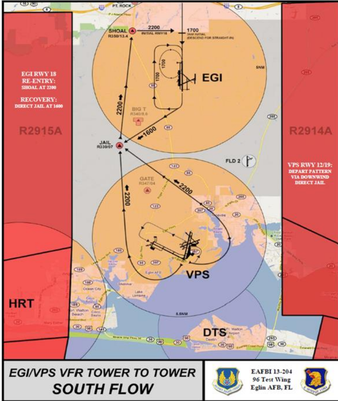
Figure A12.1. VFR Tower to Tower Procedures – South Flow.
