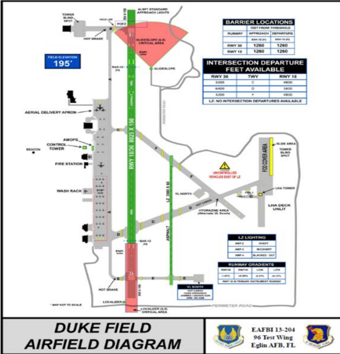
Figure A20.1. Duke Field Airfield Diagram.
