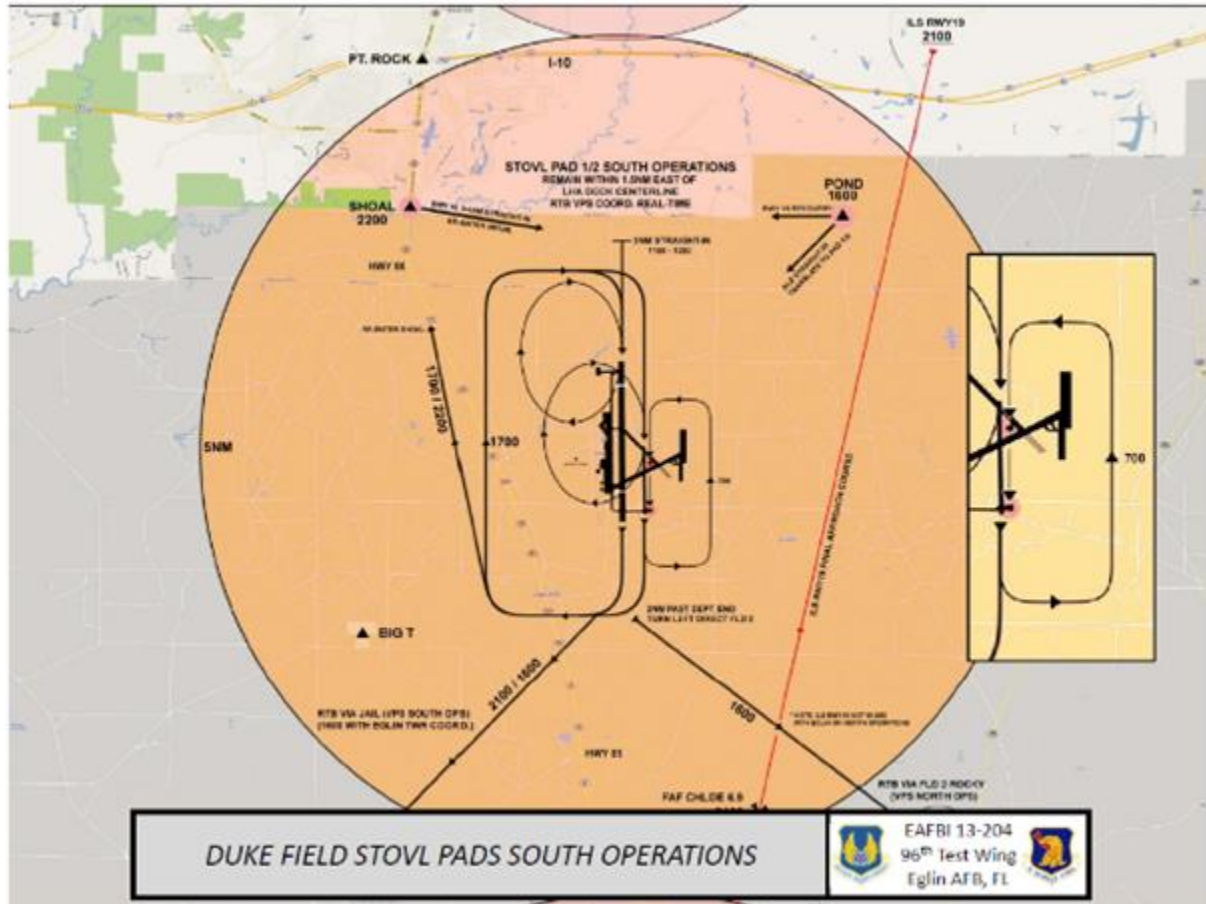
Figure A24.1. Duke Field STOVL Pads South Operations.
