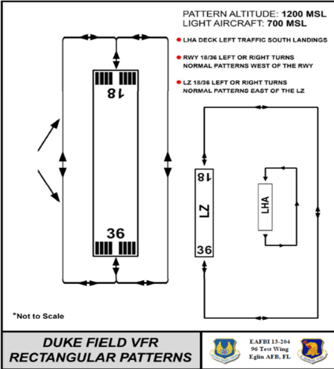
Figure A26.1. Duke Field VFR Rectangular Patterns.
