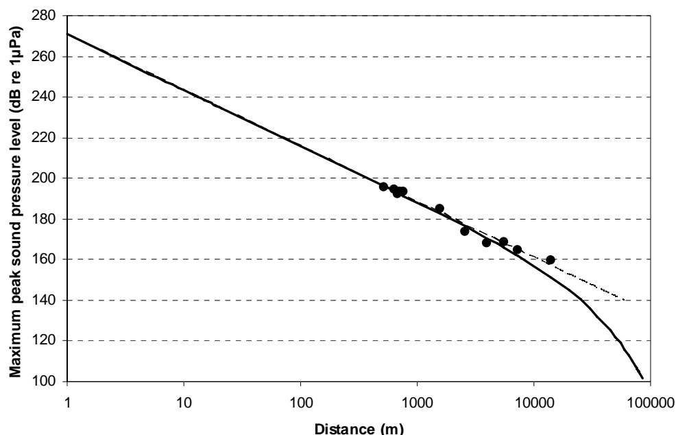
Figure 5. Relationship between maximum peak SPL (dB re 1 μPa) and distance (m) from the source of the underwater noise during the piling of monopile B10. The dashed line represents the fitted linear model of the measured values (closed circles). The solid line represents the maximum peak SPL as a function of distance, taking into account both attenuation and absorption.
