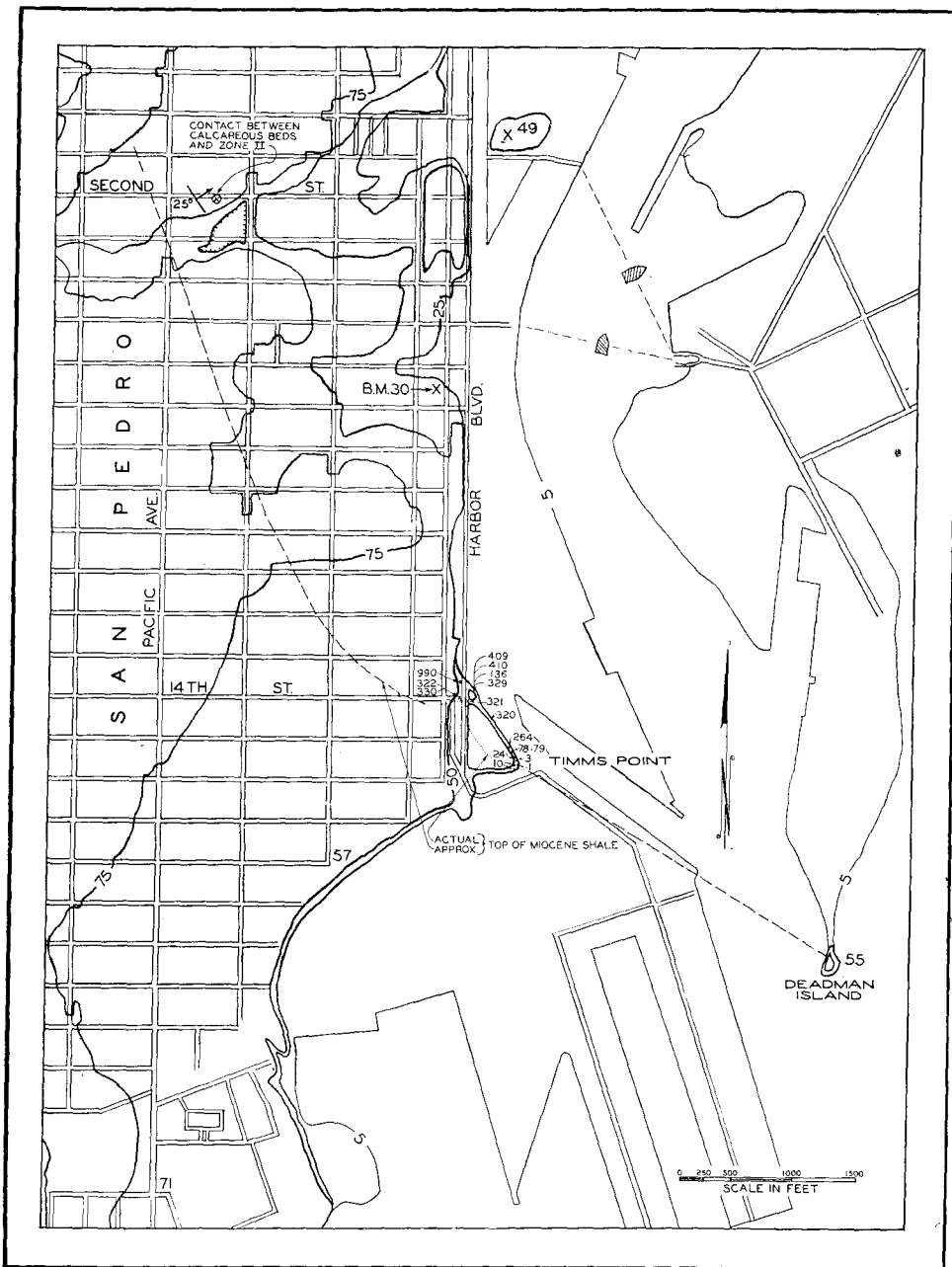
Sketch map of the town of San Pedro, California, indicating collecting localities at Timms Point. (Adapted from U. S. Geol. Survey, Wilmington Quadrangle)
