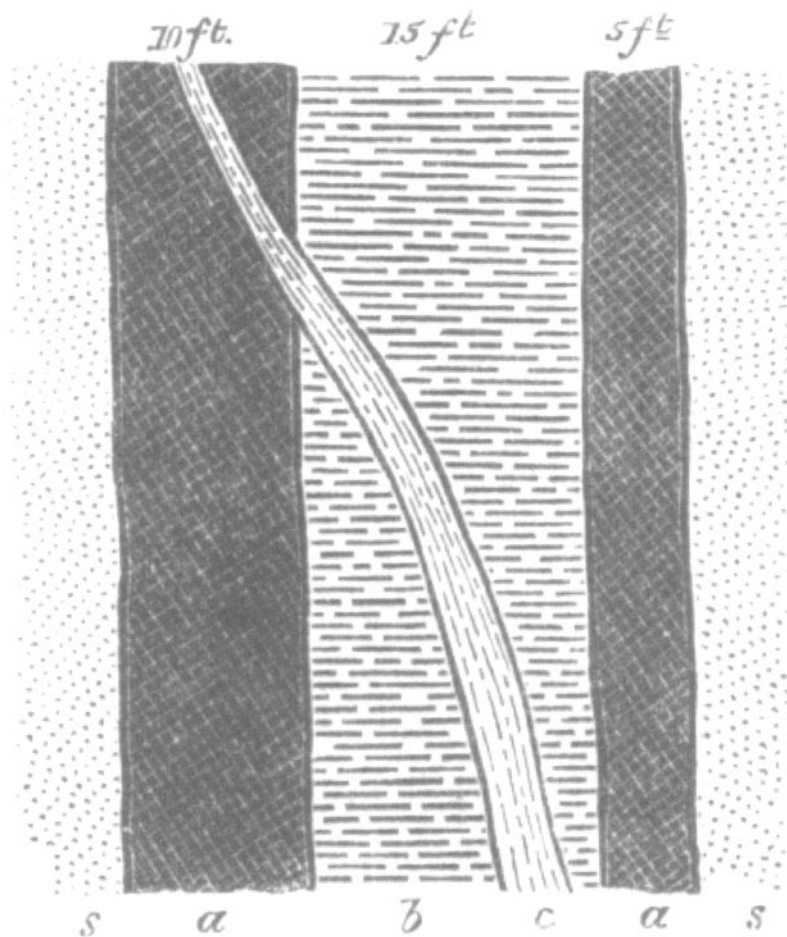
Illus 41 Diagrammatic plan of Judd's No. II Dyke: a = tholeiite; b = quartz-felsite (dacite); c = pitchstone-porphry (dacite); s = sandstone (Judd 1893, fig 3).
