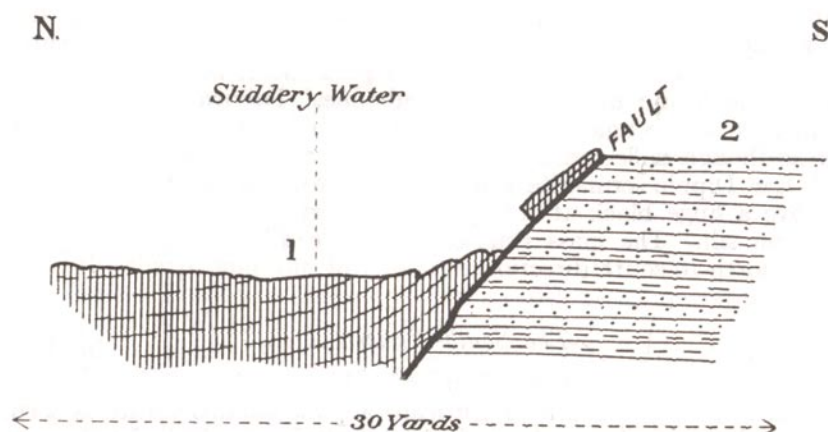
Illus 37 Junction of felsite against Triassic sediments, Slidery Water, just above Glenrie Bridge (Burrigan): 1 = felsite, with slabby jointing; 2 = Triassic sediments (Tyrrell 1928, fig 29).
