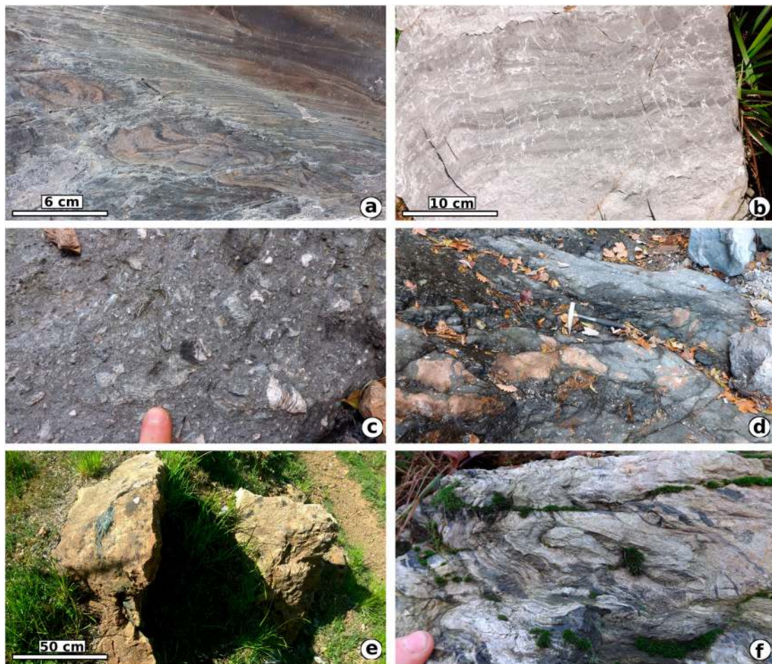
Figure 2. Some lithologies cropping out in the Forno Volasco area. (a) Centimetric alternation of metarenites and metapelites of the Pseudomacigno Fm. cropping out at SE of Casa Castellaccio. (b) Breccia at the base of the Grezzoni Fm., cropping out near Grotta del Vento. (c) Coarse metabreccia (Vinca Fm.) with clasts of phyllites, quartz veins, and tourmalinite. Outcrops below the Forno Volasco-Vergemoli road, close to the Fontanaccia area, at north of Le Buge. (d) Dolostone layer intercalated within black and gray/green metapelites, and metasandstones of the Vinca Fm. Same outcrop of (c). (e) Massive dolostone with iron oxides mineralization belonging to the Grezzone Metallifero Fm., along the road from Trimpello to Vergemoli. (f) Phyllites (Filladi Inferiori Fm.) with tourmalinite layers. Farneto, east of the Forno Volasco mining complex.
