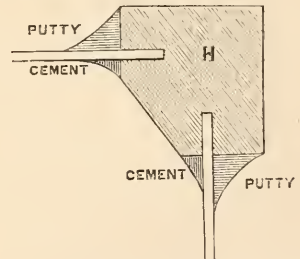
Fig. 14.—Method of Fastening Glass in Aquarium.
