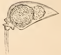
Fig. 58 b .—Side view. Animal retracted.
