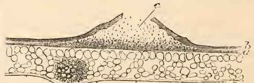
Fig. 149.— Melasmia acerina (section through a spermatogone). × 70.
