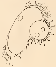
Fig. 25.— Sphærophrya , with short wavy tentacles, on Stylonychia .
