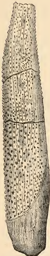
Fig. 2.— Asteracanthus ornatissimus (half nat. size, after Agassiz).
