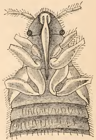
Fig. 41.— Æpophilus Bonnairei (underside × 16).
