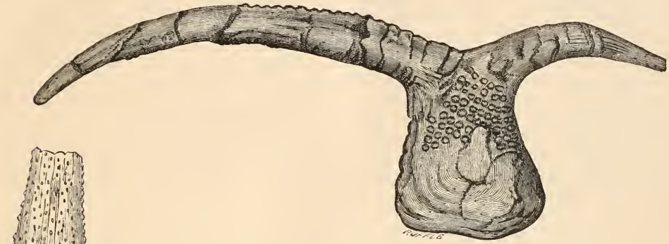
Fig. 1.— Erismacanthus Jonesii (after J. W. Davis).
