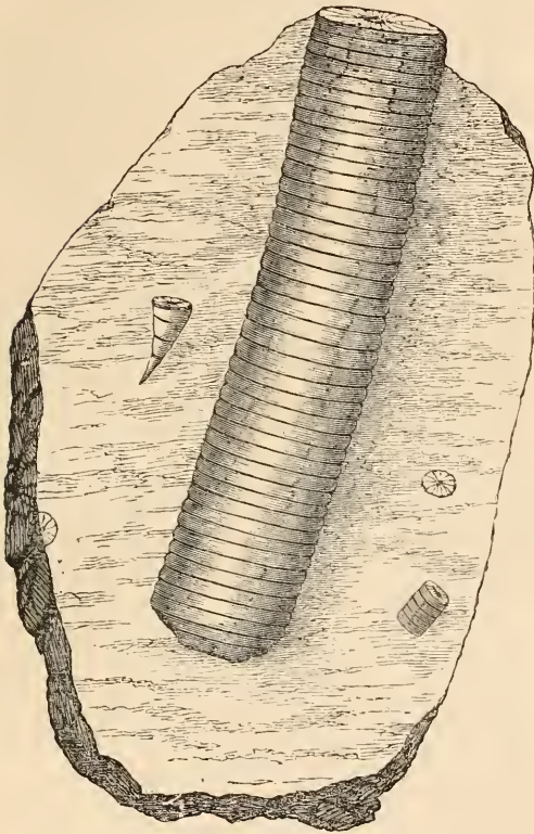
Fig. 140.—Stem of Encrinurus.
