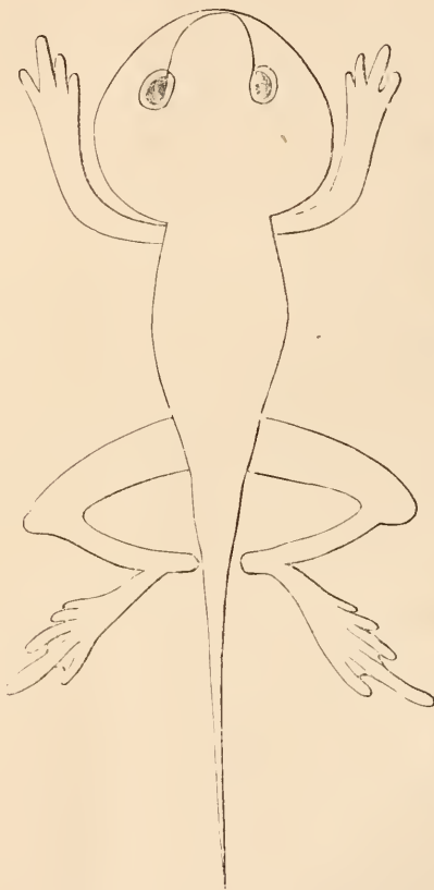
Fig. 78.—Second Frog Stage (enlarged).
