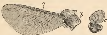
Fig. 116.—Single Samara, further developed (March 7, 1885): a, pteridium; b, simarre; c, tunica.
