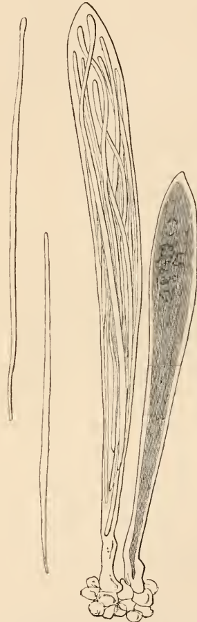
Fig. 152.—Two Asci, one immature, from the disk of Rhytisma acerinum , with two separate sporidia. \times 1000 .
