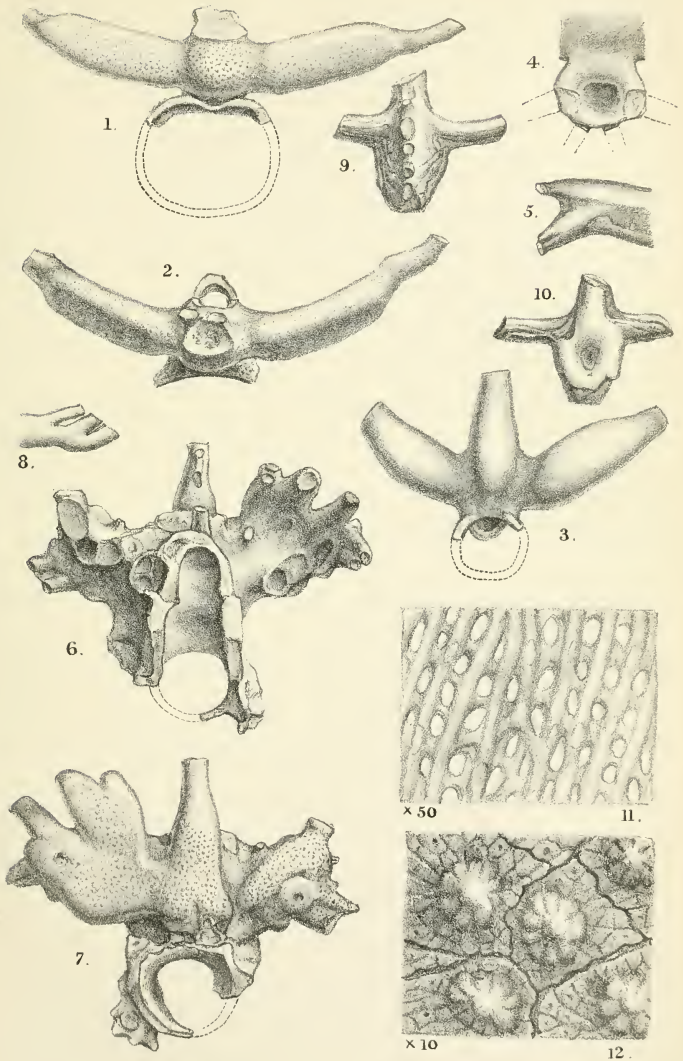
KERUNIA CORNUTA, Mayer-Eymar from the Eocene of Egypt.
