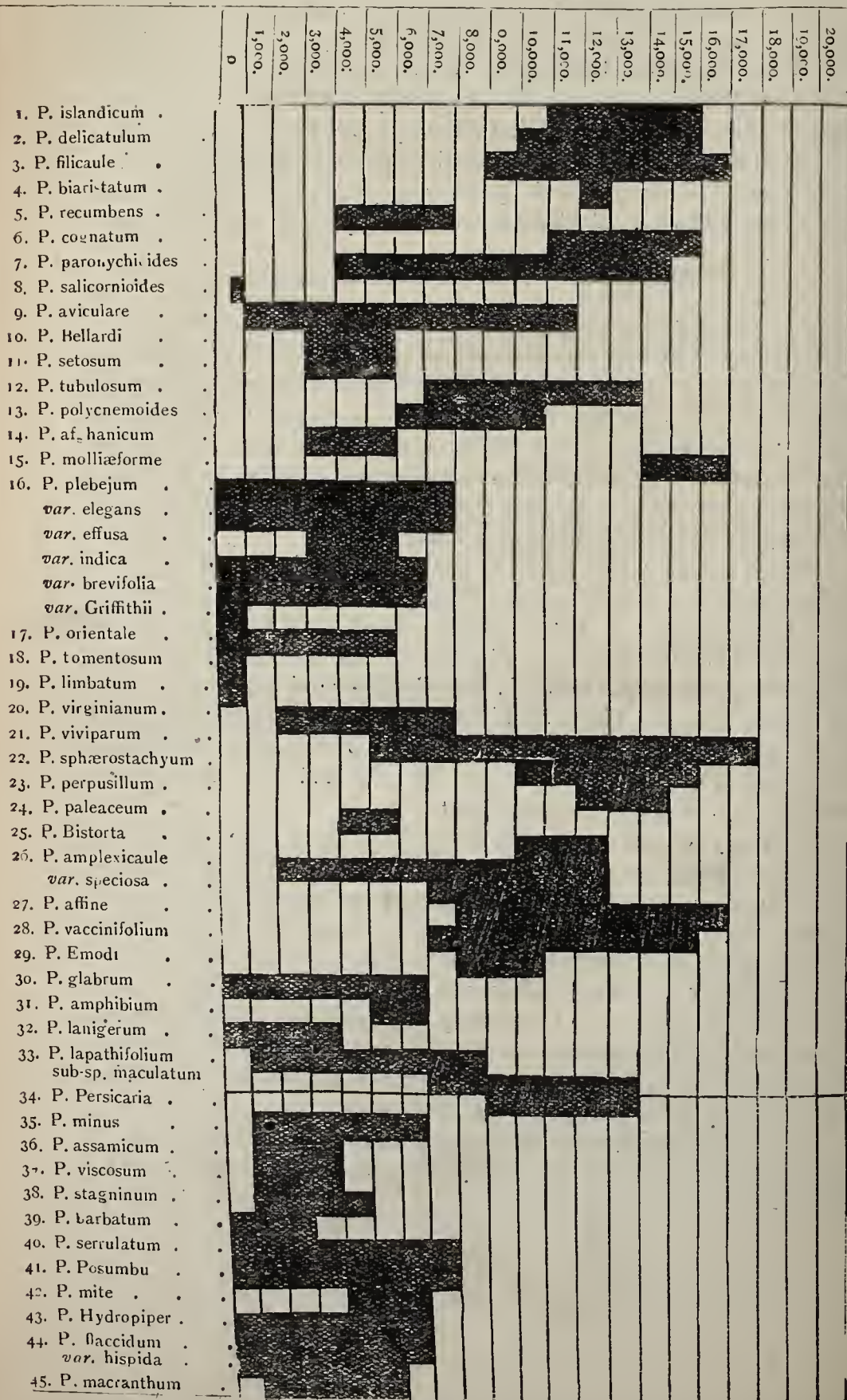
Altitudinal distribution of species in India.
