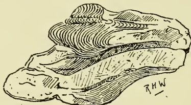
FIG. 1. Mica Schist from Hand Deeps.
