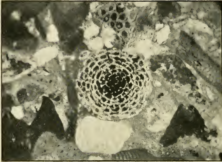
M. 77b. S. 11° W. Edd., 38.8 miles. Section of Planorbulina (? larvata ) in Eocene limestone. Ordinary light, \times 44 .
