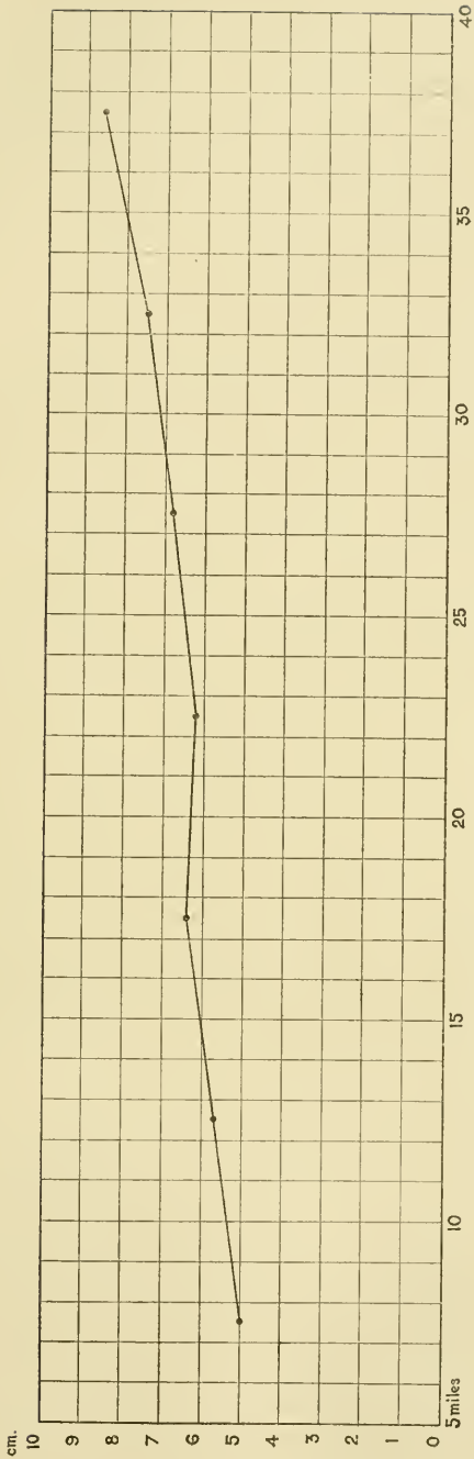
FIG. 1.—Average greatest dimension of stones for 5-mile intervals S. 17° E. from Eddystone.
