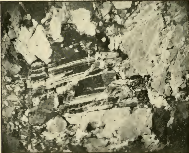
M. 62a. S. 25° W. Edd., 46.4 miles. Crushed plagioclase feldspar in chlorite schist. Crossed nicols. \times 29 .
