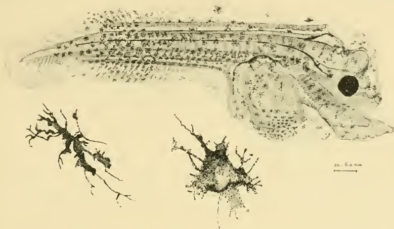
FIG. 6.— Solea lascaris . Length ca. 6 mm. Oithona Station, XCVIII. A. 25th Aug., 1913. Total depth 36 fms. Midwater haul.
