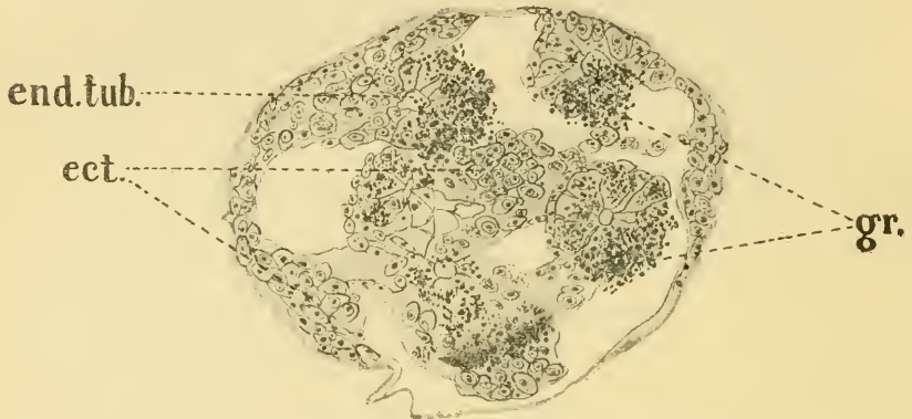
FIG. 9. \times 260 .—Section through a small restitution mass 35 days old, showing the formation of many granules in the endoderm cells. Some of these cells are breaking down, so that the tubules are less distinct. The ectoderm cells remain healthy. Ect. , ectoderm cells; end. tub. , endoderm tubules; gr. , cytoplasmic granules.
