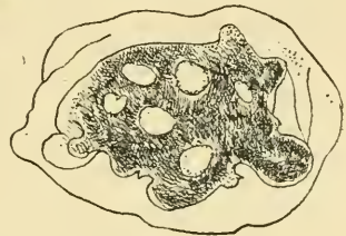
FIG. 6. \times 16 .—A restitution mass 34 days old, showing well-marked shrinkage away from the perisarc and fenestrated appearance of the cell mass.
