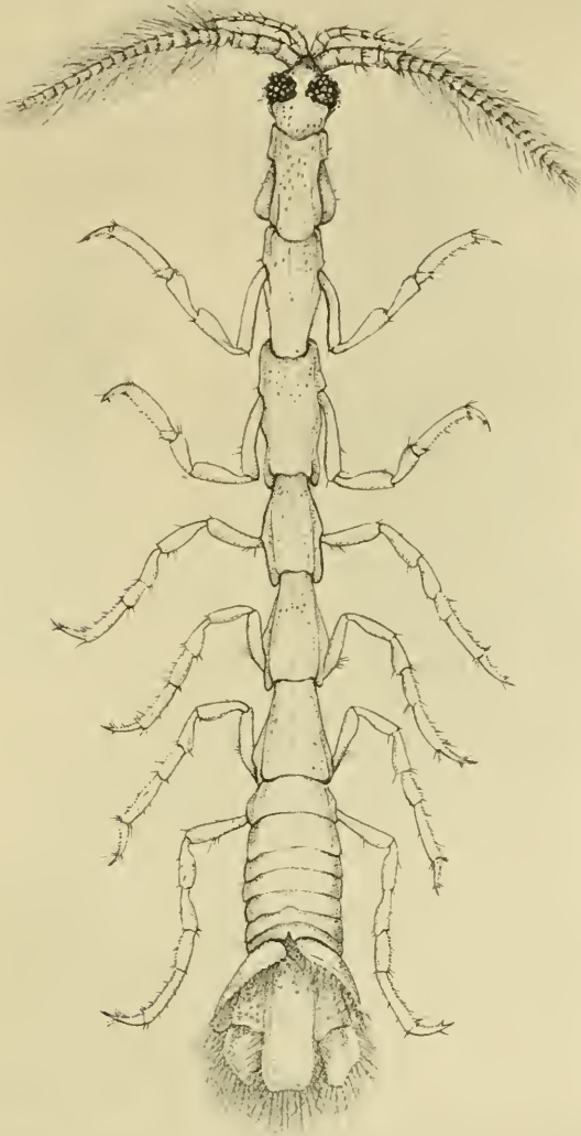
Anthura gracilis . FIG. 1.—♂, dorsal view. Eddystone specimen, \times 17 .
