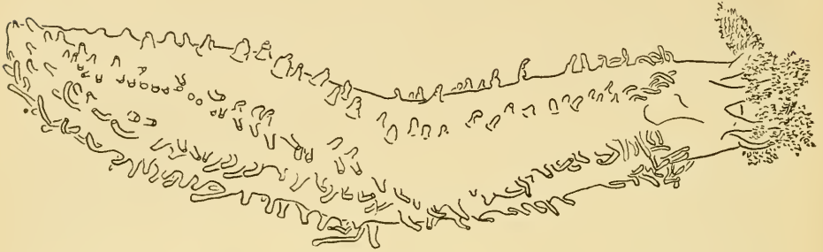
FIG. 9.—View of Cucumaria saxicola , showing the five ambulacral rows ( \times \frac{3}{4} ).
