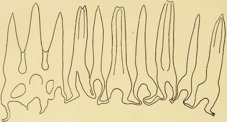
FIG. 4.—External view of the calcareous collar of C. saxicola drawn from a glycerine preparation after separating the ventral piece from the adjacent right radial piece ( \times \frac{2}{3} ).
