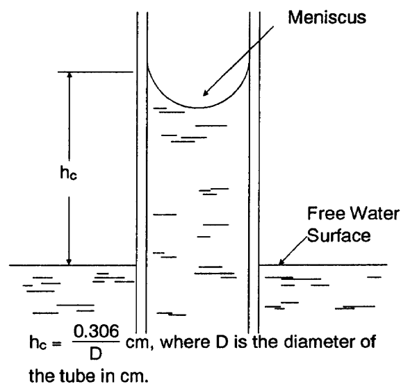
Figure 4-13. Capillary rise of water in small tubes.
