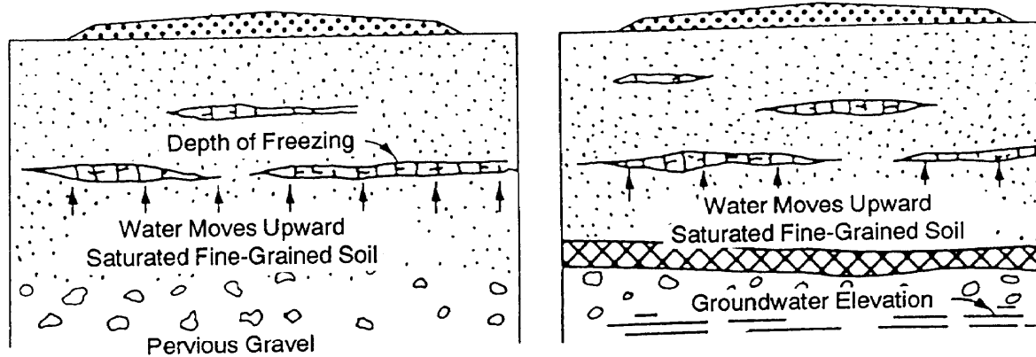
Figure 7-7. Sources of water that feed growing ice lenses.
