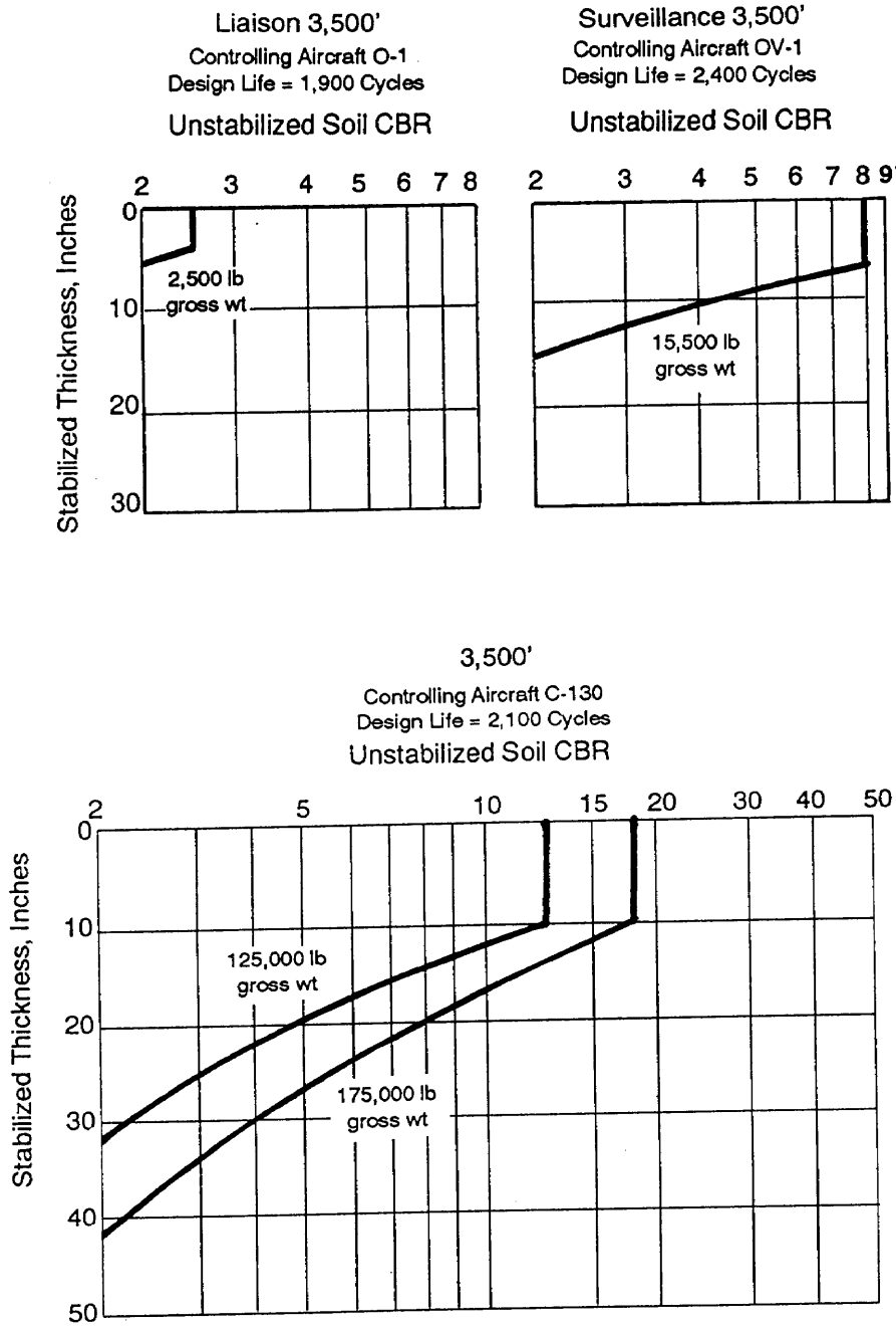
Figure 9-22. Design curves for single-layer airfields using stabilized soils in rear areas.
