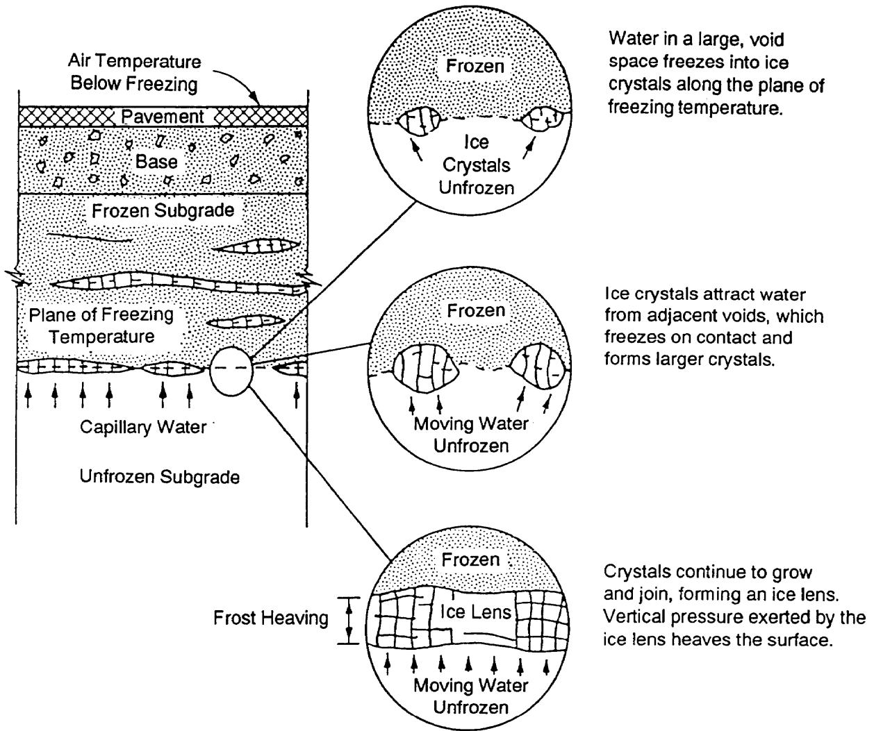
Figure 7-6. Formation of ice crystals on frost line.
