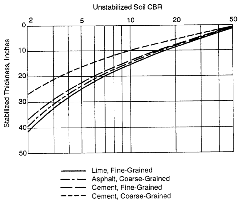
Figure 9-17. Design curve for Class C multilayer roads using stabilized soils.
