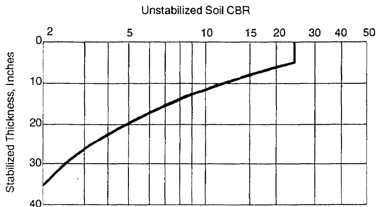
Figure 9-15. Design curve for Class E single-layer roads using stabilized soils.
