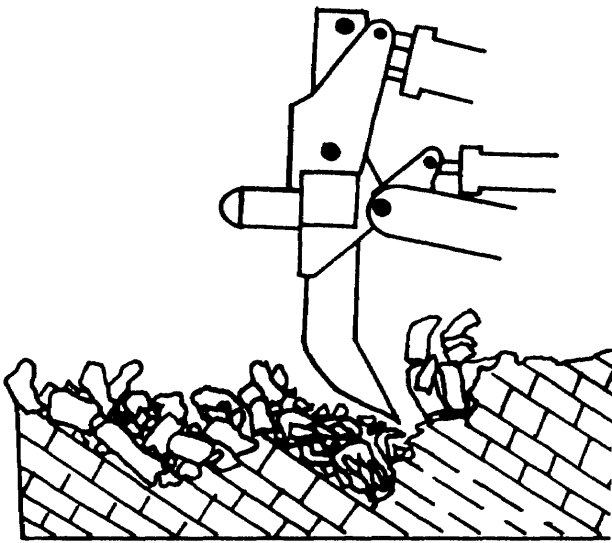
Figure 2-32. Ripping in the direction of dip.
