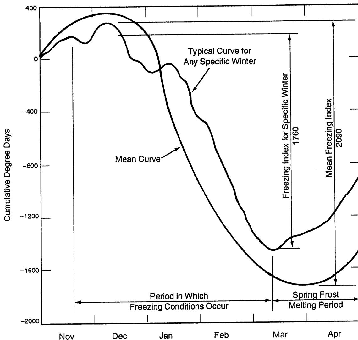
Figure 7-5. Determination of freezing index.
