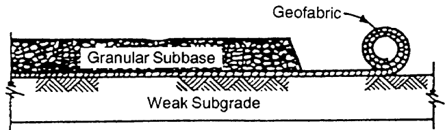
Figure 11-3. Separating a weak subgrade from a granular subbase with a geofabric.
