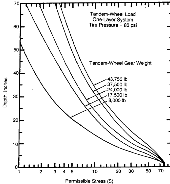
Figure 11-7. Thickness design curve for tandem-wheel load on gravel-surfaced pavements.
