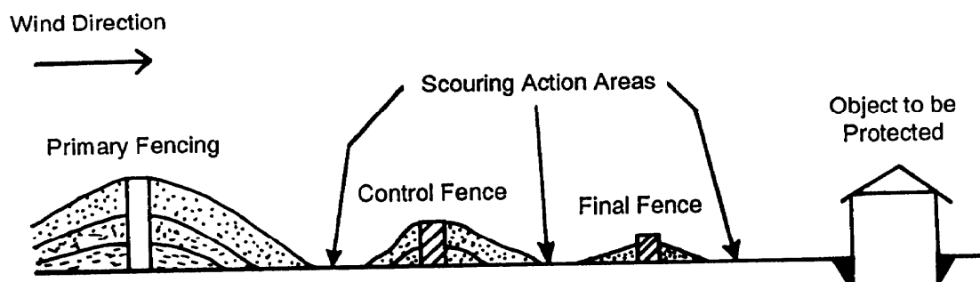
Figure 9-35. Three fences installed to control dune formation.
