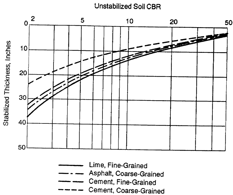
Figure 9-19. Design curve for Class E multilayer roads using stabilized soils.
