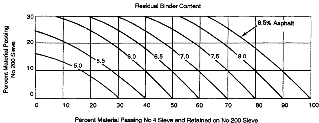
Figure 9-10. Selection of asphalt cement content.
