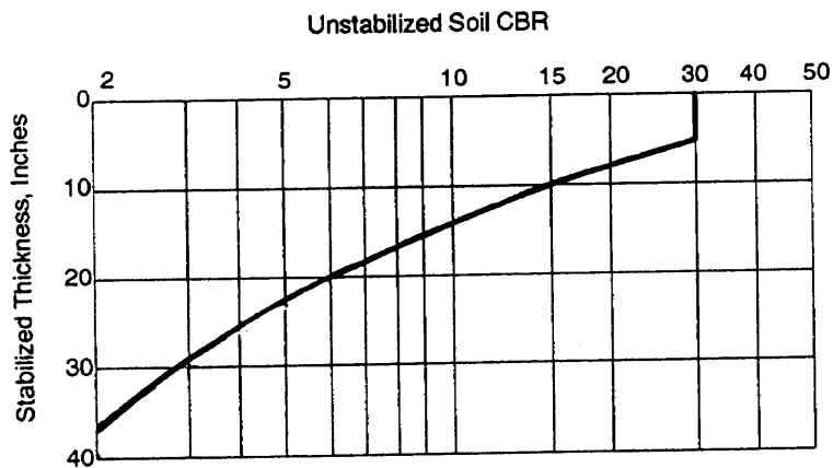
Figure 9-14. Design curve for Class D single-layer roads using stabilized soils.
