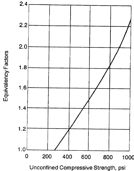
Figure 9-20. Equivalency factors for soils stabilized with cement, lime, or cement and lime mixed with fly ash.
