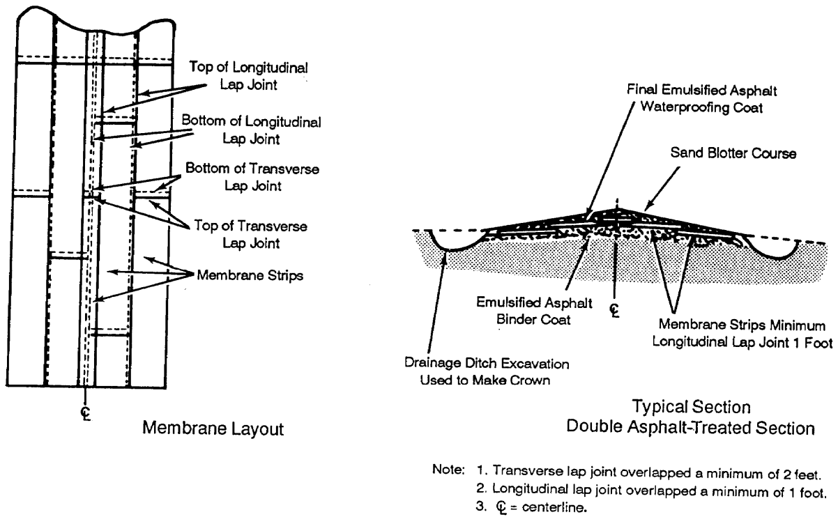
Figure 9-31. Polypropylene membrane layout for tangential sections.
