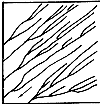
(b) Parallel
