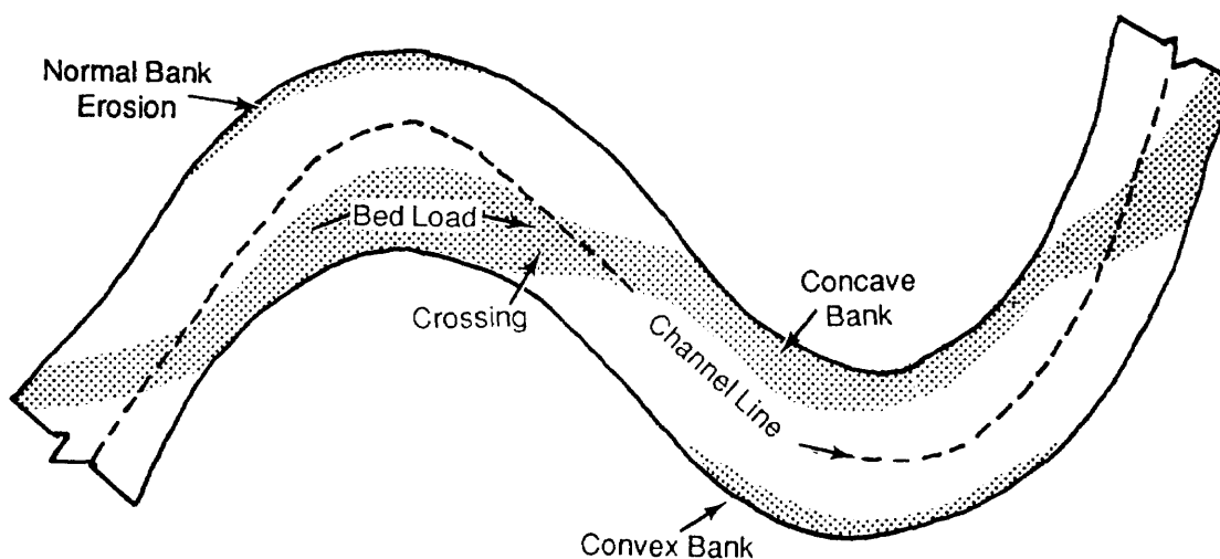
Figure 3-7. Meander erosion and deposition.
