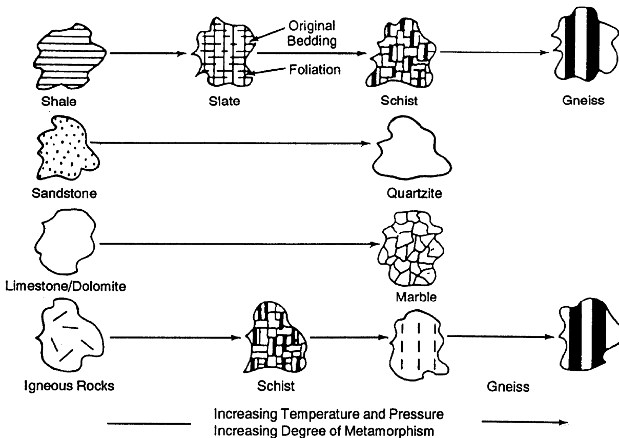
Figure 1-12. Metamorphism of existing rocks.
