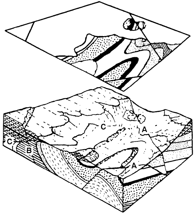
Figure 2-29. Outcrop patterns produced by faulting.
