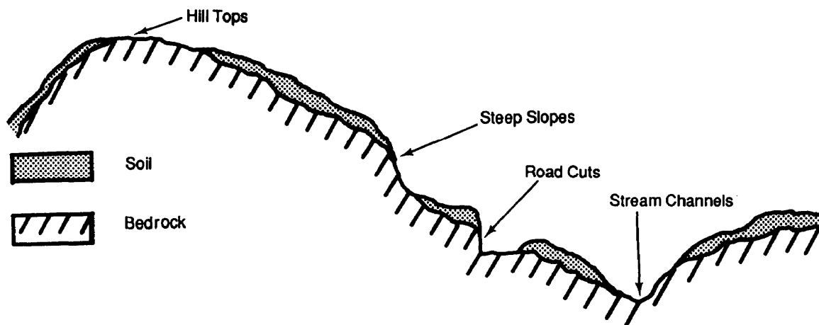
Figure 2-3. Location of rock outcrops.
