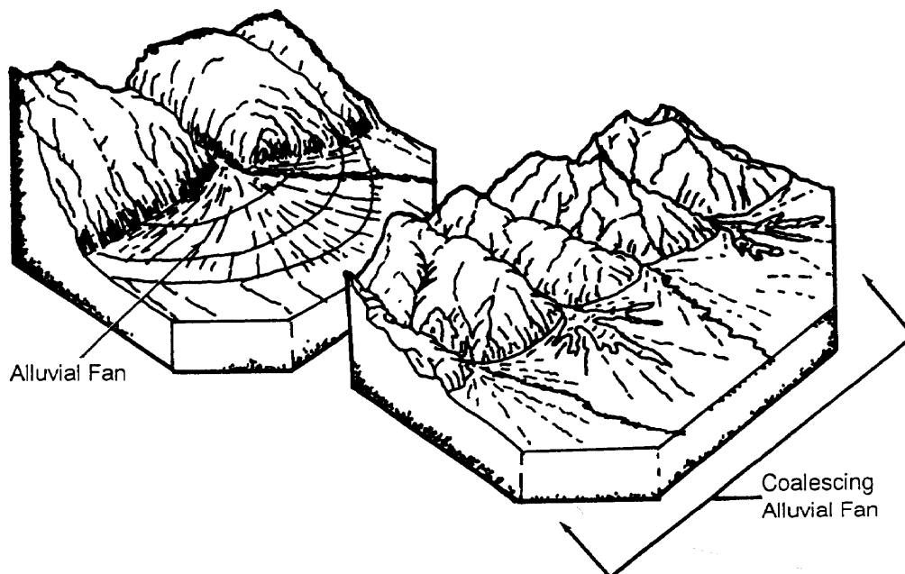
Figure 3-16. Alluvial fan and coalescing alluvial fans.
