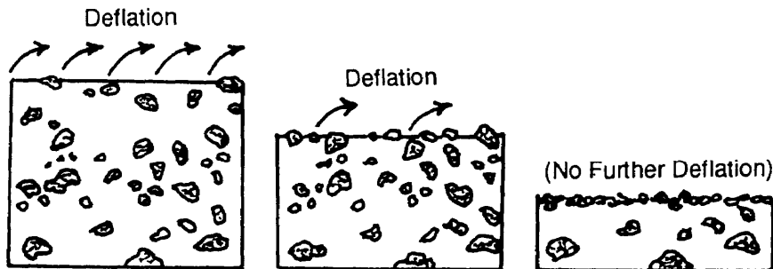
Figure 3-30. Three stages illustrating the development of desert armor.
