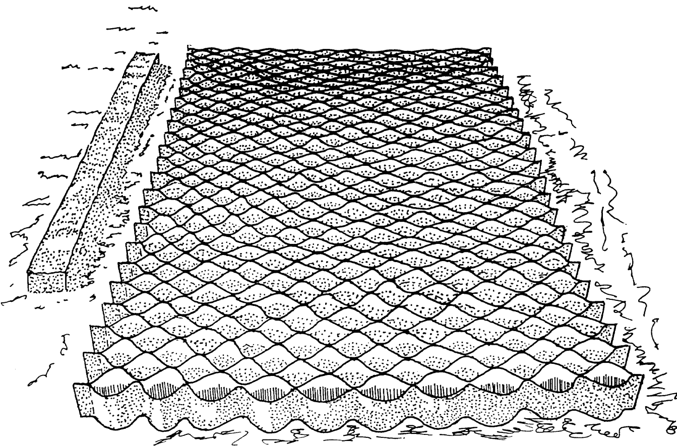
Figure 11-10. Sand grid.
