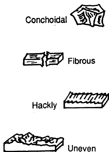
Figure 1-3. Fractures.
