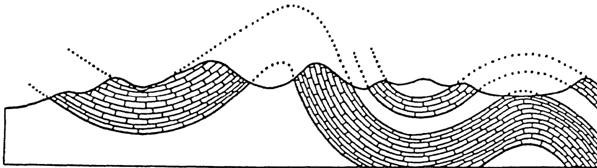
Figure 2-4. Folding of sedimentary rock layers.
