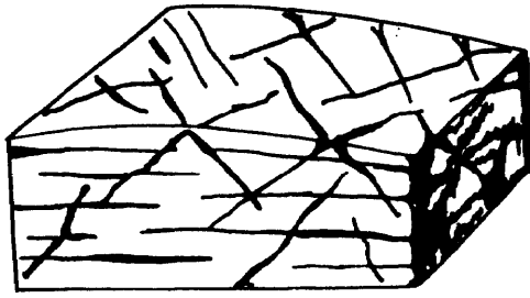
Jointed Intrusion
