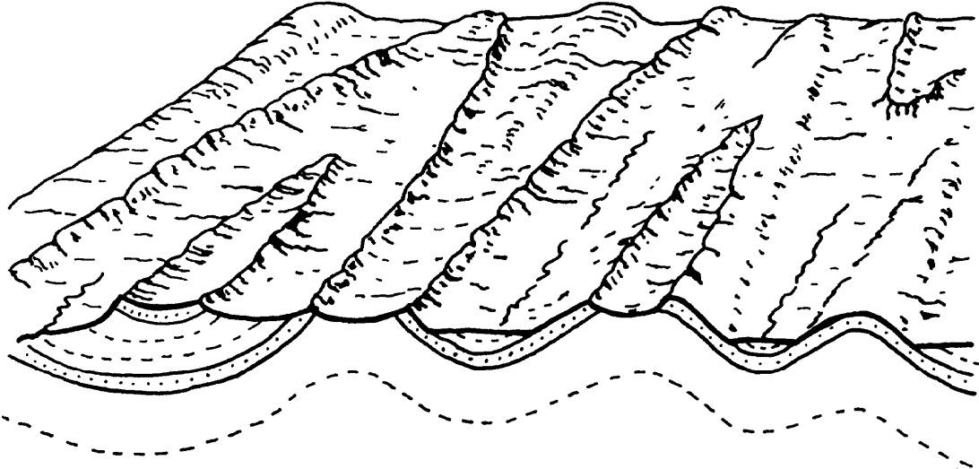
Figure 2-6. Topographic expression of plunging folds.
