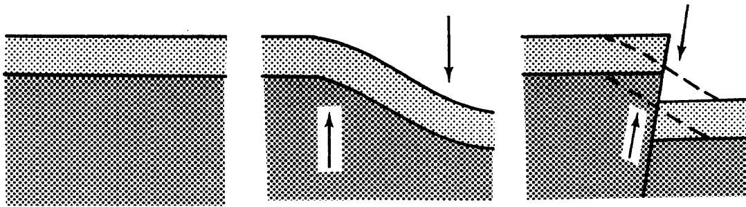
Figure 2-8. Faulting.
