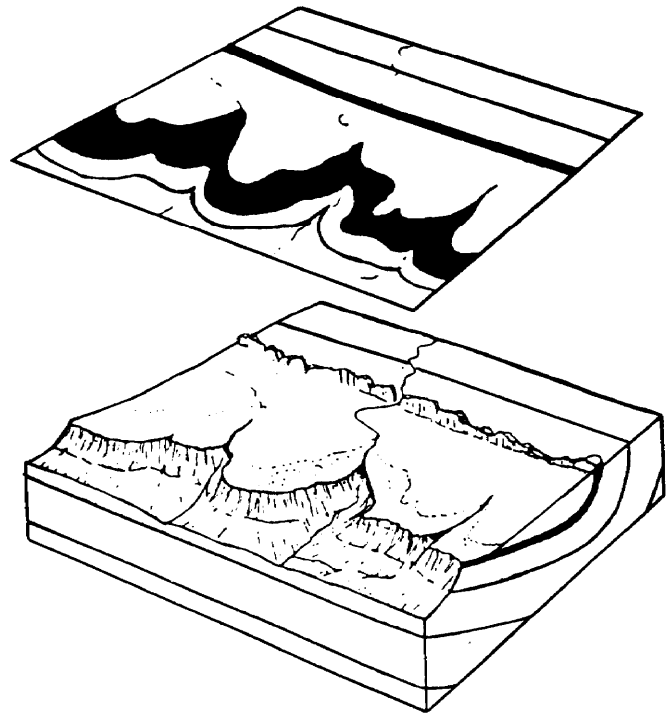
Figure 2-25. Outcrop patterns of inclined strata.
