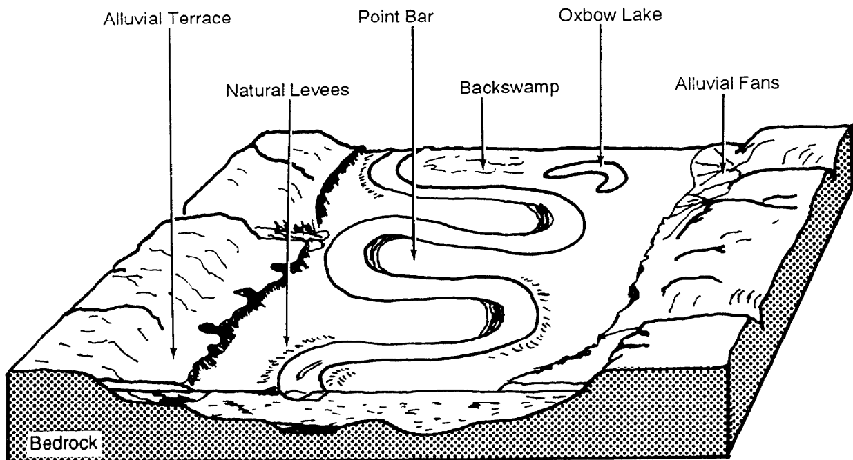
Figure 3-19. Major floodplain features.
