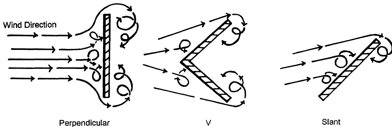
Figure 9-36. Three types of solid fencing or paneling for control of dune formation.
