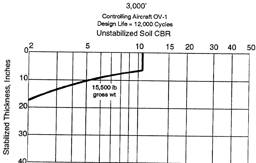
Figure 9-26. Design curves for single-layer airfields using stabilized soils in liaison COMMZ airfields
