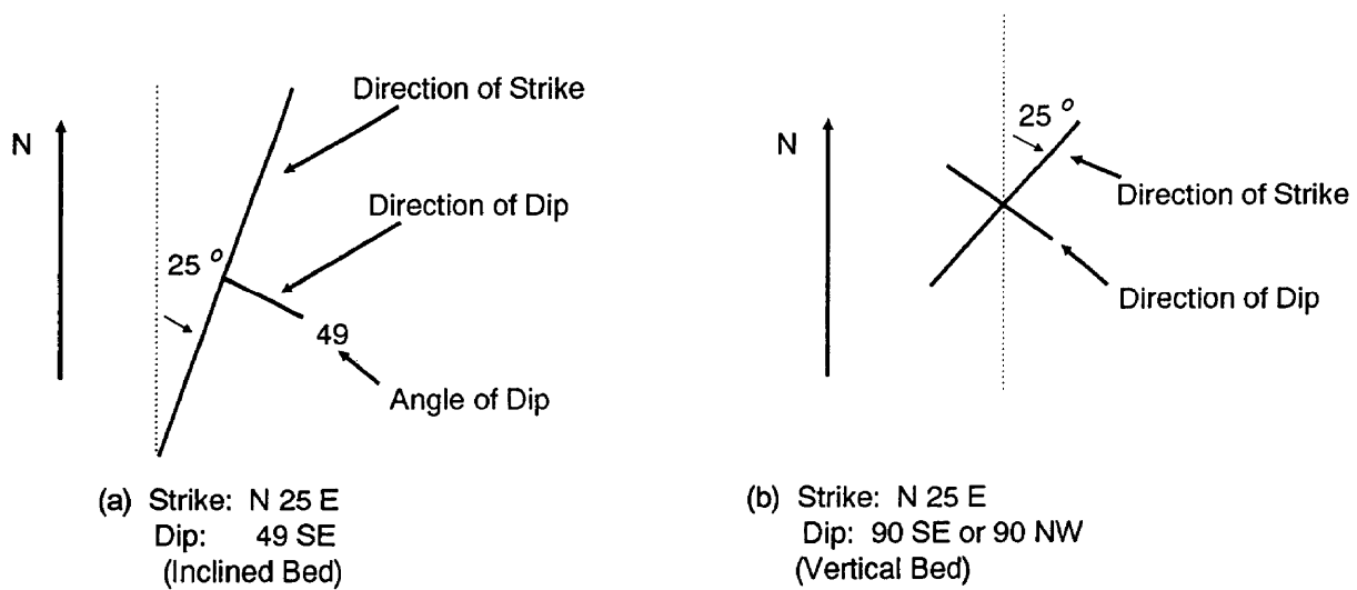
Figure 2-17. Measuring strike and dip with a Brunton compass.
