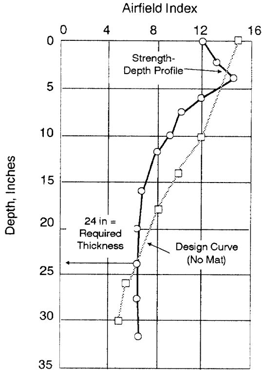
Figure 9-30. Thickness design procedure for subgrades that decrease in strength with depth.
