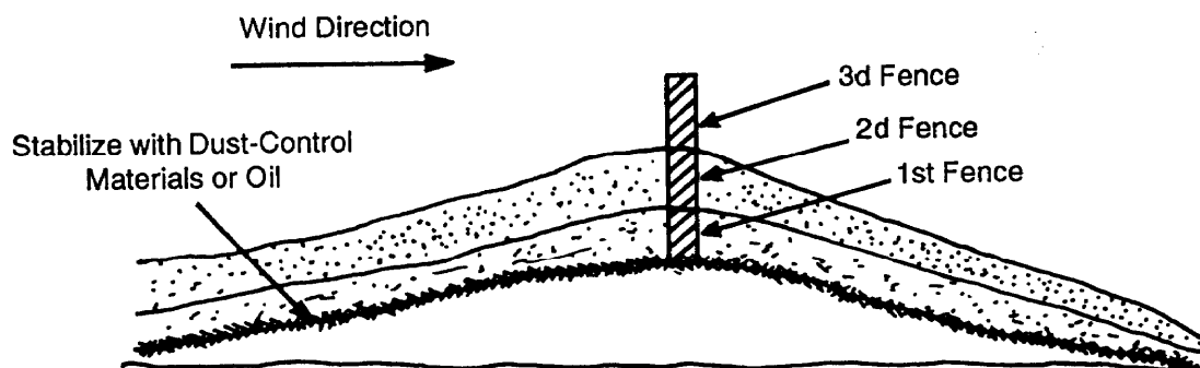
Figure 9-34. Cross section of dune showing initial and subsequent fences.
