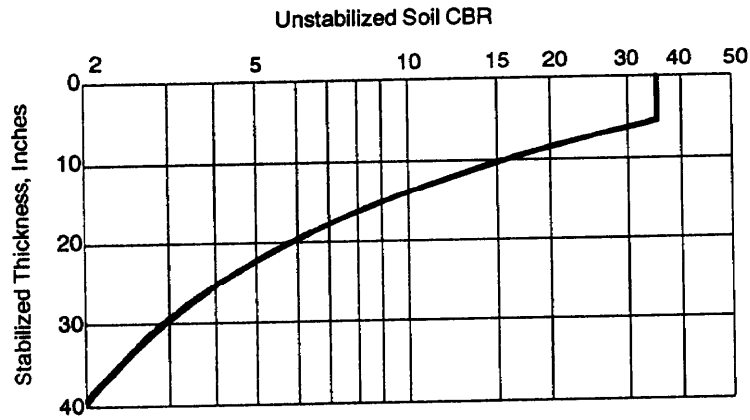
Figure 9-13. Design curve for Class C single-layer roads using stabilized soils.
