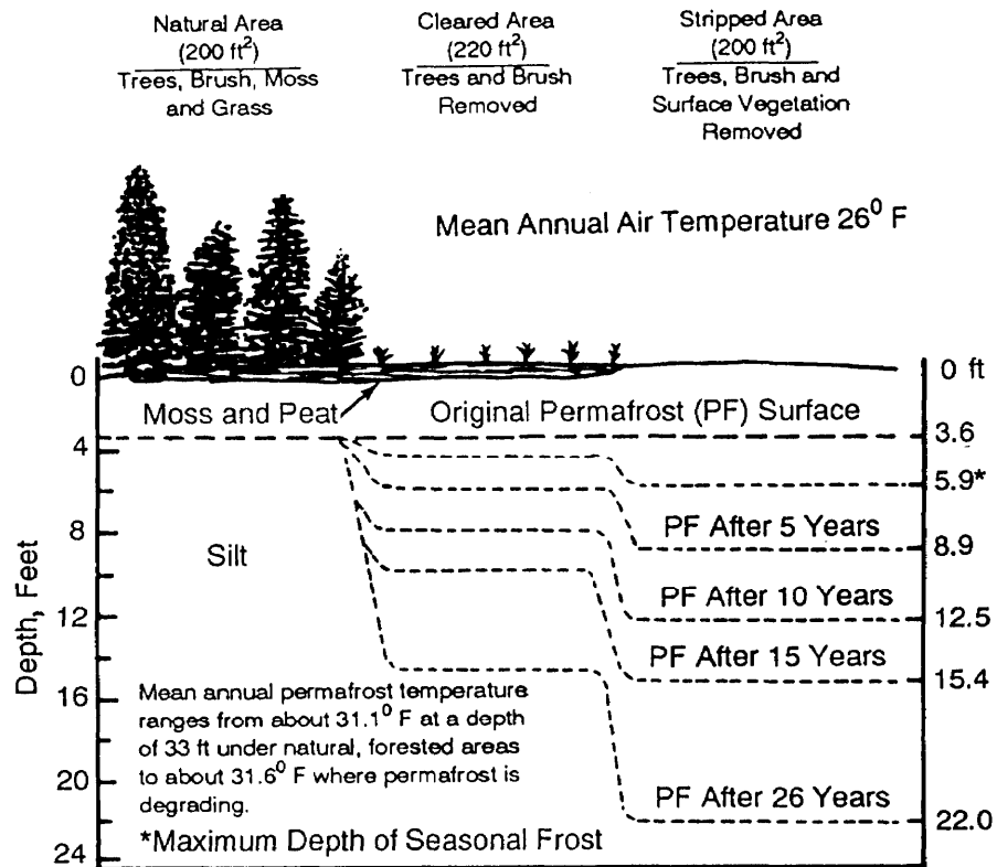
Figure 12-8. Permafrost degradation under different surface treatments.
