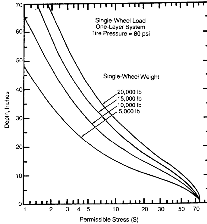
Figure 11-5. Thickness design curve for single-wheel load on gravel-surfaced pavements.
