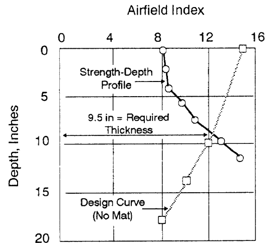
Figure 9-29. Thickness design procedure for subgrades that increase in strength with depth.
