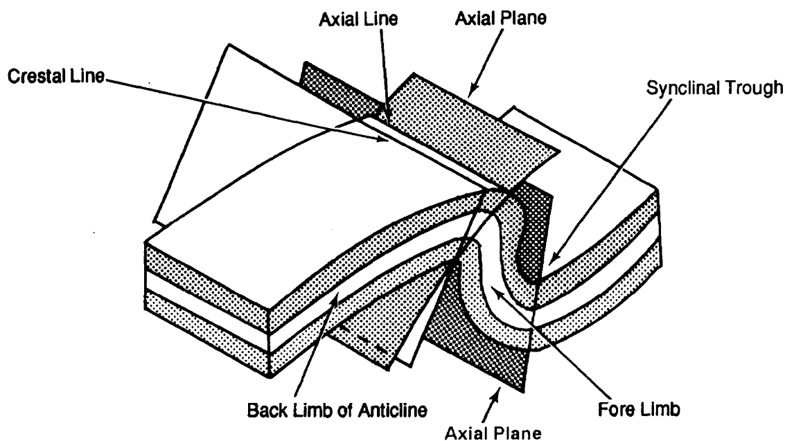
Figure 2-7. Fold symmetry.
