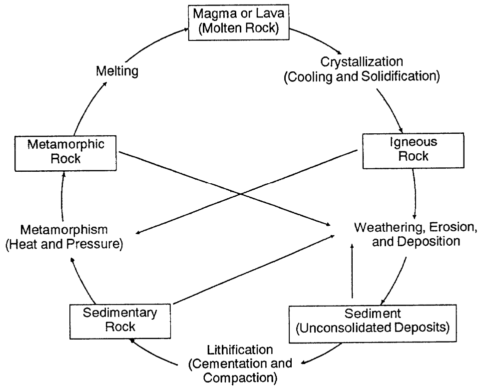
Figure 1-4. The rock cycle.
