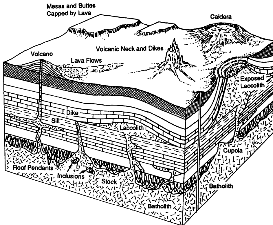
Figure 1-5. Intrusive and extrusive rock bodies.
