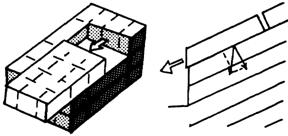
Figure 2-34. Rock slide on inclined bedding plane.
