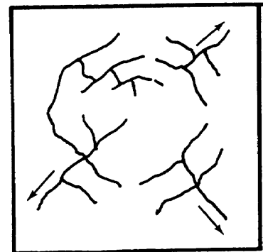
(f) Annular
