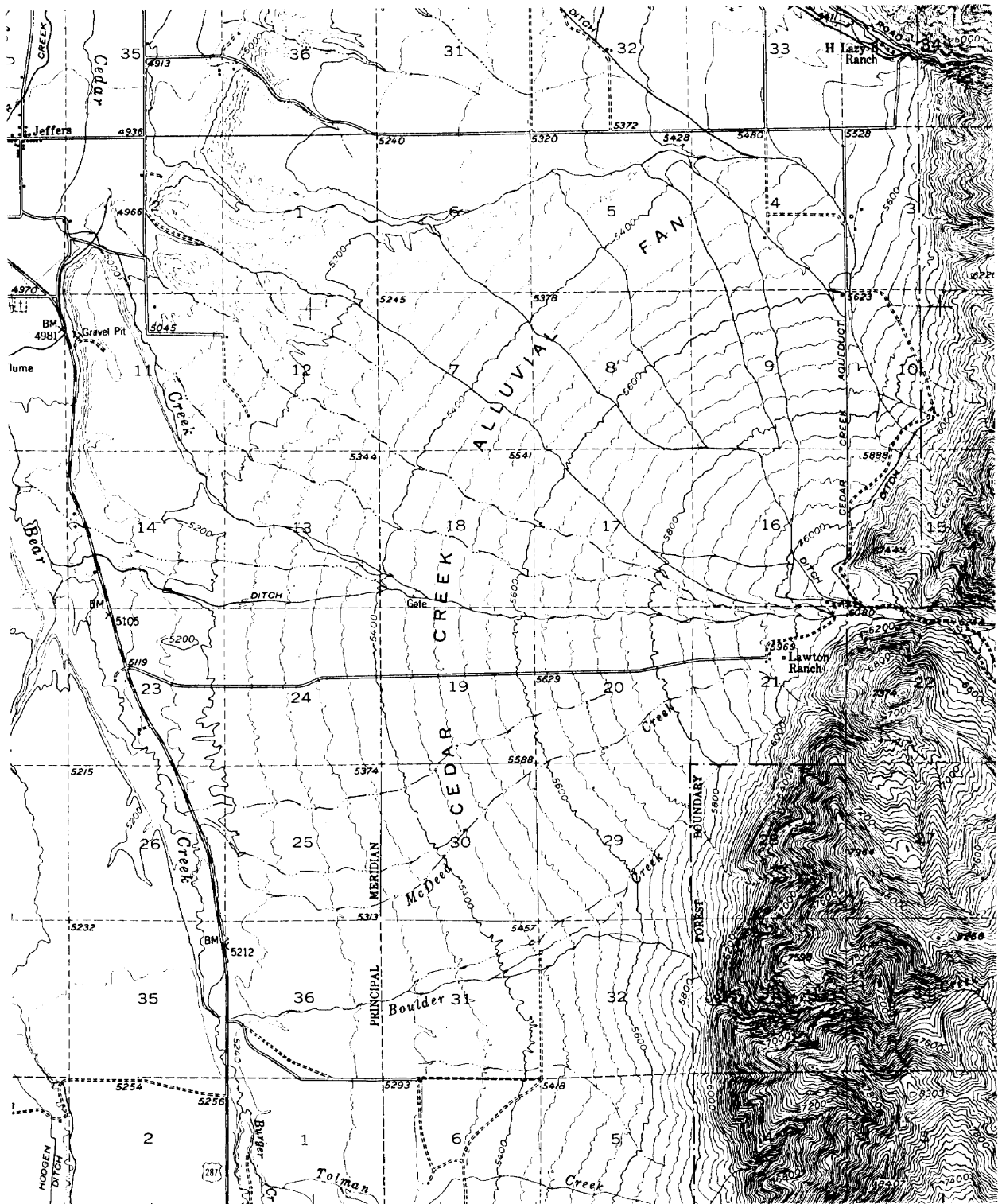
Figure 3-17. Cedar Creek alluvial fan.
