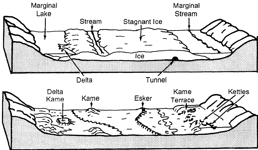
Figure 3-25. Valley deposits from melting ice.
