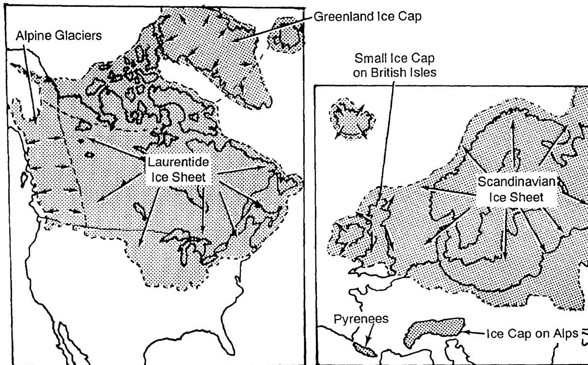
Figure 3-21. Ice sheets of North America and Europe.
