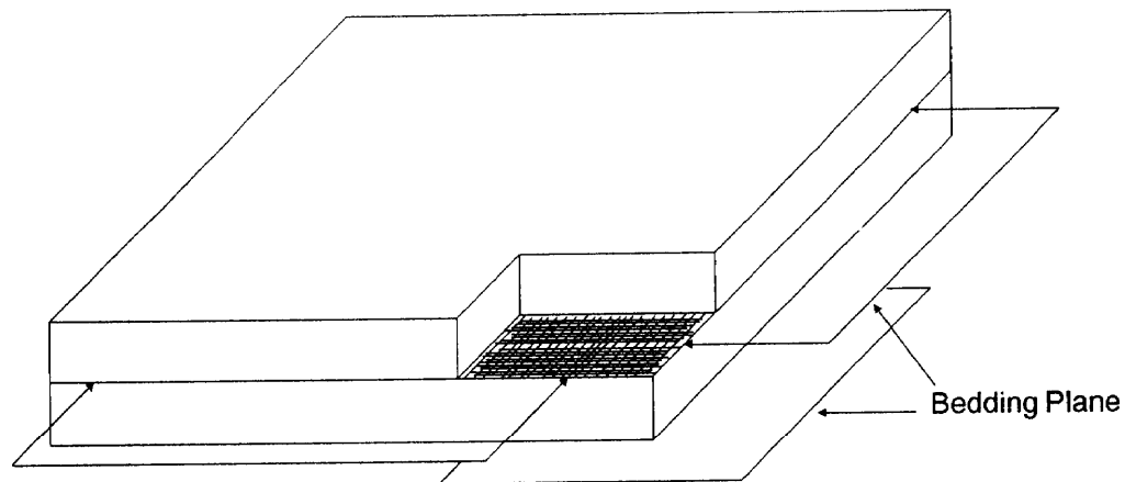
Figure 1-7. Bedding planes.
