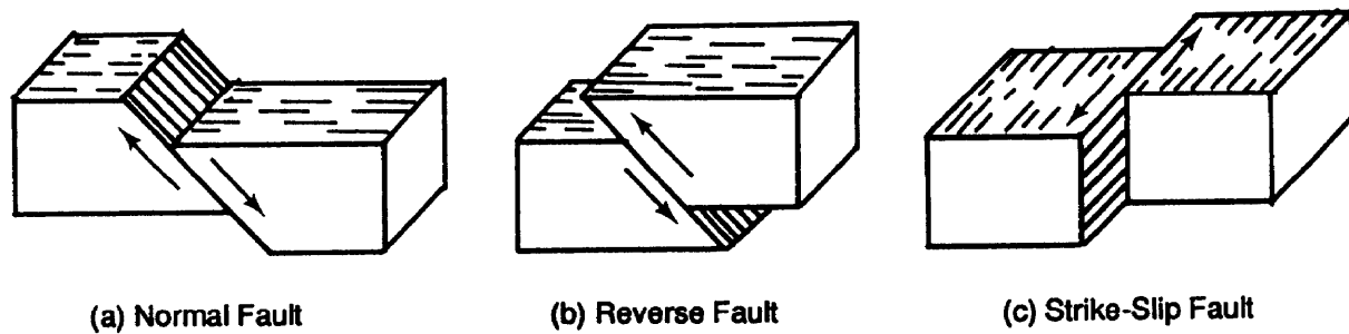
Figure 2-12. Types of faults.
