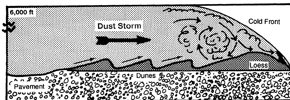
Figure 3-32. Eolian features.
