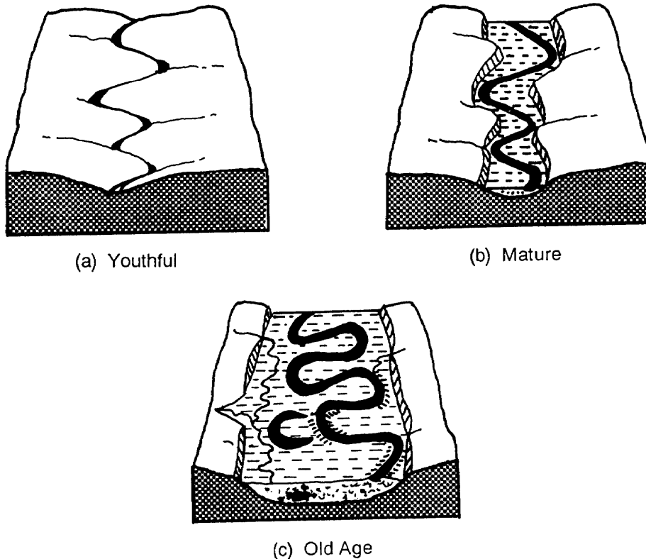
Figure 3-3. Stream evolution and valley development.
