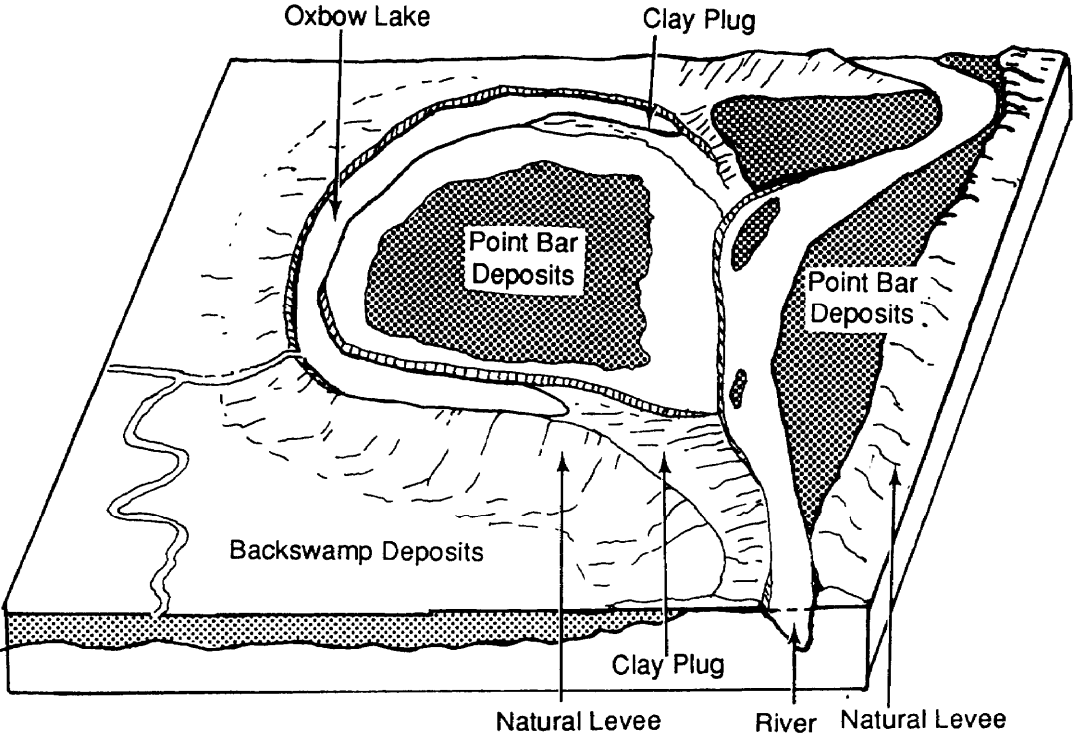
Figure 3-10. Meander development and cutoff.
