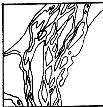
(g) Braided
