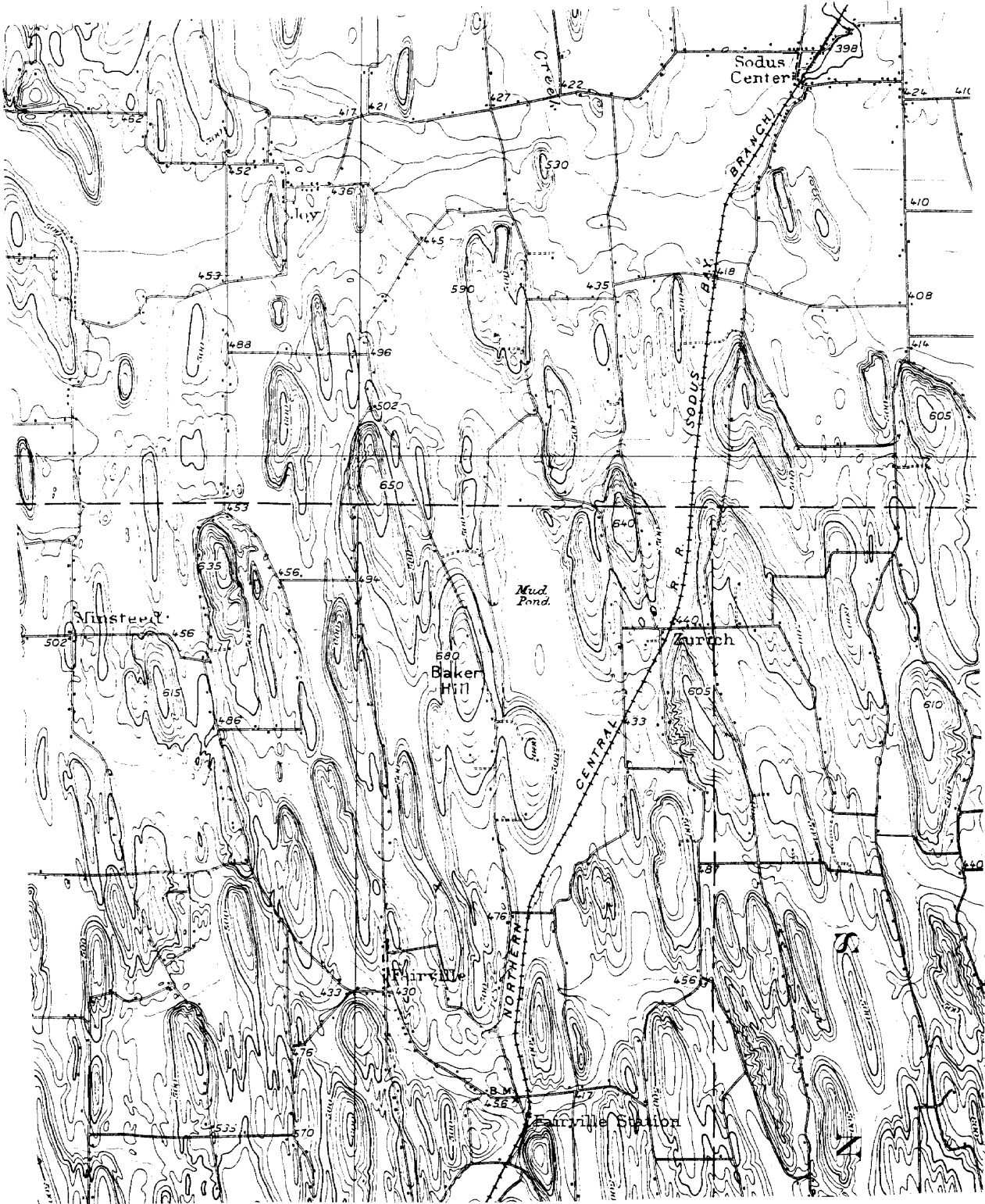
Figure 3-27. Topographic expression of a drumlin field.
