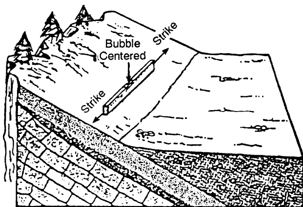
Figure 2-15. Strike.
