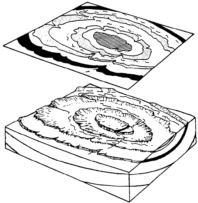
Figure 2-27. Outcrop patterns of an eroded basin.
