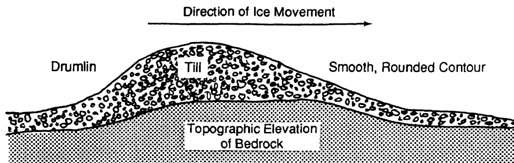
Figure 3-26. Idealized cross section of a drumlin.
