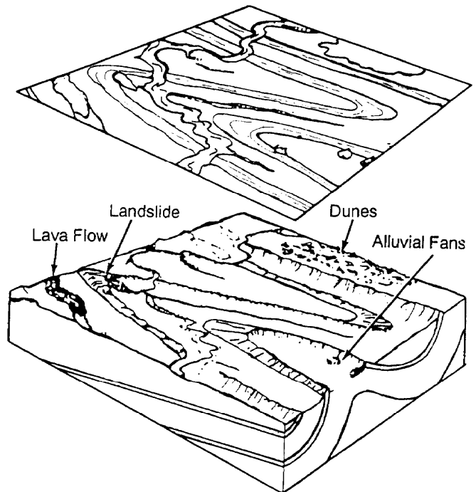
Figure 2-31. Outcrop patterns of surficial deposits.
