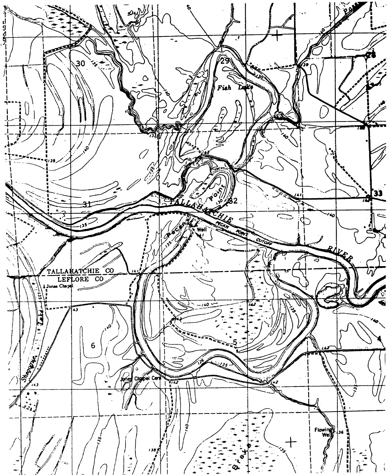
Figure 3-6. An old age stream valley.
