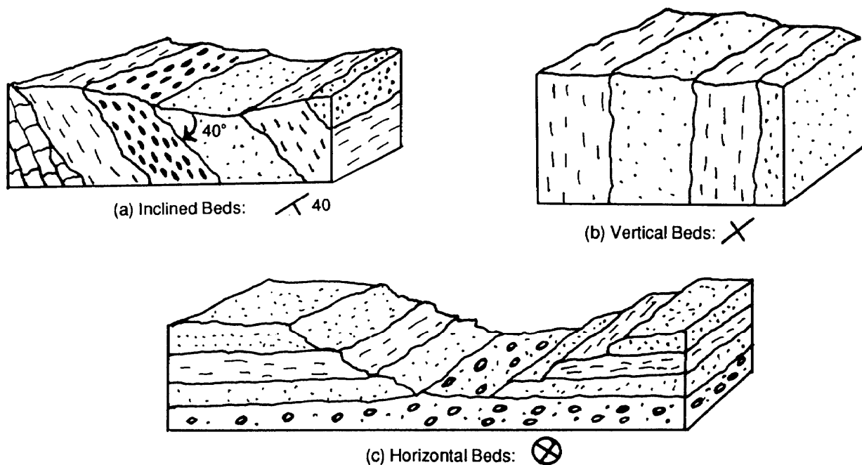
Figure 2-19. Strike and dip symbols of sedimentary rocks.
