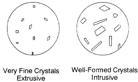
Figure 1-6. Cross section of igneous rock.
