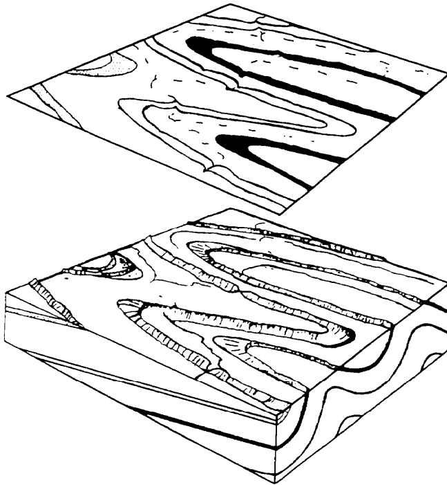
Figure 2-28. Outcrop patterns of plunging folds.
