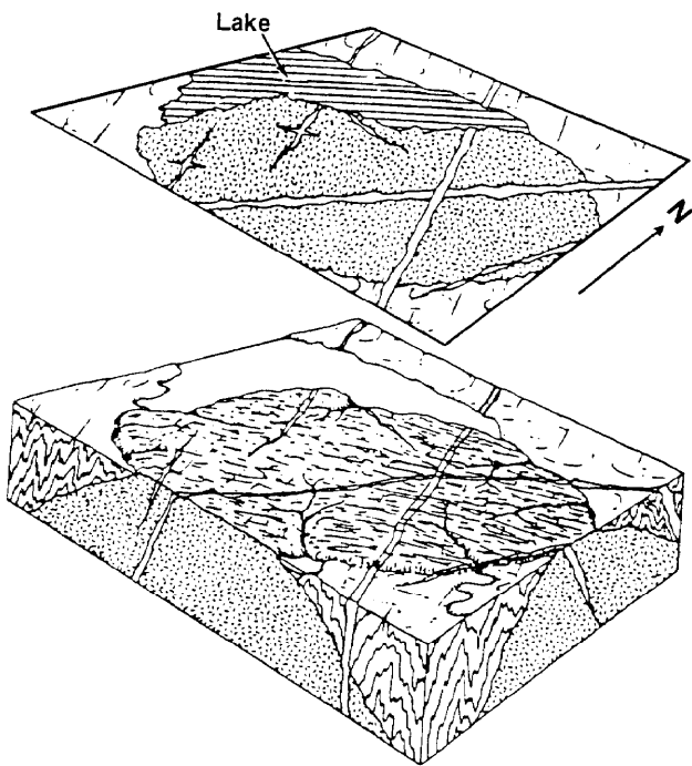
Figure 2-30. Outcrop patterns of intrusive rocks.
