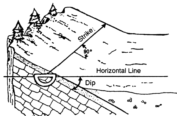
Figure 2-16. Dip.
