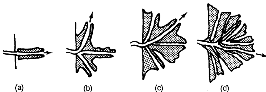
Figure 3-14. Growth of a simple delta.
