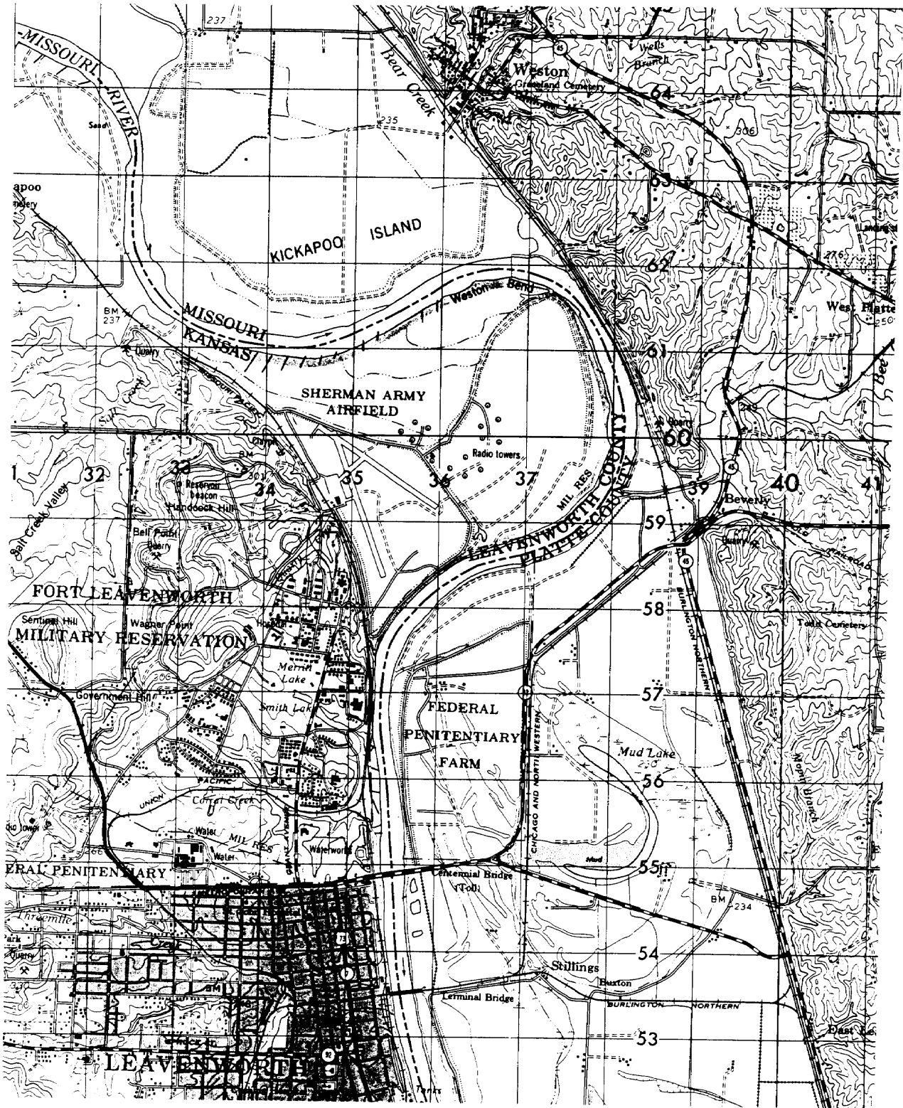
Figure 3-5. A mature stream valley.
