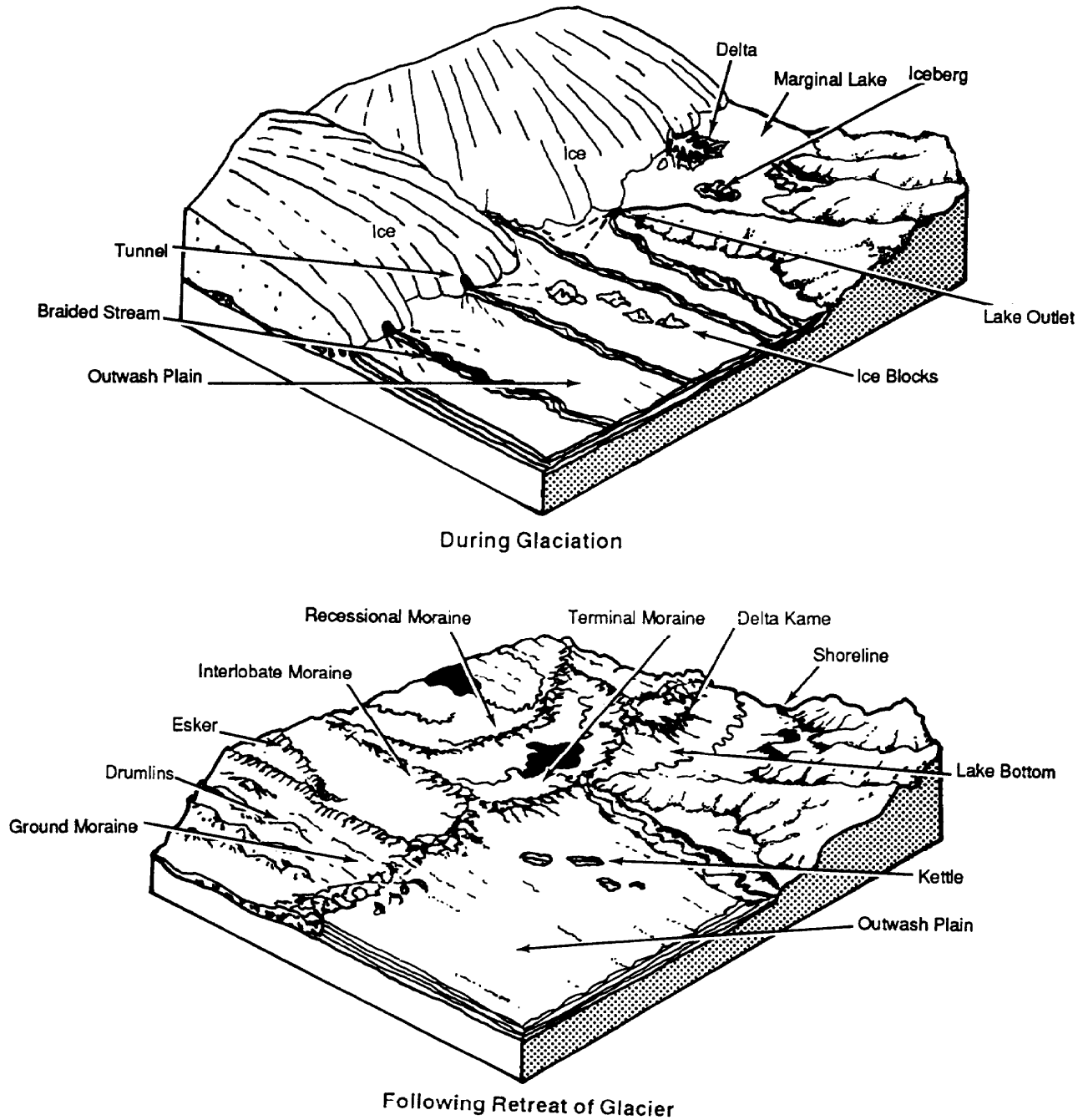
Figure 3-22. Continental glaciation.
