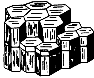
Columnar Jointing
