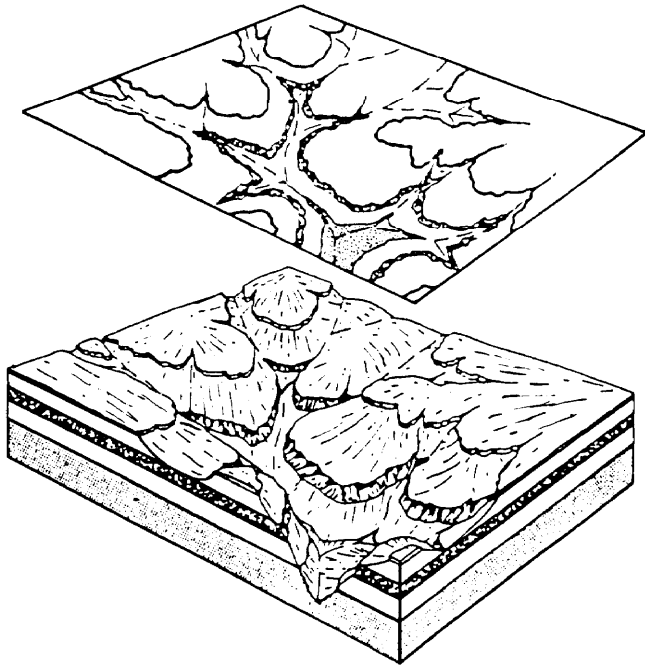
Figure 2-24. Outcrop patterns of horizontal strata.
