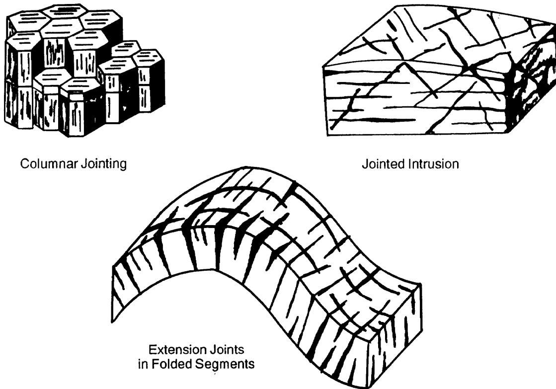
Figure 2-14. Jointing in sedimentary and igneous rock.
