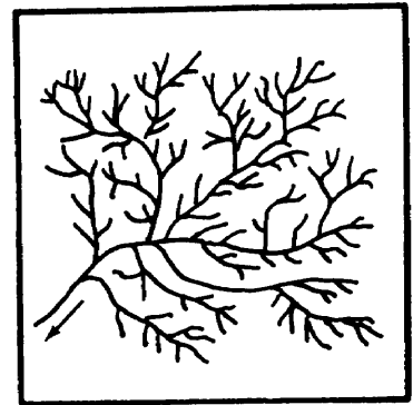
(c) Dendritic
