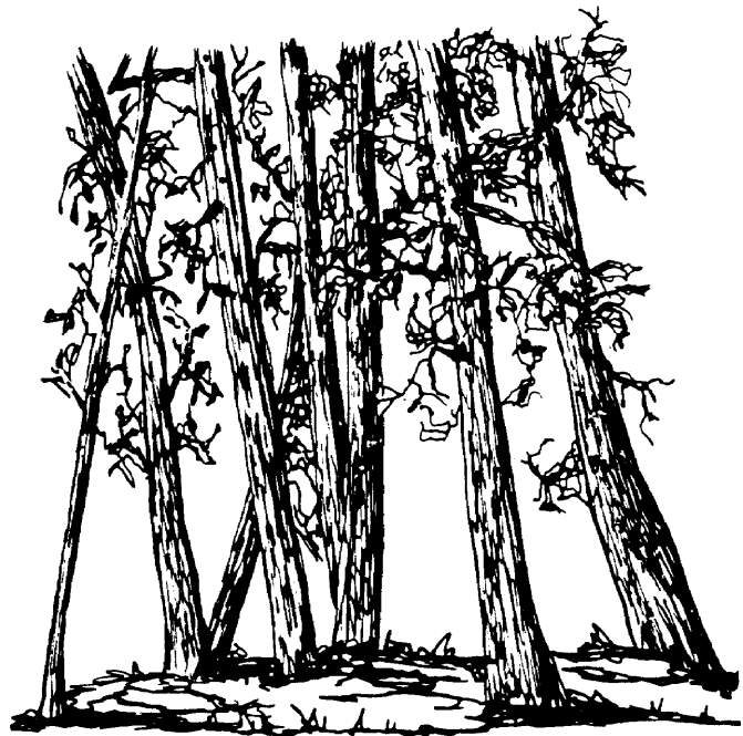
Figure 10-9. Jackstrawed trees.
