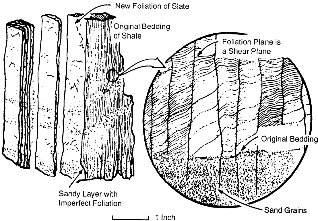
Figure 1-9. Metamorphic foliation.
