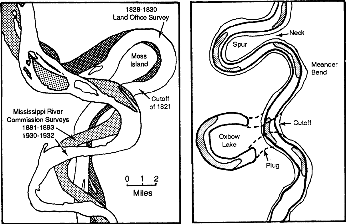
Figure 3-10. Meander development and cutoff.
