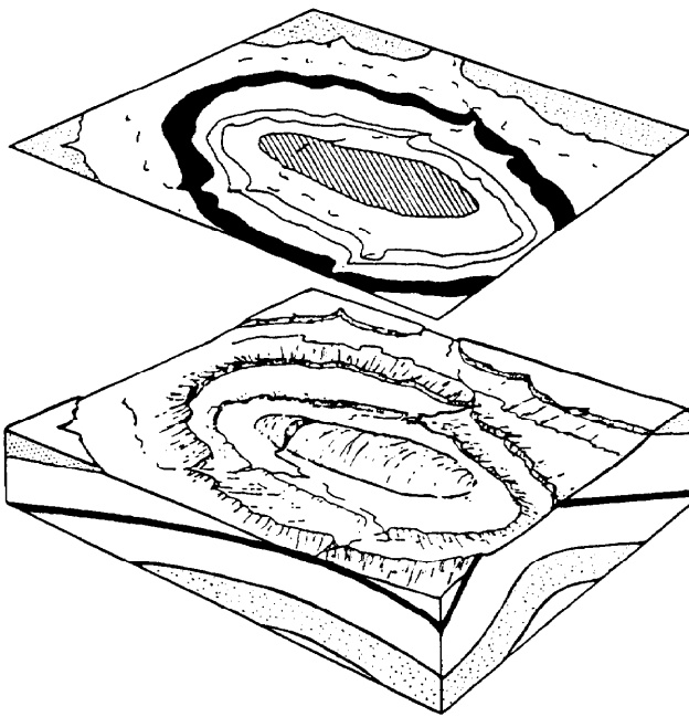
Figure 2-26. Outcrop patterns of an eroded dome.
