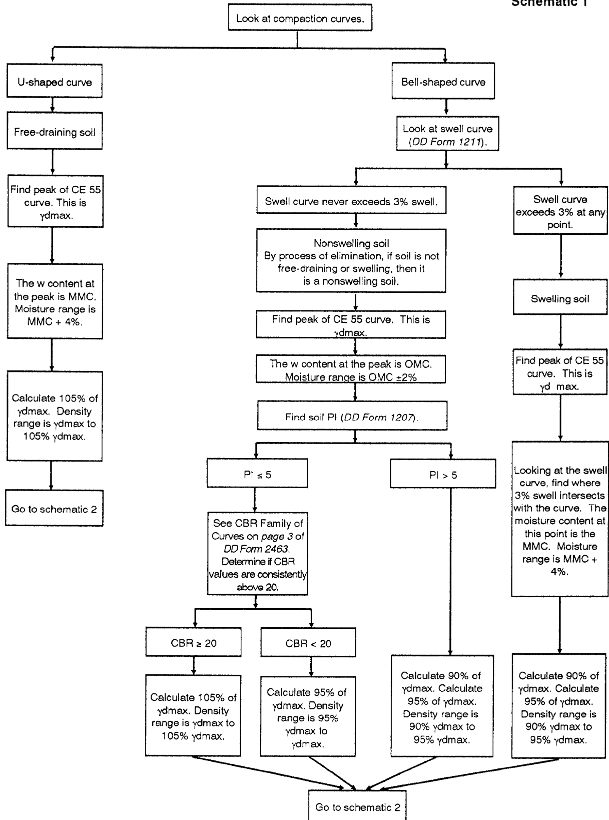
Figure A-1. CBR design flowchart.
