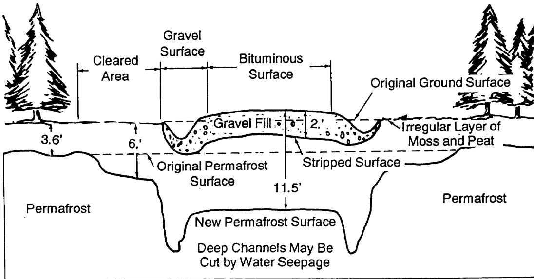
Figure 12-1. Maximum depth to permafrost below a road after 5 years in a subarctic region.
