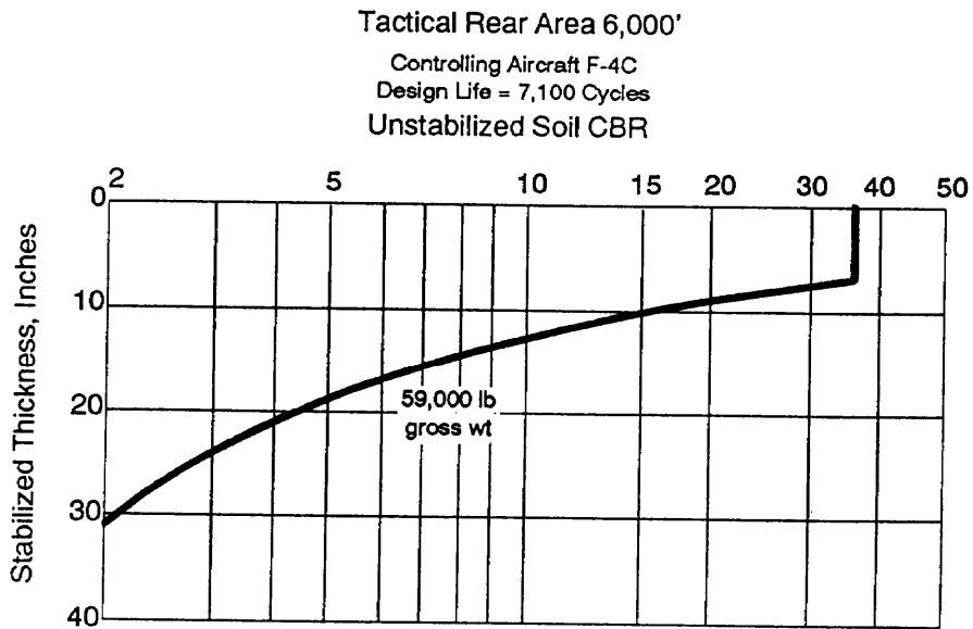
Figure 9-24. Design curves for single-layer airfields using stabilized soils in tactical rear area.
