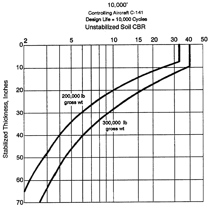
Figure 9-27. Design curves for single-layer airfields using stabilized soils in COMMZ.
