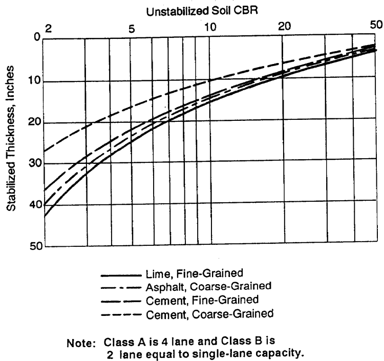
Figure 9-16. Design curve for Class A and Class B multilayer roads using stabilized soils.
