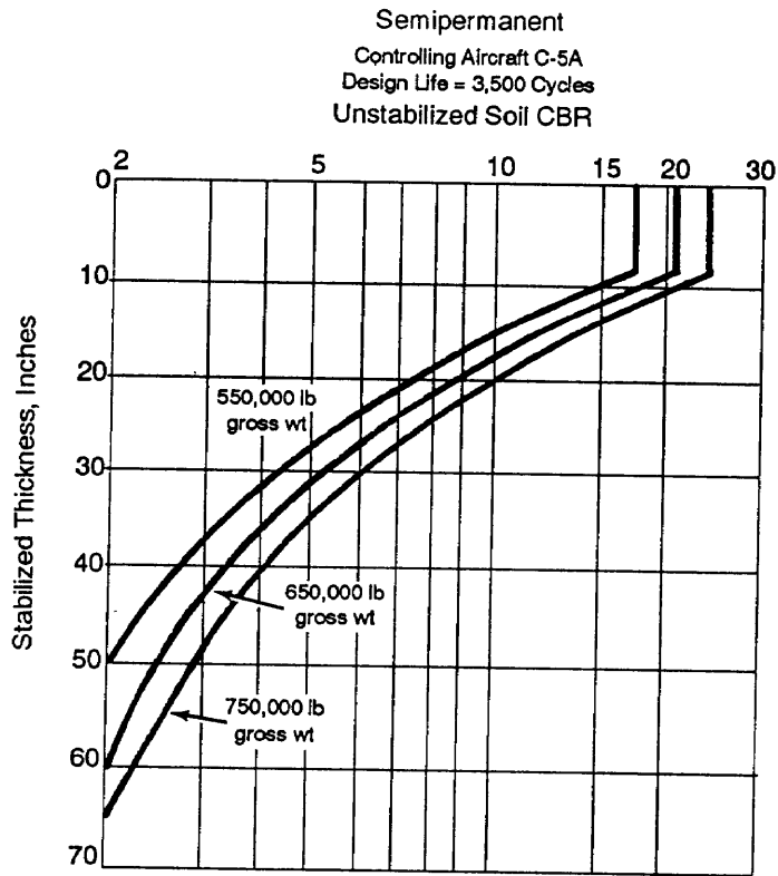
Figure 9-28. Design curves for single-layer airfields using stabilized soils in semi-permanent COMMZ airfields.
