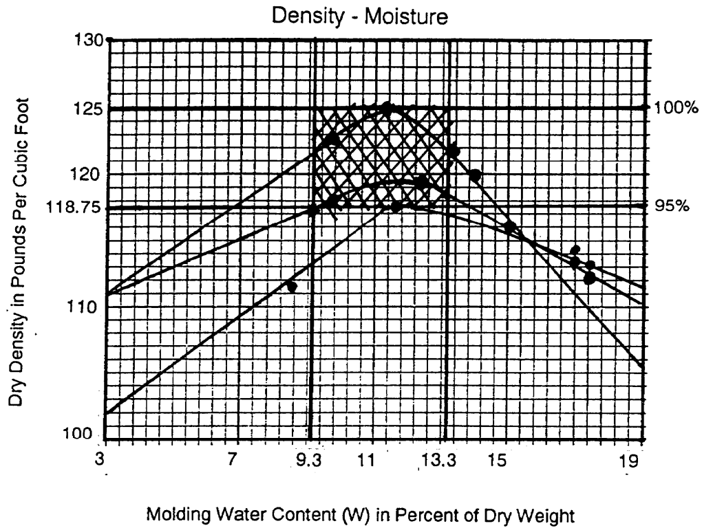
Figure A-7. Density-moisture curve for Rio Meta Plain soil with density and moisture ranges plotted.
