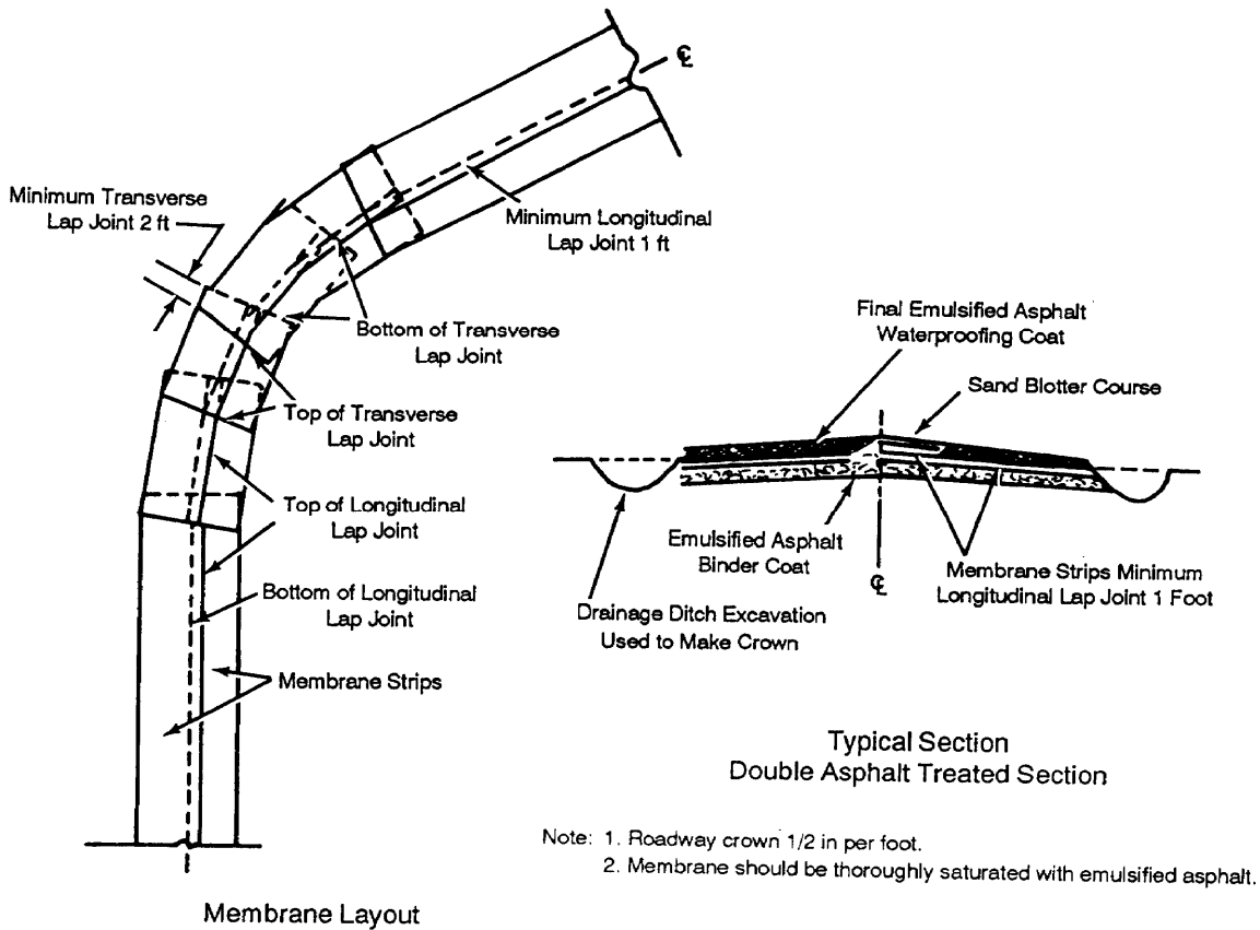
Figure 9-32. Polypropylene membrane layout for curved sections.
