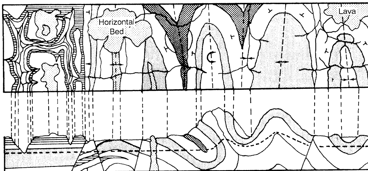
Figure 2-23. Geologic map and cross section.
