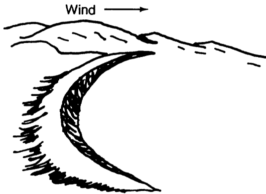
(c) Barchan
