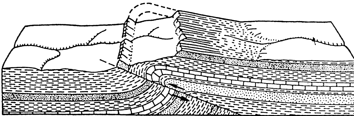
Figure 2-10. Thrust fault with drag folds.
