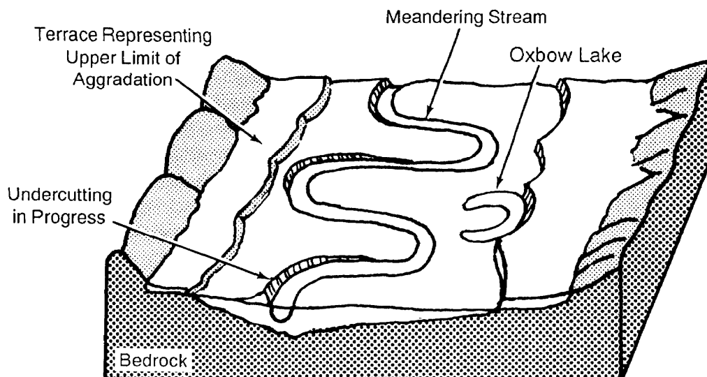
Figure 3-12. Alluvial terraces.
