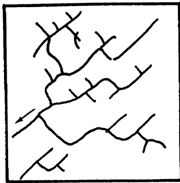
(a) Rectangular
