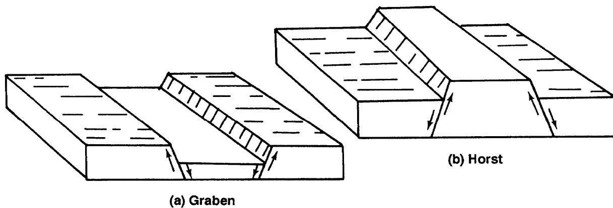
Figure 2-13. Graben and horst faulting.
