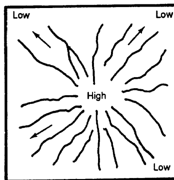
(e) Radial
