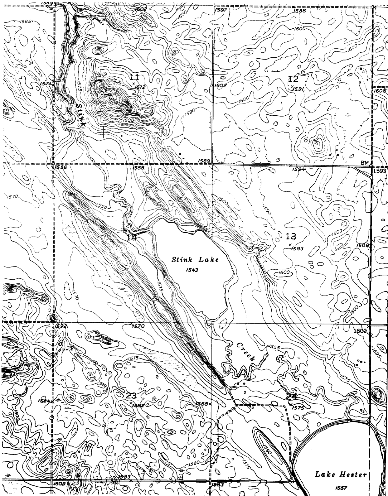
Figure 3-24. Moraine topographic expression with kettle lakes, swamps, and eskers.
