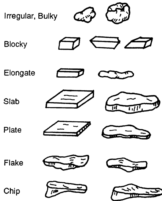
Figure 1-13. Crushed shape.
