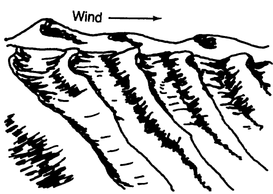
(a) Transverse
