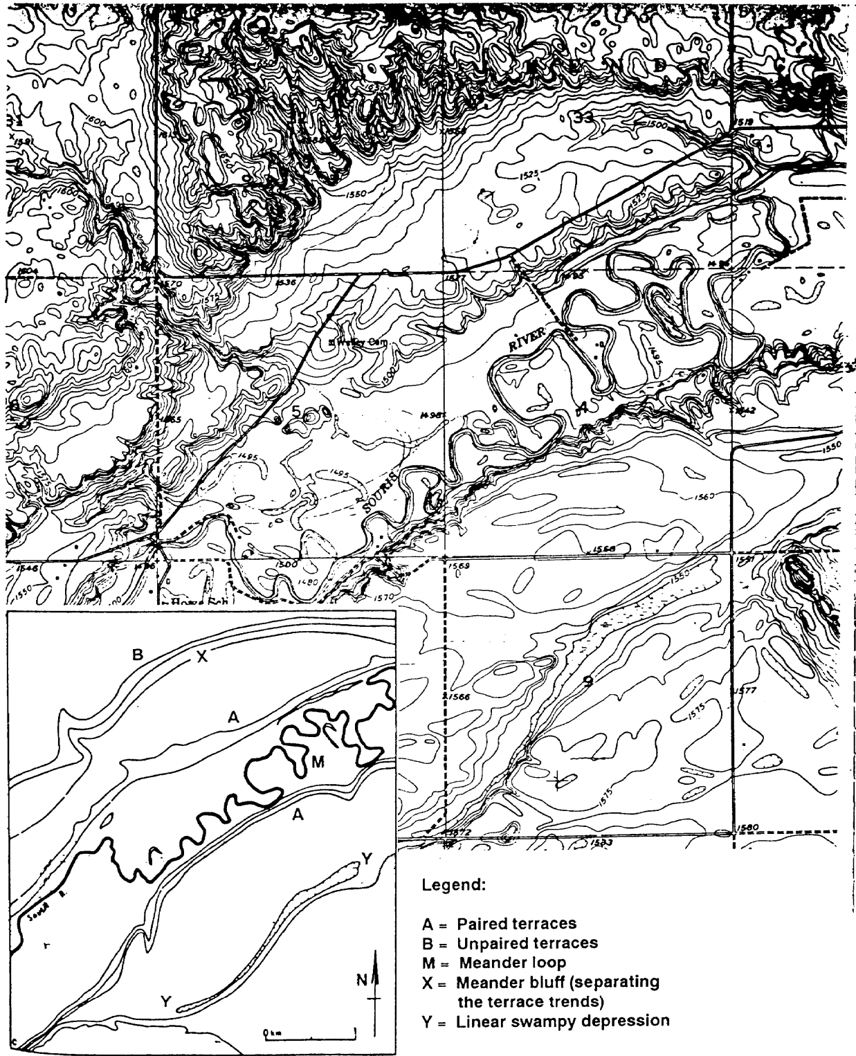
Figure 3-13. Topographic expression of alluvial terraces.
