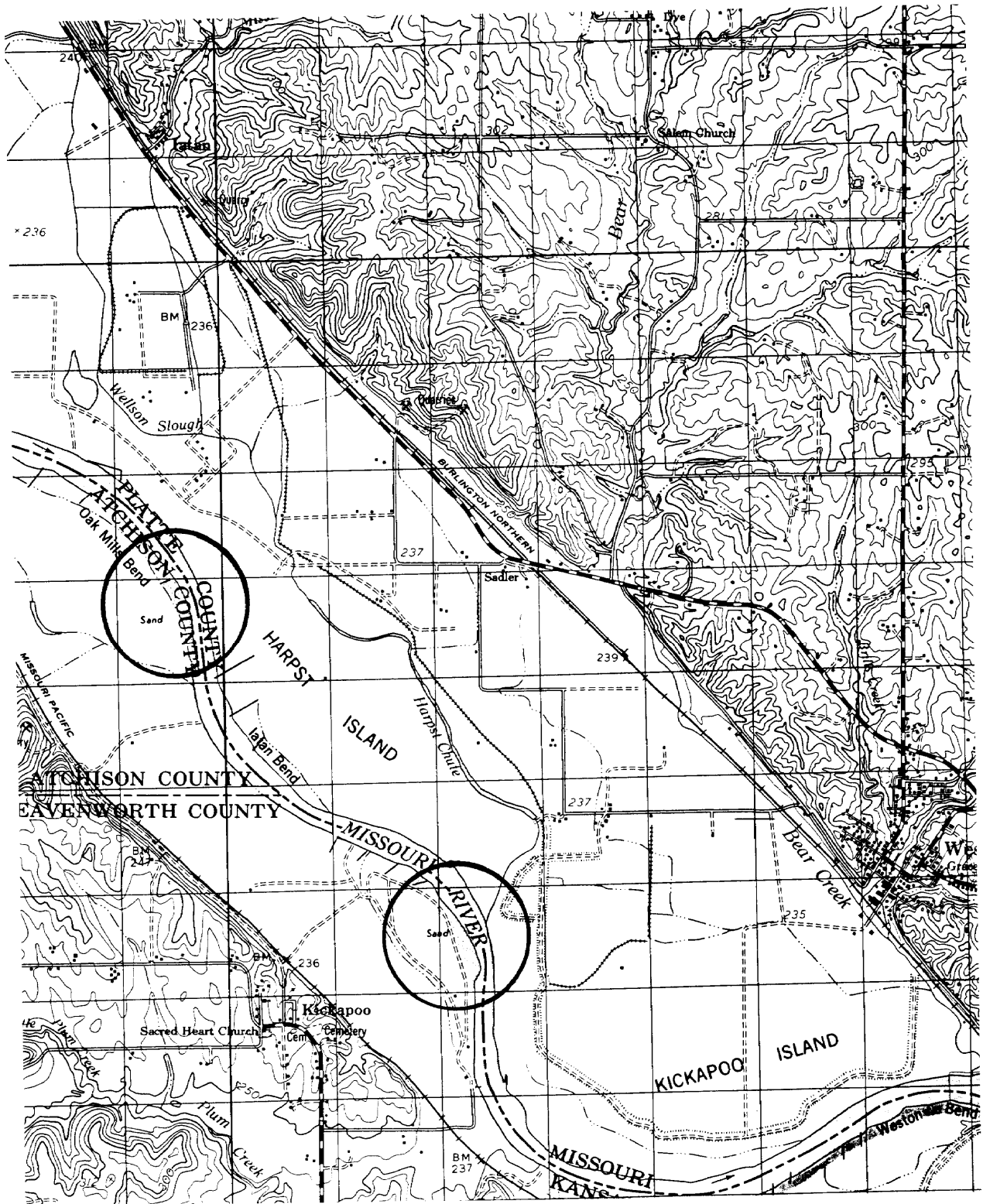
Figure 3-8. Point bar deposits designated by gravel symbols.
