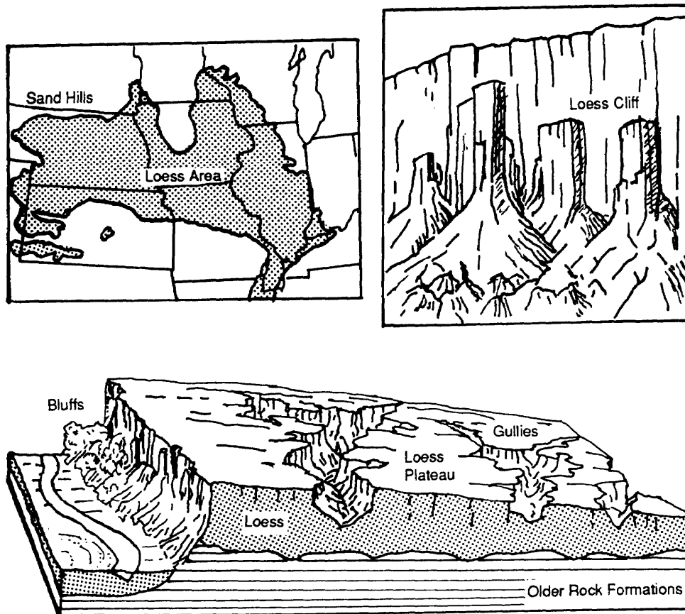
Figure 3-34. Loess landforms.
