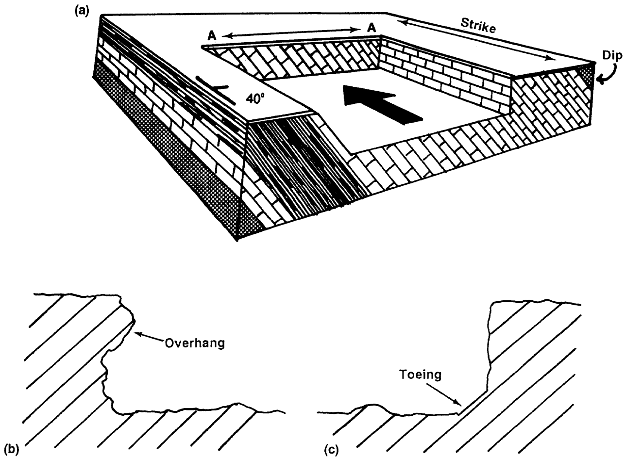
Figure 2-37. Quarry in the direction of strike.
