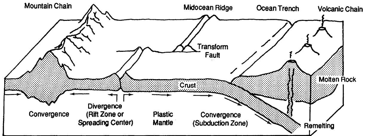
Figure 2-2. Major features of the plate tectonic theory.
