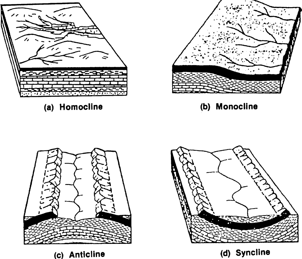
Figure 2-5. Common types of folds.
