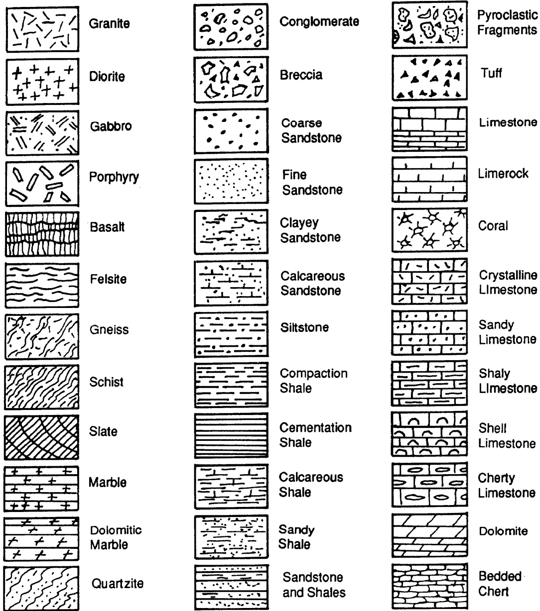
Figure 2-20. Symbolic patterns for rock types.
