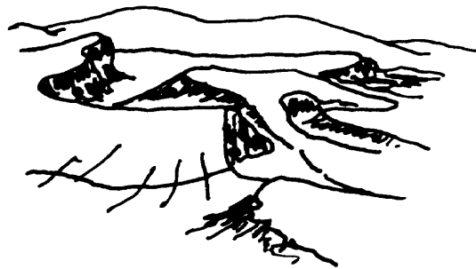
(e) Complex
