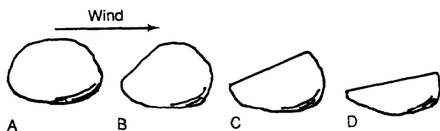
Figure 3-31. Cutting of a ventifact.
