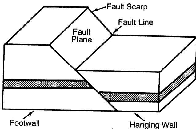
Figure 2-11. Fault terminology.
