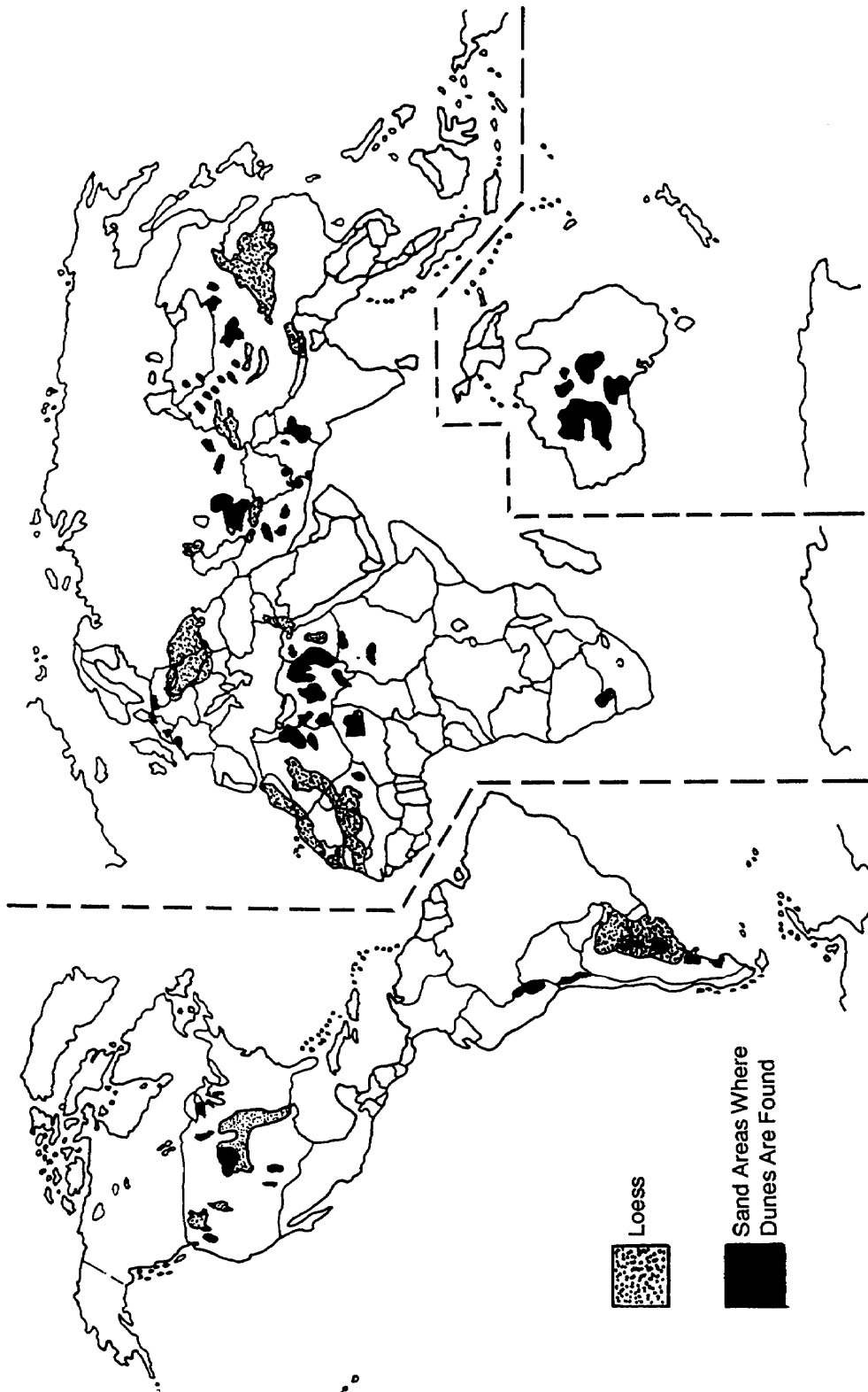
Figure 3-36. Worldwide distribution of eolian landforms.
