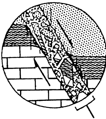
Figure 2-9. Fault zone.
