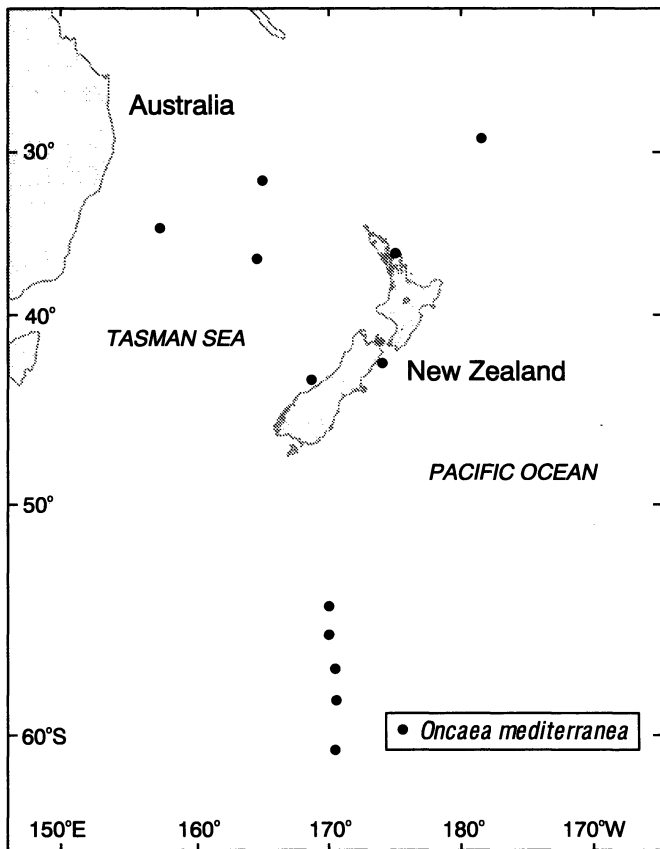
Fig. 26. New records of a, Oncaea furcula and O. inflexa ; b, Oncaea lacinia and O. media ; c, Oncaea mediterranea ; d, Oncaea prolata and O. quadrata , in the Southwest Pacific Ocean.
