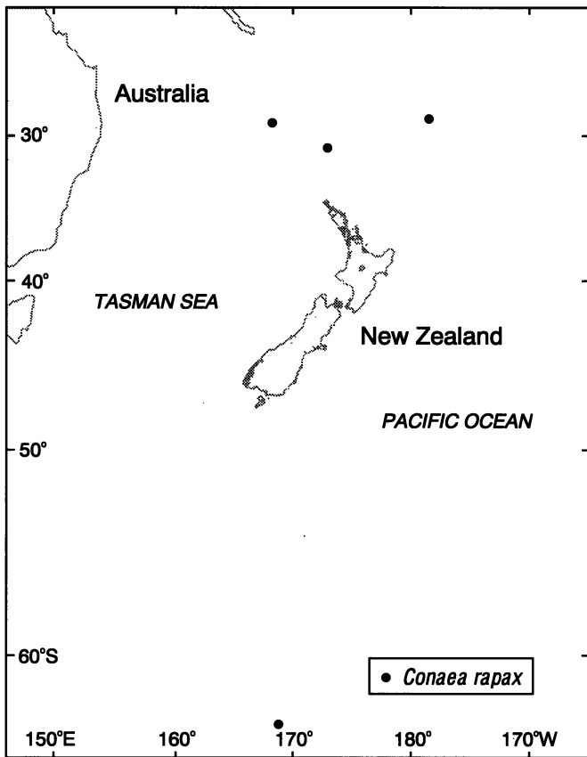
Fig. 27. New records of a, Oncaea redacta and O. scottodicarloi ; b, Oncaea venusta ; c, Conaeta rapax , in the Southwest Pacific Ocean.
