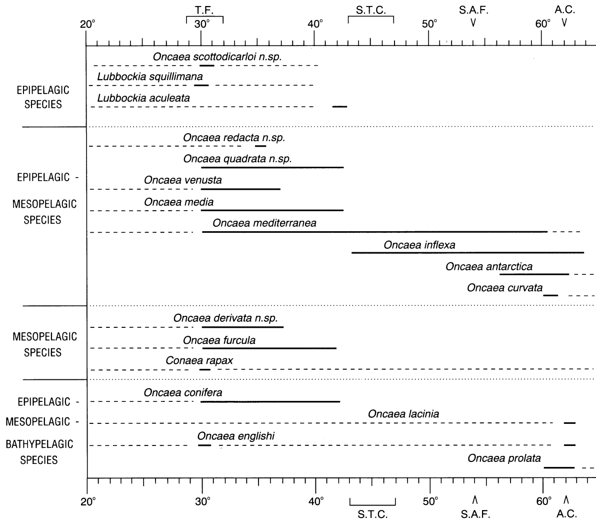
Fig. 28. Distribution of Oncaeidae with depth and latitude: _____ Southwest Pacific records, ---- likely distribution from existing records. S.T.C. = Subtropical Convergence, S.A.F. = Subantarctic Front, A.C. = Antarctic Convergence.
