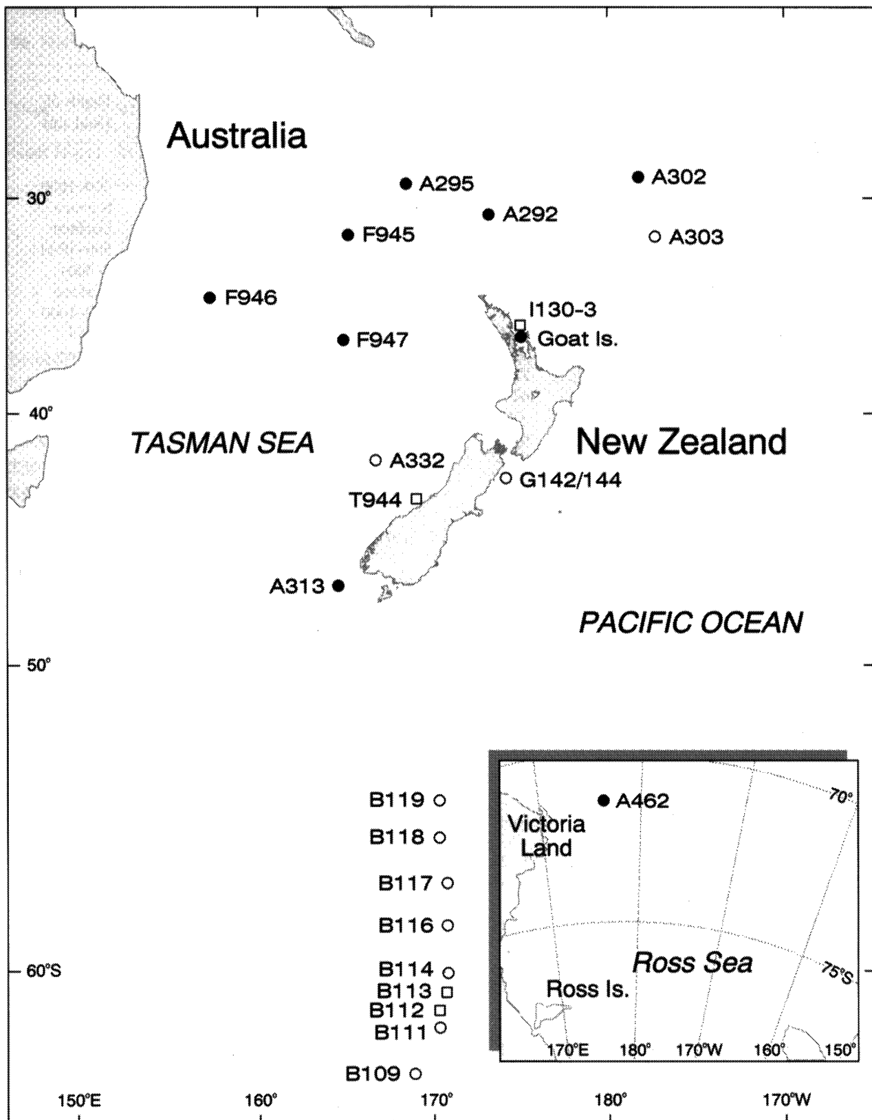
Fig. 1. Map of the Southwest Pacific Ocean (including the Ross Sea) indicating the position of stations from which specimens were collected, with the maximum sampling depth indicated: □ = 0-125 m; ■ = 126-250 m; ○ = 251-500 m; ● = > 500 m.
