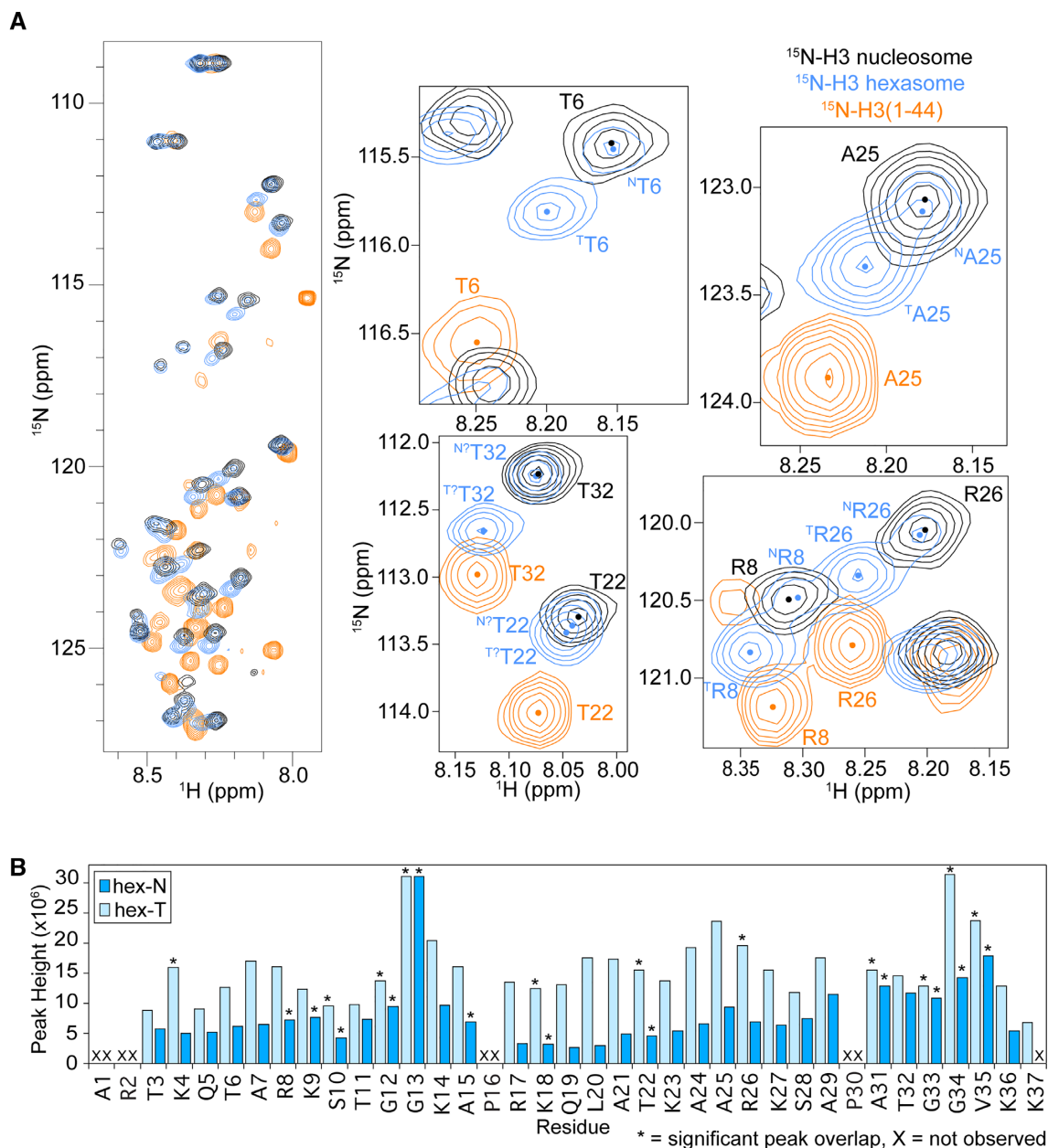
Figure 2. Tetrasomal tail is more dynamic. (A) H3 tail conformation within tetrasome more closely mirrors H3 tail peptide. Overlay of ^1\text{H}/^{15}\text{N} -HSQC/HMPC spectra collected on ^{15}\text{N} -H3 nucleosome (black), ^{15}\text{N} -H3 hexasome (blue), and ^{15}\text{N} -H3(1-44) (orange). Comparison of the spectra shows that, in general, the tetrasomal H3 tail experiences a more similar chemical environment to the H3 tail peptide than does the nucleosomal H3 tail, which suggests a more extended tail ensemble within the tetrasome than the nucleosome. Expanded regions of the overlay are shown for selected residues for closer comparison of histone tail states. Small circles mark the approximate center of each peak to aid in the spectral comparison. These spectra were collected on 44\mu\text{M} ^{15}\text{N} -H3 nucleosome species or 110\mu\text{M} ^{15}\text{N} -H3(1-44) in 20 mM MOPS pH 7, 150 mM KCl, 1 mM EDTA, 1 mM DTT, 7% \text{D}_2\text{O} at 25^\circ\text{C} and on an 800 MHz spectrometer. (B) Peak intensity (height) is plotted as a function of residue for the hex-N (blue) and hex-T (light blue) H3 tails within the hexasome for the spectrum shown in Figure 1A (blue). Residues that are not observed in the spectra are marked with an 'X'. Residues with significant overlap that prevents accurate determination of peak height are marked by '*'.
