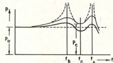
(c) (i) — Target Response of Actual Receiver. (ii) — Target Response of Analogous Electrical Network of Receiver. (iii) — Response (ii) without Damping—this is the Theoretical Response of the Simplified Network of Fig. 7(b).
