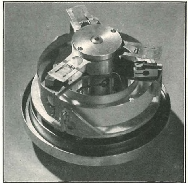
(a) 100 kc/s Z-cut quartz ring mounted on thread suspension, with cover removed.
