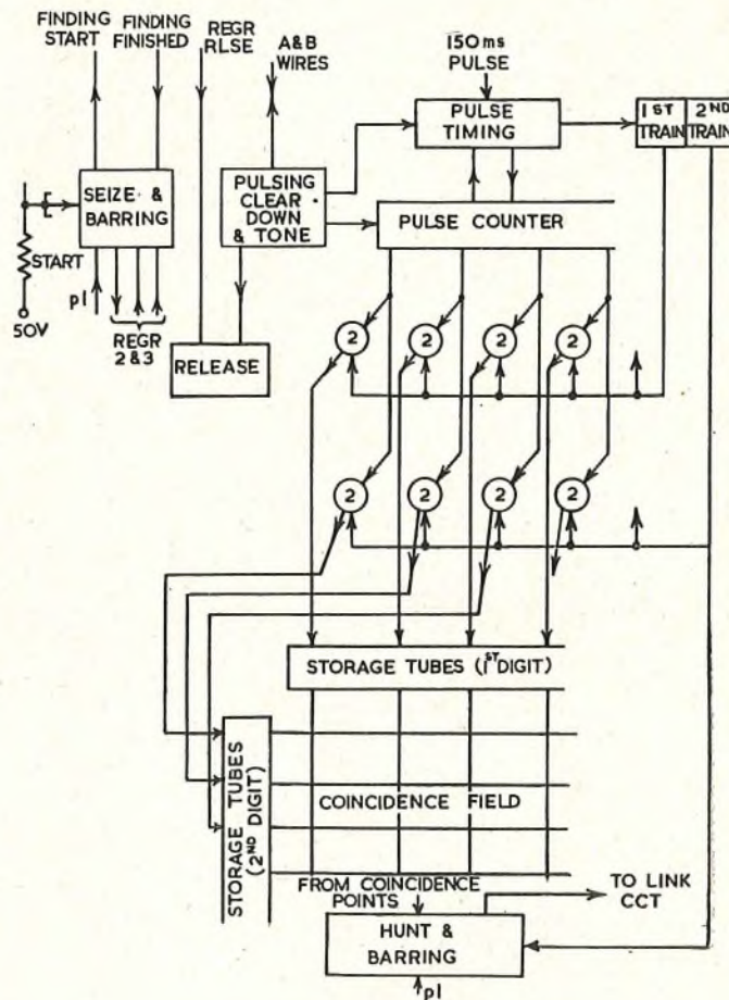
FIG. 2.—BLOCK SCHEMATIC DIAGRAM OF THE REGISTER.
