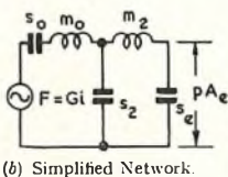
(b) Simplified Network.
