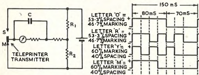
FIG. 4.—BASIC CIRCUIT OF BIAS DISTORTION TESTER.
