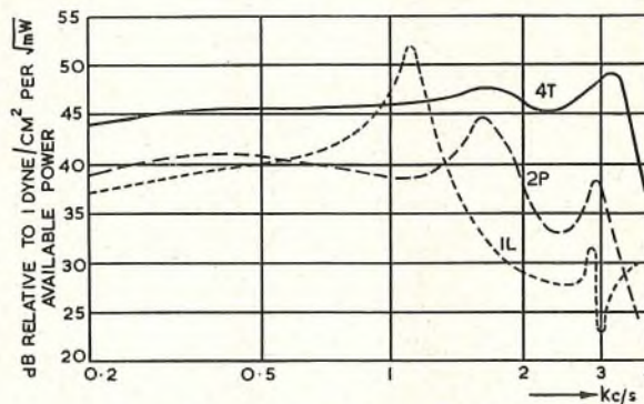
FIG. 9.—SENSITIVITY/FREQUENCY CHARACTERISTICS OF 4T, 2P and 1L RECEIVER INSETS.
