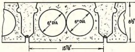
CROSS-SECTION OF ROOF UNIT.
