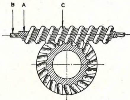
FIG. 3.—FLEXIBLE ROD AND PINION WHEEL.
