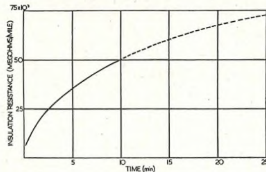
FIG. 19.—INSULATION RESISTANCE OF THE CABLE.
