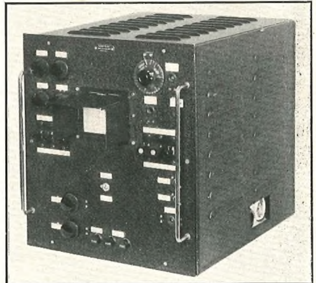
FIG. 2.—ELECTRONIC DISTORTION MEASURING SET.
