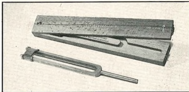
FIG. 1.—TUNING-FORK STROBOSCOPE.
