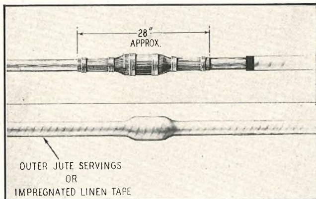
(c) The Completed Splice.
