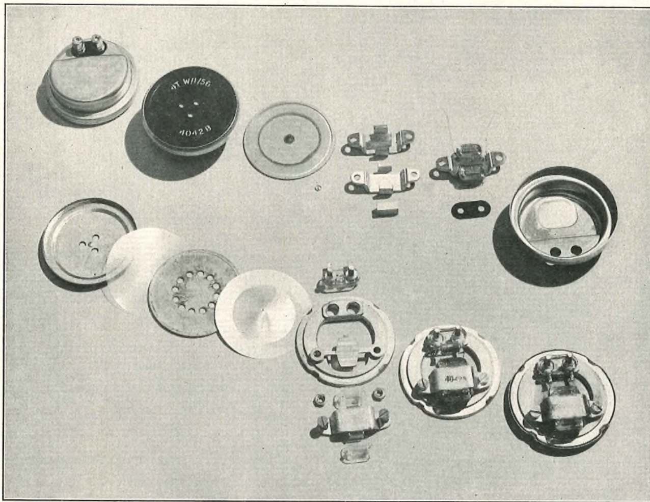
FIG. 8.—THE ROCKING-ARMATURE RECEIVER AND ITS COMPONENT PARTS.
