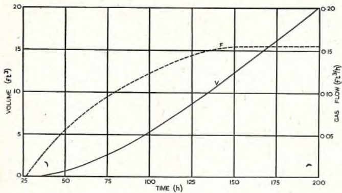
Cable type: 54/044. Length: 4.432 miles. Sending pressure: 10 lb/in 2 . Receiving pressure: atmospheric.
