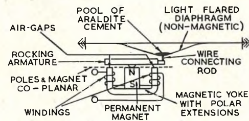
FIG. 2.—BASIC ELEMENTS OF ROCKING-ARMATURE RECEIVER.
