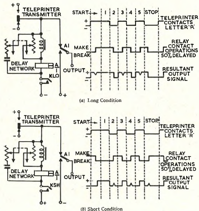
FIG. 5.—BASIC CIRCUIT OF SIGNAL-BIASING UNIT.
