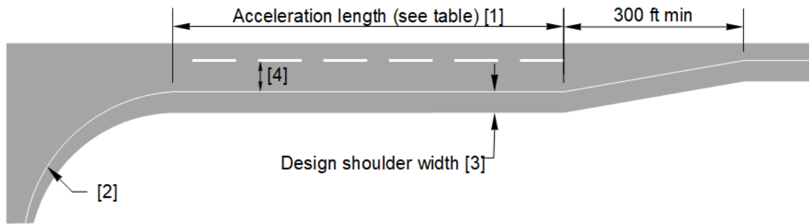
Exhibit 1310-27 Acceleration Lane
