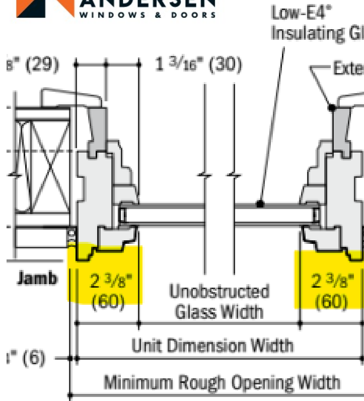
Horizontal Section
