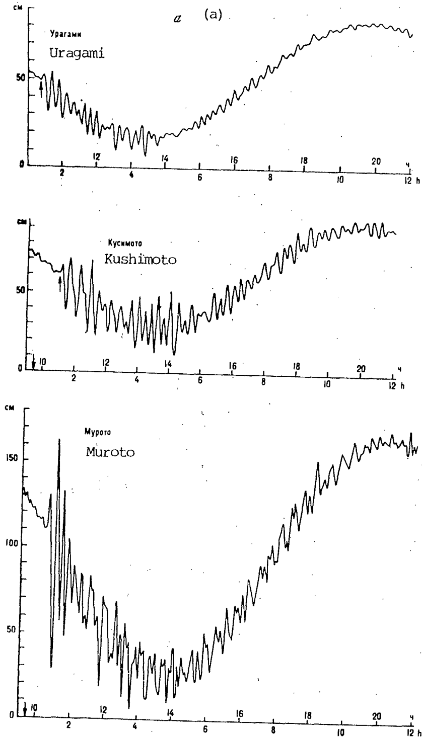
Records of the tsunami of 1.IV.1968 on tide gauges on the Kii Peninsula and the east of Shikoku Island (a), on the west of Shikoku Island (b), and on Kyushu Island (c) (Kajiura et al, 1968a).
