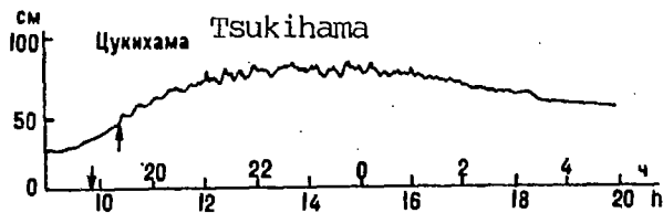
Fig. 29 Records of the tsunami of 27.V.1928 (Iida, 1956).
