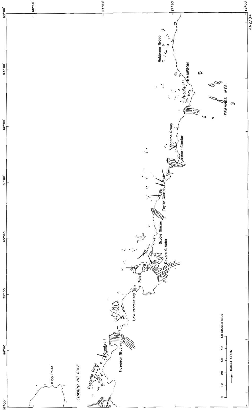
FIG. 1. Locality map of the Mac-Robertson Land and Kemp Land coast—showing raised beaches.
