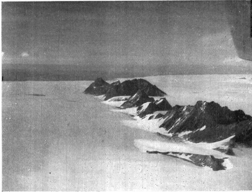
1. Charnockite mountains of the David Range. A small nunatak of Painted Gneiss is in the right foreground.
