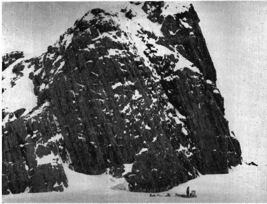
5. Stillwell Gneiss near Fold Island.
