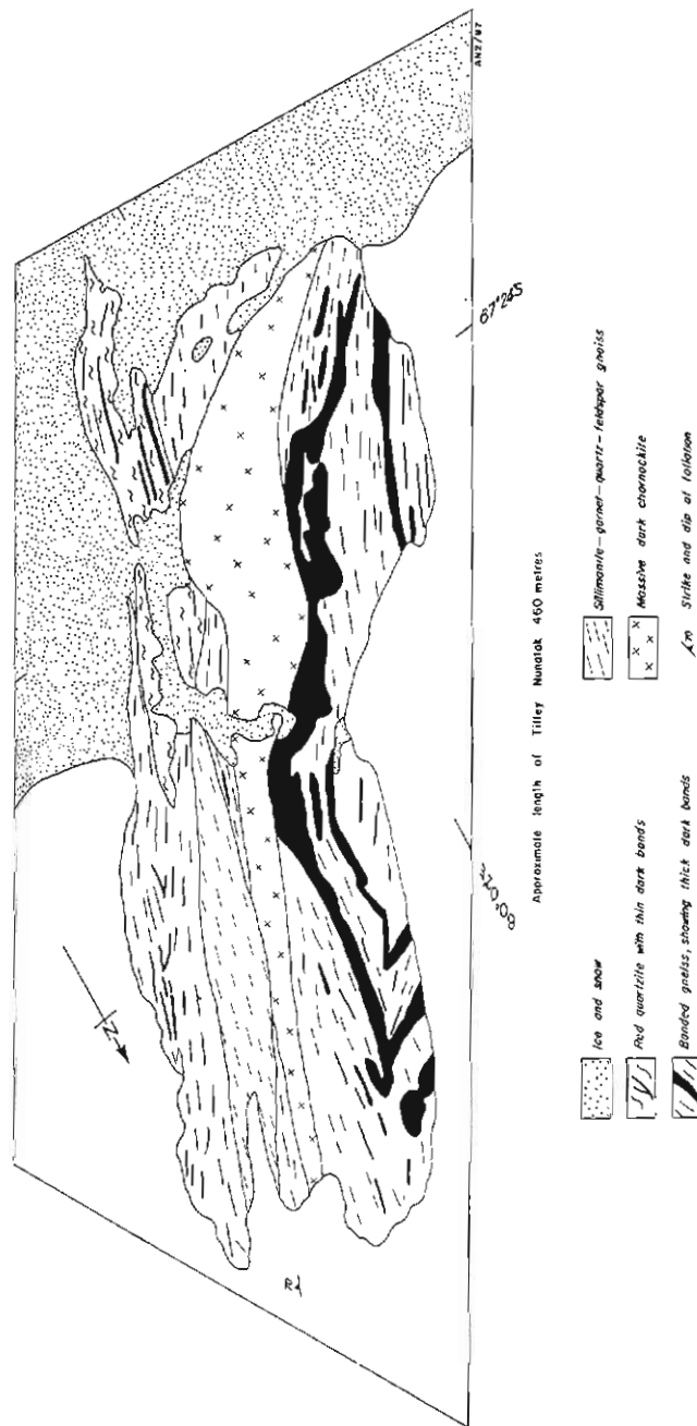
Fig. 4. Geological sketch of Tilley Nunatak (based on oblique air-photographs)
