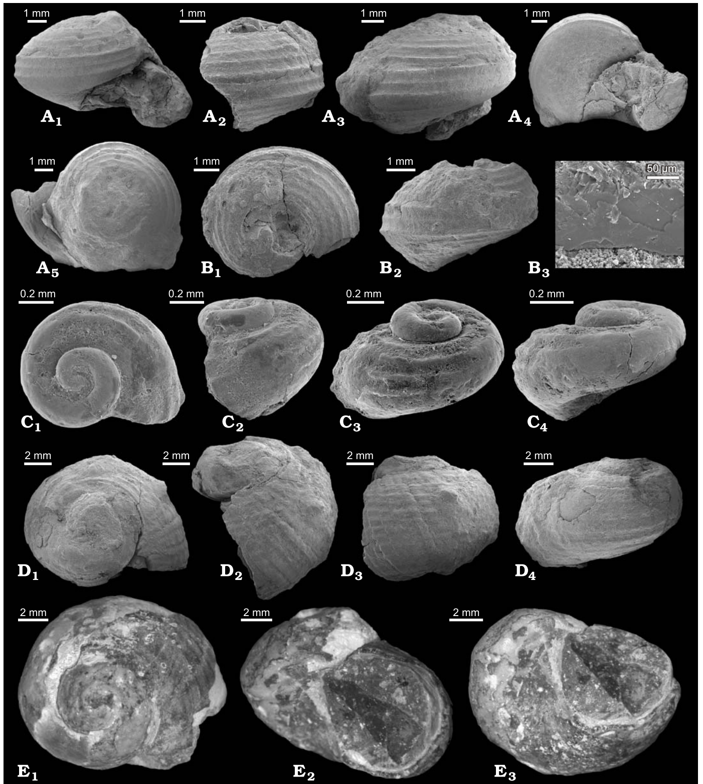
Fig. 8. The trochid gastropod Margarites sasakii sp. nov. from the Campanian (Upper Cretaceous) Omagari seep site in Hokkaido, Japan. A. UMUT MM30171 in apertural (A 1 ) lateral (A 2 , A 3 ), umbilical (A 4 ), and apical (A 5 ) views. B. UMUT MM30172 in apical (B 1 ) and lateral (B 2 ) views; B 3 , cross section through outer layer. C. Juvenile UMUT MM30173 in apical (C 1 ), and lateral (C 2 –C 4 ) views. D. Holotype (UMUT MM30174) in apical (D 1 ) and lateral (D 2 –D 4 ); note change in ornamentation in D 4 . E. NMM 229 in apical (E 1 ), apertural (E 2 ), and umbilical (E 3 ) views.
