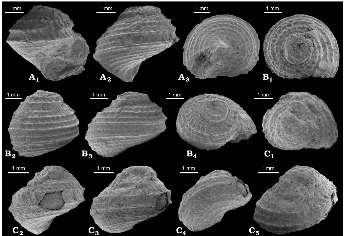
Fig. 9. The seguenzioid gastropod Cataegis nakagawensis sp. nov. from the Campanian (Upper Cretaceous) Omagari seep site in Hokkaido, Japan. A. Holotype (UMUT MM30175) in apertural (A 1 ), lateral (A 2 ), and umbilical (A 3 ) views. B. UMUT MM30176 in apical (B 1 ), lateral (B 2 , B 3 ), and latero-apical (B 4 ) views. C. UMUT MM30177 in apical (C 1 ), lateral (C 2 , C 3 ), latero-umbilical (C 4 ), and latero-apical (C 5 ) views.
