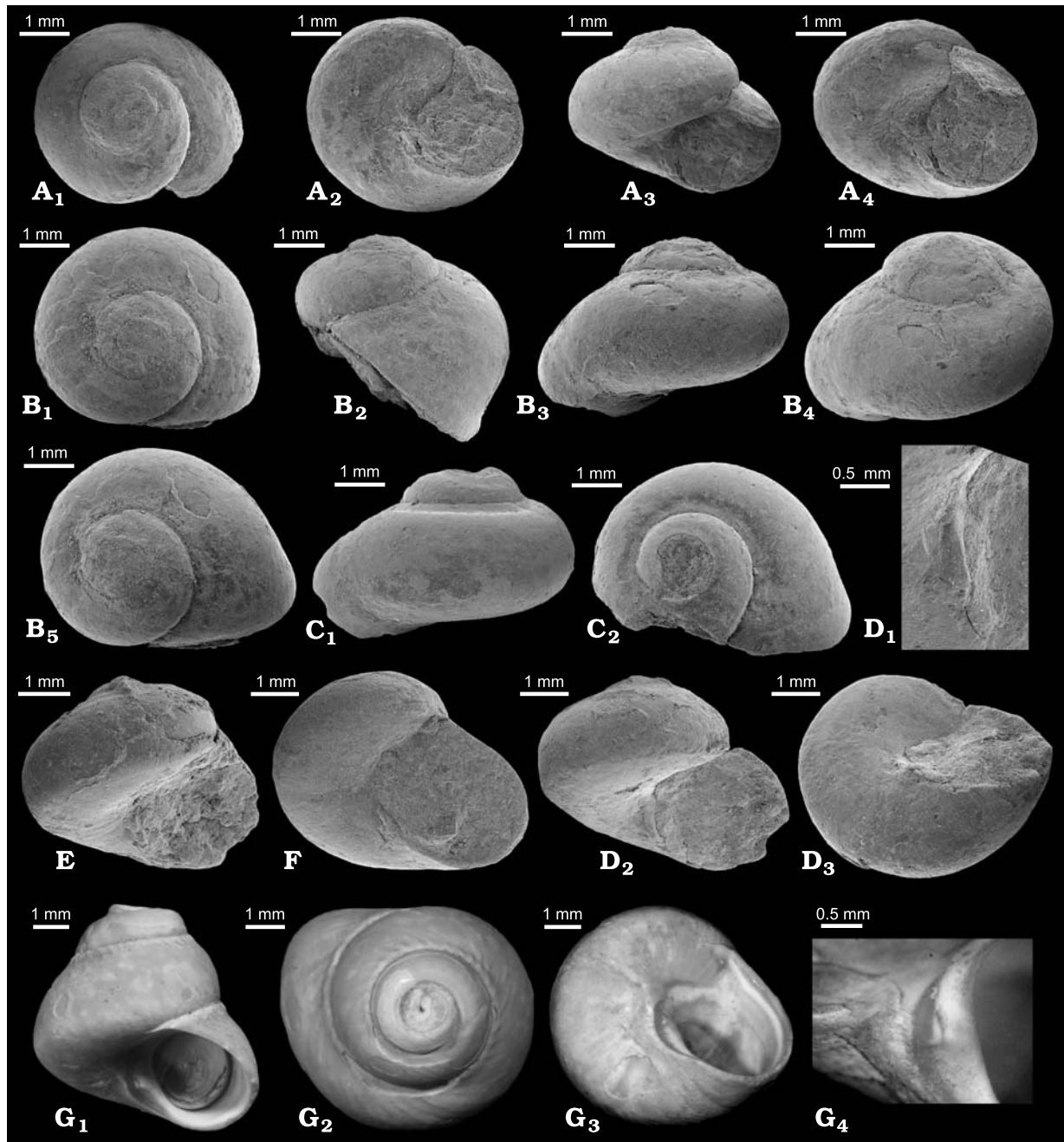
Fig. 7. Turbinid gastropods of the genus Cantrainea from chemosynthesis-based communities. A–F. Cantrainea omagariensis sp. nov. from Campanian (Upper Cretaceous) Omagari seep site in Hokkaido, Japan. A. UMUT MM30165 in apical (A 1 ), umbilical (A 2 ), lateral (A 3 ), and apertural views (A 4 ). B. Holotype (UMUT MM30166) in apical (B 1 , B 5 ), lateral (B 2 , B 3 ), and latero-apical (B 4 ) views. C. UMUT MM30167 in lateral (C 1 ) and apical (C 2 ) views. D. UMUT MM30168; details of inner lip (D 1 ), apertural (D 2 ) and umbilical (D 3 ) views. E. UMUT MM30169 in lateral view. F. UMUT MM30170 in apical view. G. Recent Cantrainea nuda Okutani, 2001 from “depression B” of the Minami Ensei Knoll, Okinawa Trough, Japan (NSMT-Mo 73040) in lateral (G 1 ), apical (G 2 ), and umbilical (G 3 ) views; G 4 , details of inner lip.
