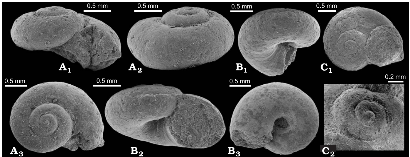
Fig. 14. Skeneimorph gastropod from the Campanian (Upper Cretaceous) Omagari seep site in Hokkaido, Japan. A. UMUT MM30193 in apertural (A 1 ), lateral (A 2 ), and apical (A 3 ) views. B. UMUT MM30194 in lateral (B 1 ), apertural (B 2 ), and umbilical (B 3 ) views. C. UMUT MM30195 in apical view (C 1 ) and close up of initial whorls (C 2 ).
