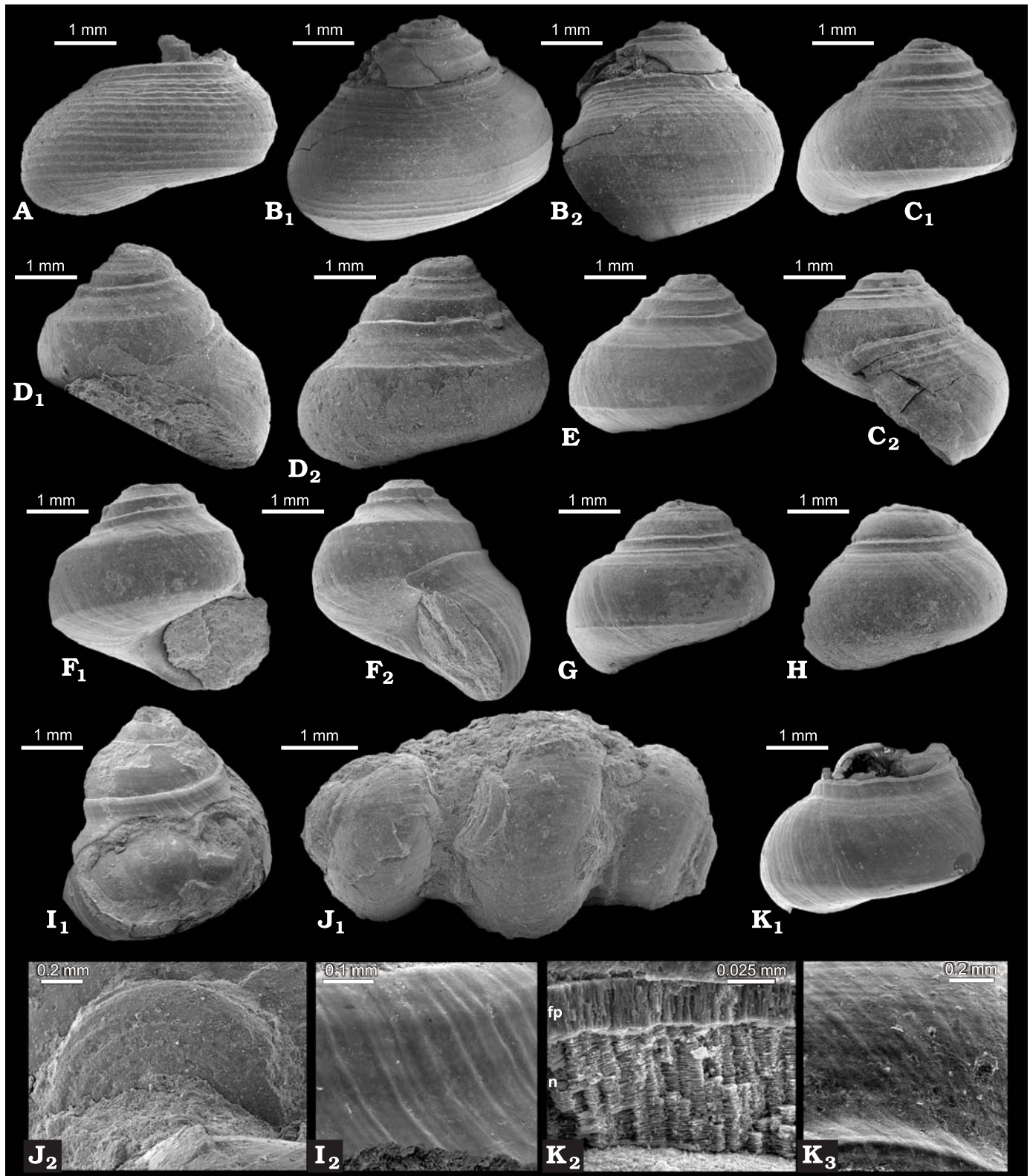
Fig. 5. The turbinid gastropod Cantrainea yasukawensis sp. nov. from the Campanian (Upper Cretaceous) Yasukawa seep site in Hokkaido, Japan. A. UMUT MM30153 in lateral view. B. UMUT MM30154 in lateral view (B 1 ) and another view (B 2 ) showing inclination of the aperture. C. UMUT MM30155 in lateral view (C 1 ) and another view (C 2 ) showing inclination of the aperture. D. UMUT MM30156 in lateral view (D 2 ) and another view (D 1 ) showing inclination of the aperture. E. UMUT MM30157 in lateral view. F. Holotype (UMUT MM30158) in apertural (F 1 ) and lateral (F 2 ) views. G. UMUT MM30159 in lateral view. H. UMUT MM30160 in lateral view. I. UMUT MM30161 in lateral view (I 1 ) and details of ornamentation (I 2 ). J. UMUT MM30162, aggregation of three specimens and an operculum; J 1 , general view; J 2 , the operculum. K. UMUT MM30163 in lateral view (K 1 ), shell microstructure (K 2 ) including the inner nacreous (n) and fibrous prismatic (fp) layers, and details of shell ornamentation (K 3 ).
