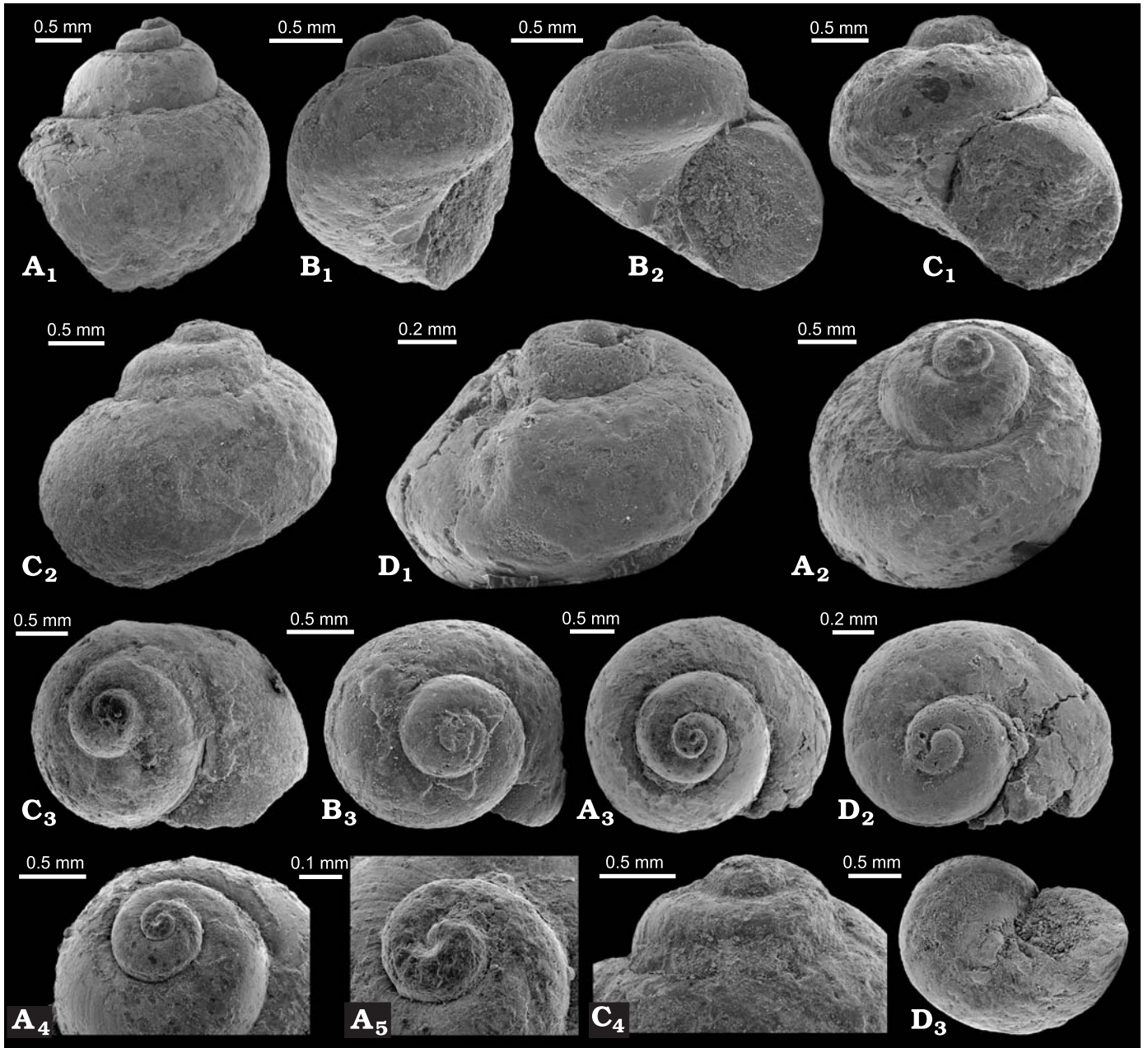
Fig. 13. Naticiform gastropod from the Campanian (Upper Cretaceous) Omagari seep site in Hokkaido, Japan. A. UMUT MM30189 in lateral (A 1 ), latero-apical (A 2 ), and apical (A 3 ) views; A 4 , close up of the juvenile whorls, A 5 , close up of the initial whorl. B. UMUT MM30190 in lateral (B 1 ), apertural (B 2 ), and apical (B 3 ) views. C. UMUT MM30191 in apertural (C 1 ), lateral (C 2 ), and apical (C 3 ) views; C 4 , close up of the juvenile whorls in lateral view. D. UMUT MM30192 in lateral (D 1 ), apical (D 2 ), and umbilical (D 3 ) views.
