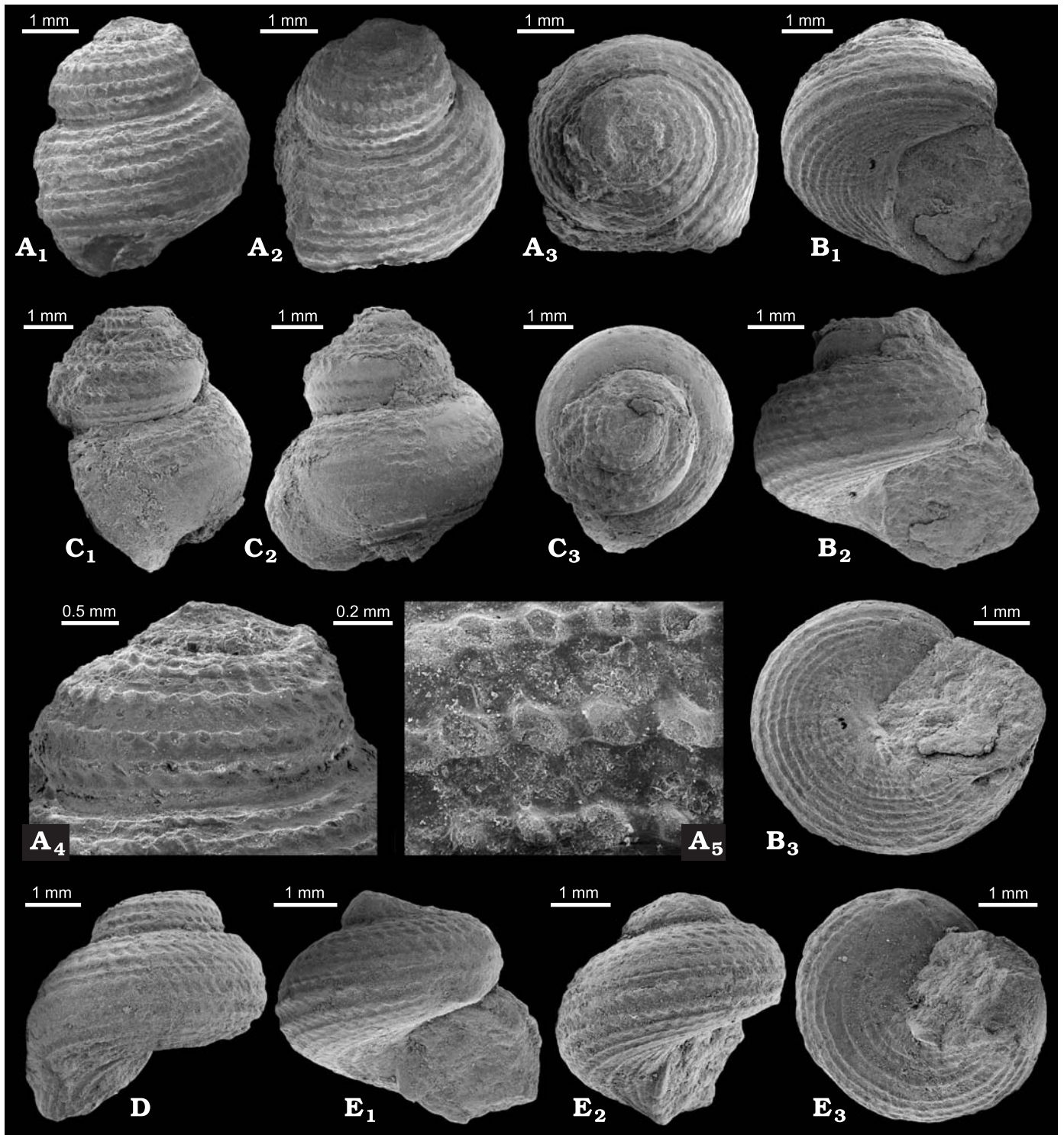
Fig. 4. The turbinid gastropod Homalopoma abeshinaiensis sp. nov. from the Campanian (Upper Cretaceous) Omagari seep site in Hokkaido, Japan. A. UMUT MM30148 in lateral (A 1 ), latero-apical (A 2 ), and apical (A 3 ) views; A 4 , juvenile whorl; A 5 , details of shell ornamentation. B. UMUT MM30149 in apertural (B 1 ), lateral (B 2 ), and umbilical (B 3 ) views. C. Holotype (UMUT MM30150) in lateral (C 1 , C 2 ) and apical (C 3 ) views. D. UMUT MM30151 in lateral view. E. UMUT MM30152 in apertural (E 1 ), lateral (E 2 ), and umbilical (E 3 ) views.
