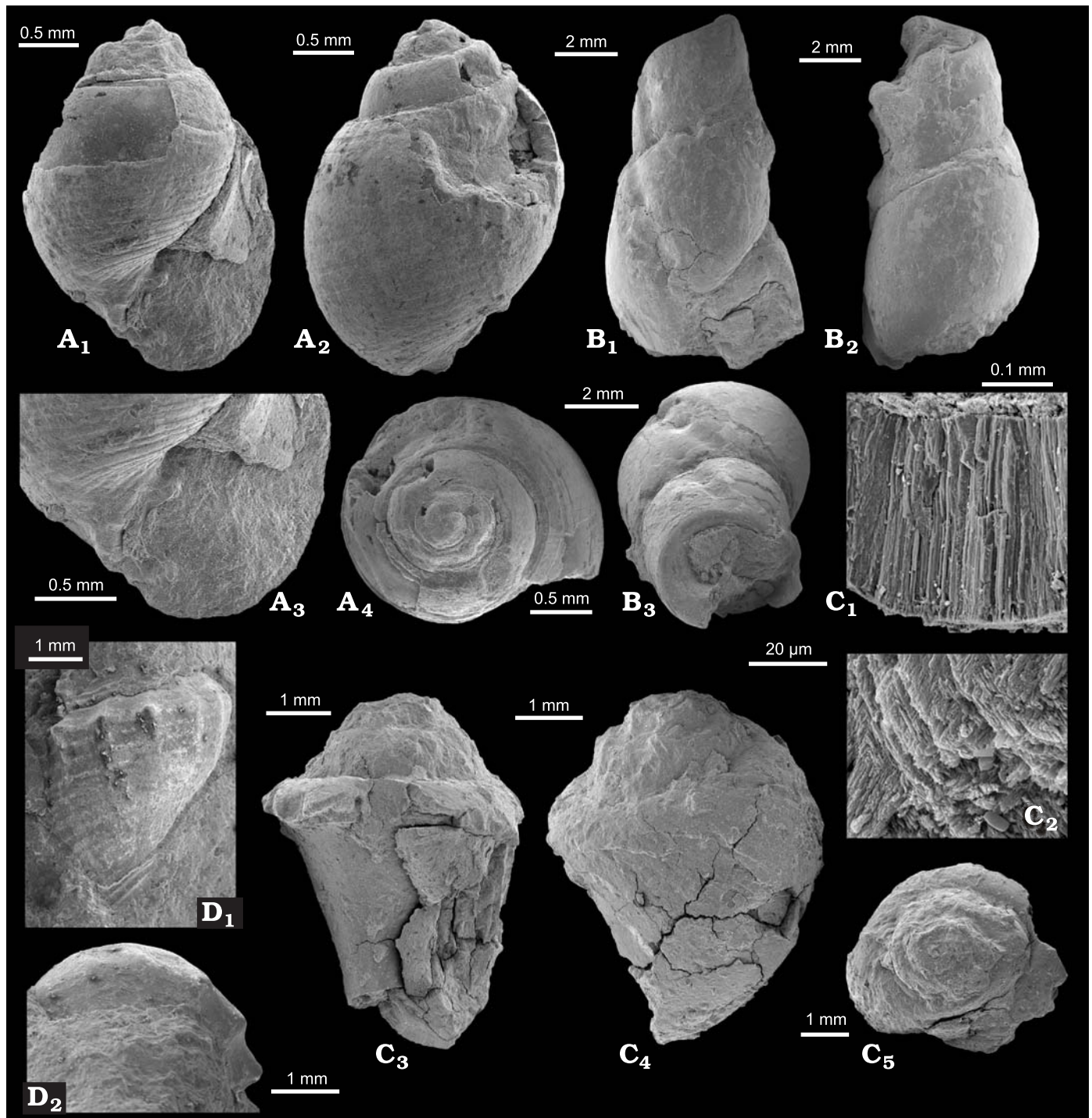
Fig. 12. Gastropods from the Campanian (Upper Cretaceous) Omagari (B) and Yasukawa (A, C, D) seep sites in Hokkaido, Japan. A. ?Sulcoactaeon sp. (UMUT MM30185) in apertural (A 1 ), lateral (A 2 ), and apical (A 4 ) views; A 3 , close up of the aperture. B. Gastropoda indet. 1 (UMUT MM30186) in apertural (B 1 ), lateral (B 2 ), and apical (B 3 ) views. C. Gastropoda indet. 2 (UMUT MM30187) in apertural (C 3 ), lateral (C 4 ), and apical (C 5 ) views; C 1 , fibrous prismatic shell outer layer, C 2 , cross lamellar inner layer. D. Neogastropoda indet. (UMUT MM30188) in lateral (D 1 ) and apical (D 2 ) views.
