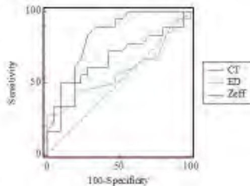
ROC curves
