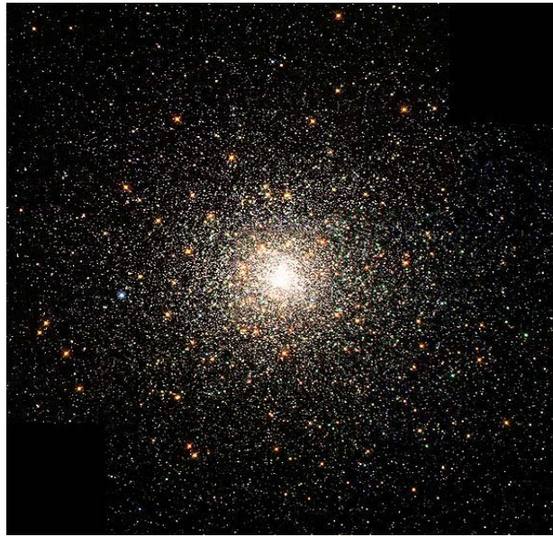
Stars in M80 are mostly old, metal poor members of Population II.
