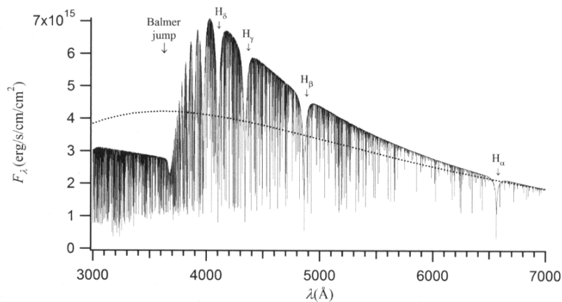
Figure 1.8 Theoretical monochromatic flux emerging from an A type star with T_{\text{eff}} = 8000\text{K} . The first four Balmer absorption lines, as well as the Balmer jump, are identified in this figure. Thousands of other absorption atomic lines can also be seen. This theoretical flux was obtained with the Phoenix stellar atmosphere code (Hauschildt, P.H., Allard, F. and Baron, E., The Astrophysical Journal , 512, 377 (1999)) while using the elemental abundances found in the Sun. The flux at the surface of a blackbody with T = 8000\text{K} (dotted curve) is also shown.
