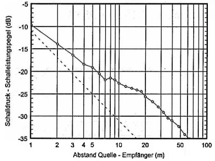
Fig. 7.12 Room PL - 1000 Hz - Dif = 8.0 dB
