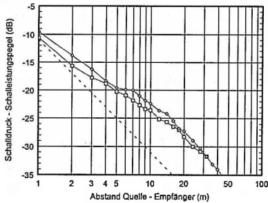
Fig. 6.9 Sound decay curve in hall 2
