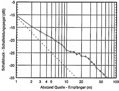
Fig. 7.11 Room PL - 500 Hz - Dif = 7.5 dB
