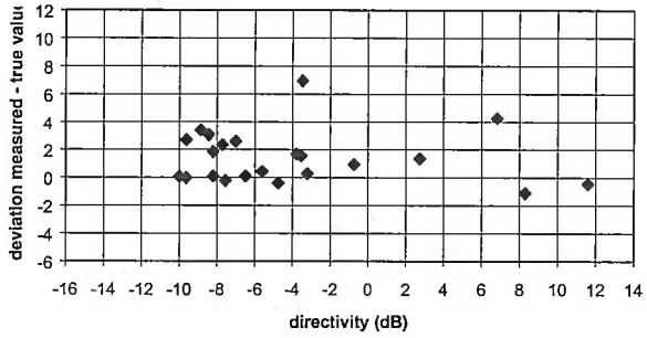
Fig. 6.15 Evaluation on measuring path according to ISO 11204, hall 3, A-weighted level, radiation directional
