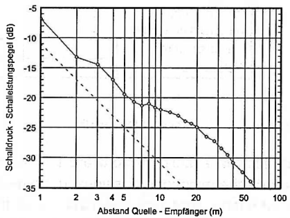
Fig. 7.14 Room PL - 4000 Hz - Dif = 8.4 dB
