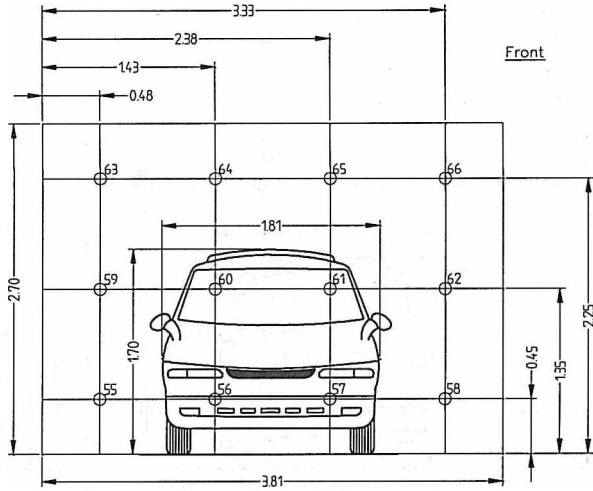
Fig. 6.4 Front view with measuring points 55 to 66
