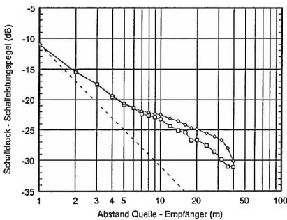
Fig. 7.7 Room DO - Dif = 7.0 dB - DL2 = 2.8 dB (length) Dif = 7.7 dB - DL2 = 1.9 dB (breadth)
