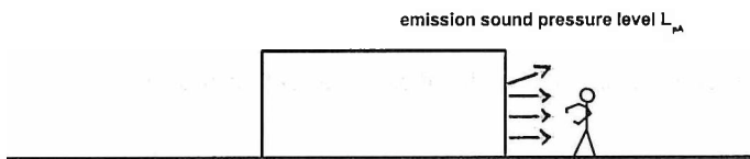
Fig. 2.5 Sound pressure level at the workplace with machine in free field
