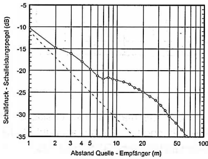
Fig. 7.13 Room PL - 2000 Hz - Dif = 8.0 dB
