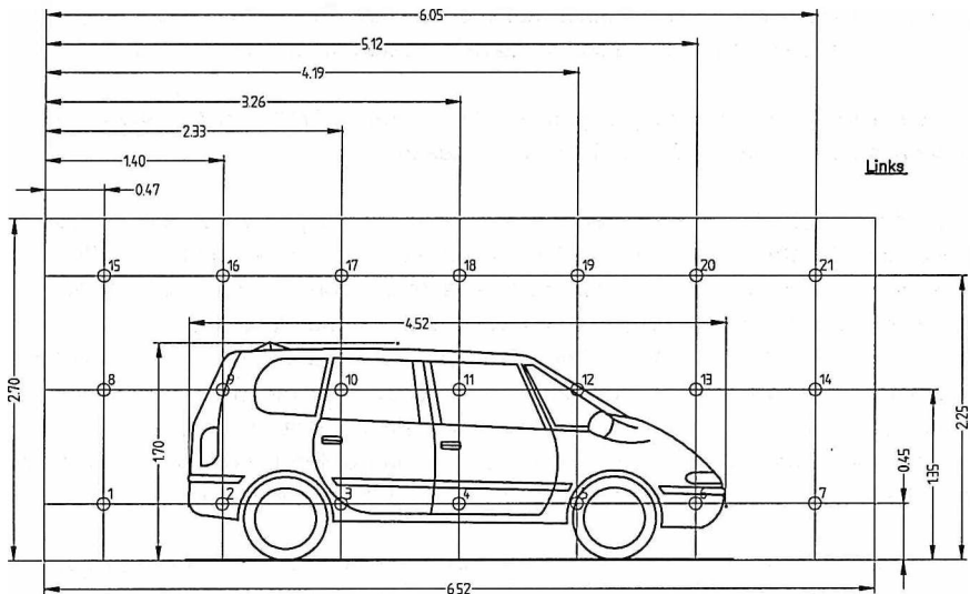
Fig. 6.1 Right side view with measuring points 1 to 21
