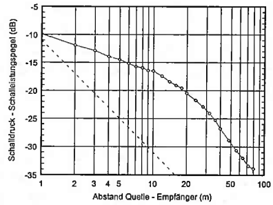
Fig. 6.12 Sound decay curve in hall 5
