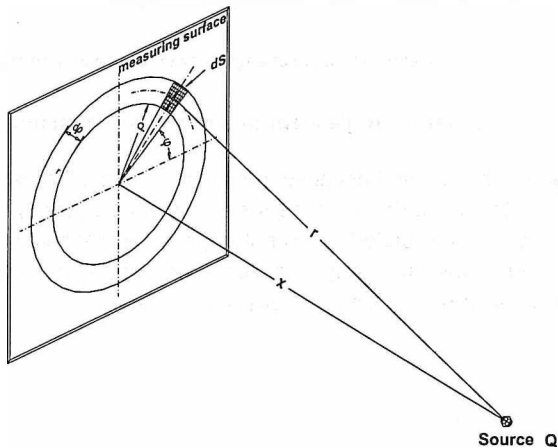
Fig. 5.5 Determination of the sound power transmitted through the measuring surface by measurement of p^2
