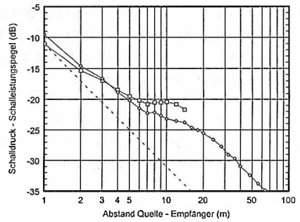
Fig. 7.4 Room PL - Dif = 7.4 dB - DL2 = 2.3 dB
