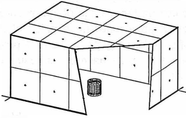
Fig. 5.6 reference sound source in measuring surface
