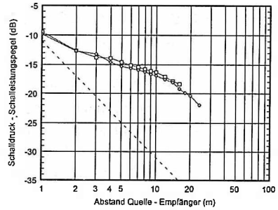
Fig. 6.11 Sound decay curve in hall 4
