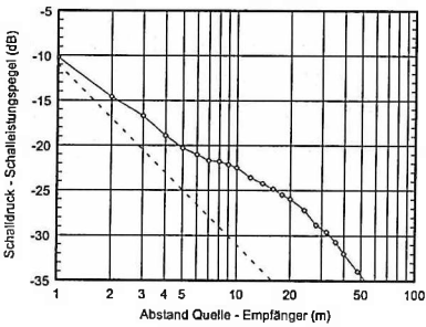
Fig. 6.10 Sound decay curve in hall 3
