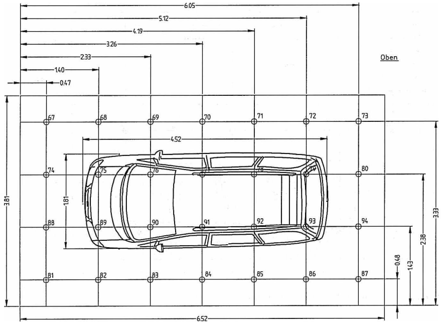
Fig. 6.5 Top view with measuring points 67 to 94
