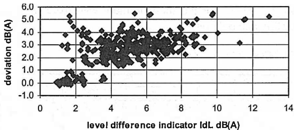
Fig. 7.18 Omnidirectional radiation, all microphone positions, RSS 1 - 4, all rooms
