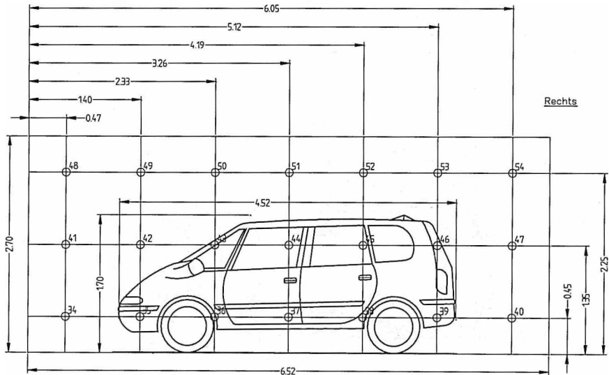
Fig. 6.3 Left side view with measuring points 34 to 54
