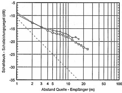
Fig. 7.3 Room PK - Dif = 11.7 dB - DL2 = 2.7 dB
