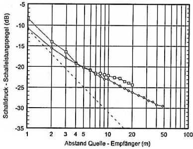
Fig. 6.8 Sound decay curve in hall 1
