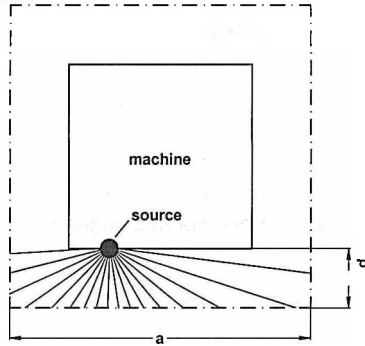
Fig. 5.4: Sound rays emanating from a source on the machine surface
