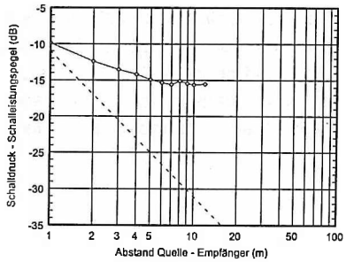
Fig. 6.13 Sound decay curve in hall 6
