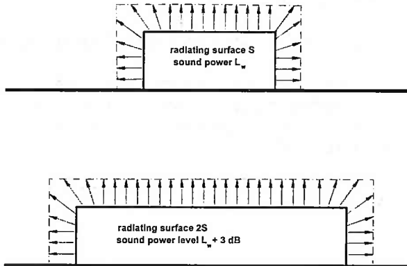
Fig. 2.2 The sound power level is increasing corresponding to the size of the machine
