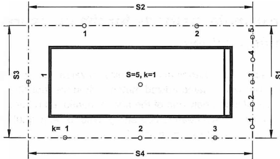
Fig. 4.1 arrangement of measurement points with different density
