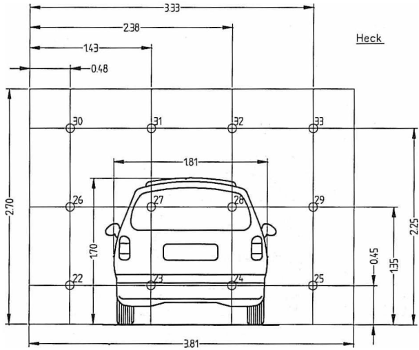
Fig. 6.2 Rear view with measuring points 22 to 33
