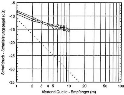
Fig. 7.5 Room RH - Dif = 13.7 dB - DL2 = 1.0 dB
