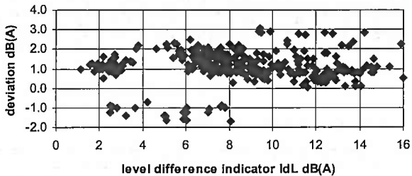
Fig. 7.19 Radiation directional, all microphone positions, RSS 1 - 4, all rooms
