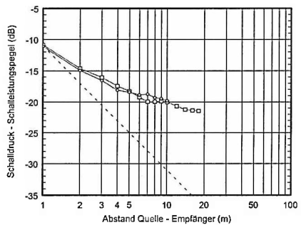
Fig. 7.8 Room GU - Dif = 10.0 dB - DL2 = 1.6 dB
