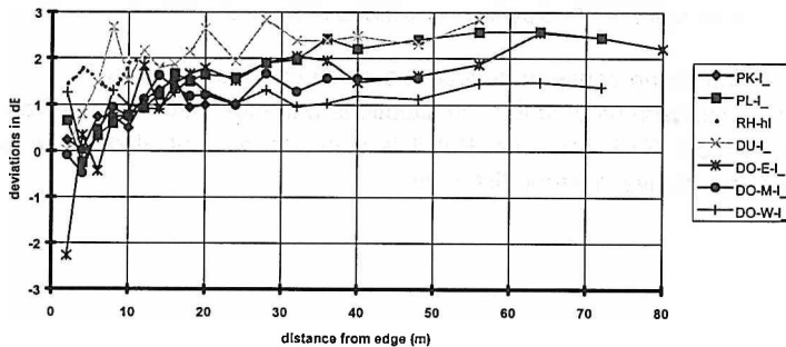
Fig. 7.16 Deviations with measuring at single points - path radial to radiating area - RSS position d6 Hall GU is not included in this evaluation, because in this hall no path is leading away from the radiating area.
