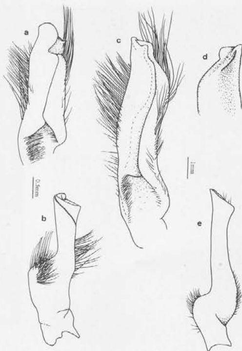
FIG. 2. Latreillopsis bispinosa Henderson, 1888, ♂, QM W10804; a — first male pleopod, abdominal view; b — second male pleopod, abdominal view; Paromola japonica Parisi, 1915, ♂, QM W10710; c — first male pleopod, abdominal view; d — sternal view of same (setae not shown); e — second male pleopod, abdominal view.
