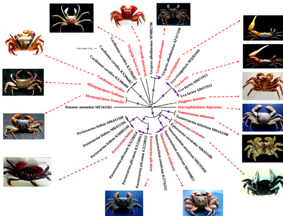
Fig. 4: Neighbour-joining tree was drawn using Kimura-2 parametric distance model. Species marked in red and black were sequences of this study and reference Genbank sequences (with accession numbers), respectively. Bootstrap values >70 were shown in purple circles. Penaeus monodon (Genbank Acc. No.: 563565) used as an out-group. Species without reference sequences in the phylogram indicates the first-time barcoded species.
