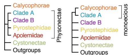
Figure 3: (A) Maximum likelihood (ML) phylogram with bipartition frequencies from the ML bootstraps and the Bayesian posterior distribution of trees. Unlabeled nodes have support >0.99 for both bootstraps and posteriors. The numbers of valid described species estimated to be in each clade based on taxonomy are shown below each clade name on the right. (B) The topologies found in the posterior distribution of trees that conflict with the ML tree. (C) The topologies evaluated by the SOWH tests. For more details on the SOWH topologies refer to Fig. S2.
