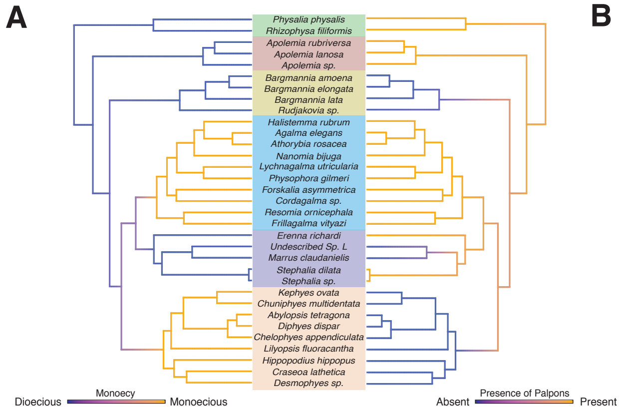
Figure 5: Stochastic mapping reconstruction of the evolutionary history of A) sexual mode, whether a colony is monoecious or dioecious and B) presence/absence of palpons (modified reduced gastrozooids). The color gradients show the reconstructed probability estimate of the discrete character states along the branches. Intermediate values reflect uncertainty.
