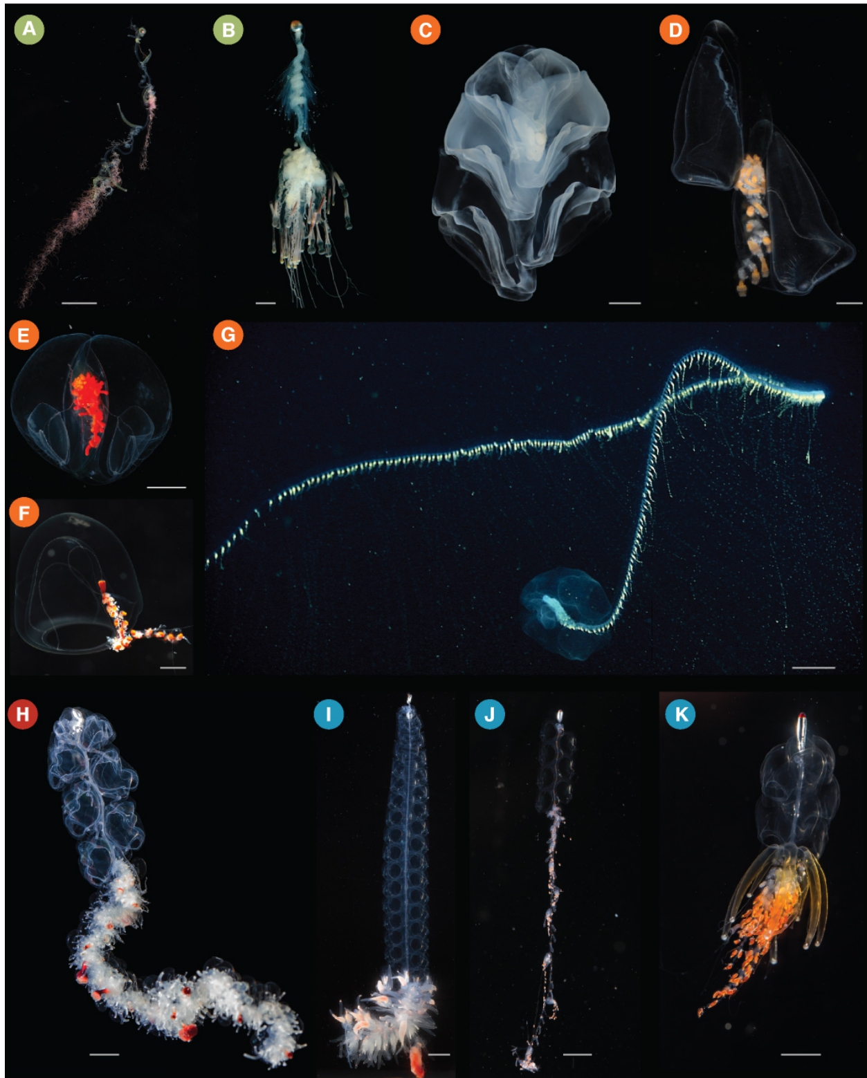
Figure 1: Photographs of living siphonophores. They correspond to the clades shown in Figure 3 as follows: Cystonectae (A-B), Calycophorae (C-G), Apolemiidae (H), and Clade A within Euphysonectae (I-K). (A) Rhizophysa eysenhardtii , scale bar = 1 cm. (B) Bathypphysa conifera , scale bar = 2cm. (C) Hippopodius hippopus , scale bar = 5 mm. (D) Kephyes hiulcus , scale bar = 2 mm. (E) Desmophyes haematogaster , scale bar = 5 mm. (F) Sphaeronectes christiansonae , scale bar = 2 mm. (G) Praya dubia , scale bar = 4 cm. (H) Apolemia sp., scale bar = 1 cm. (I) Lychnagalma utricularia , scale bar = 1 cm. (J) Nanomia sp., scale bar = 1 cm. (K) Physophora hydrostatica , scale bar = 5 mm. Photo credits: S. Siebert (C,H,I,K), S. Haddock (A,D,E,F), R. Sherlock (B), MBARI (G), C. Munro (J)
