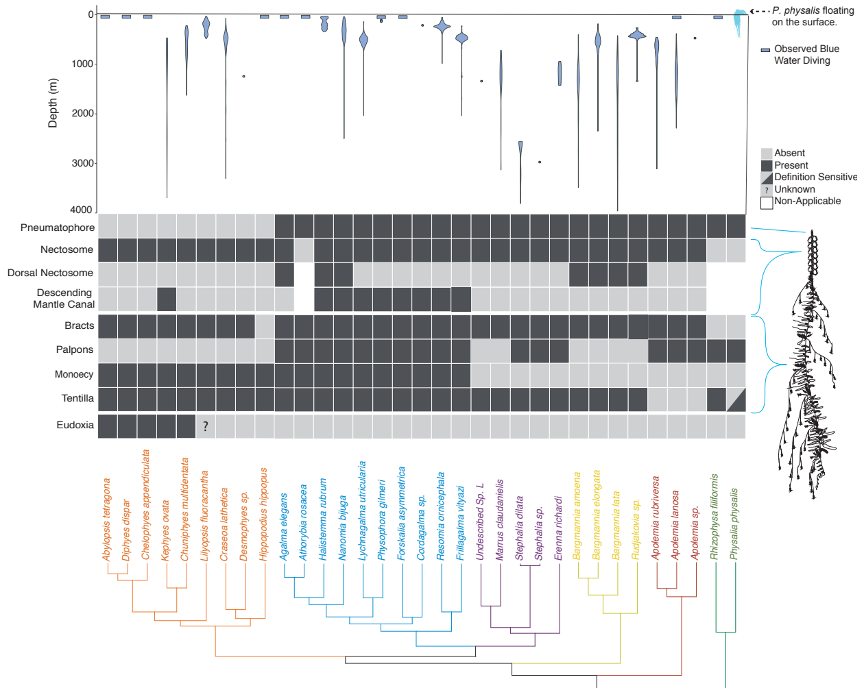
Figure 4: Siphonophore phylogeny showing the distribution of the main anatomical characters and the bathymetric distributions of the different species. Bottom: siphonophore phylogeny, colored by clade. Middle panel: diagram showing the presence/absence of traits across Siphonophora, with the physical location of the trait shown on a schematic of Nanomia bijuga (schematic by Freya Goetz). Top: Bathymetric distribution of siphonophore species. Physalia illustration by Noah Schlottman, taken from http://phylopic.org/
