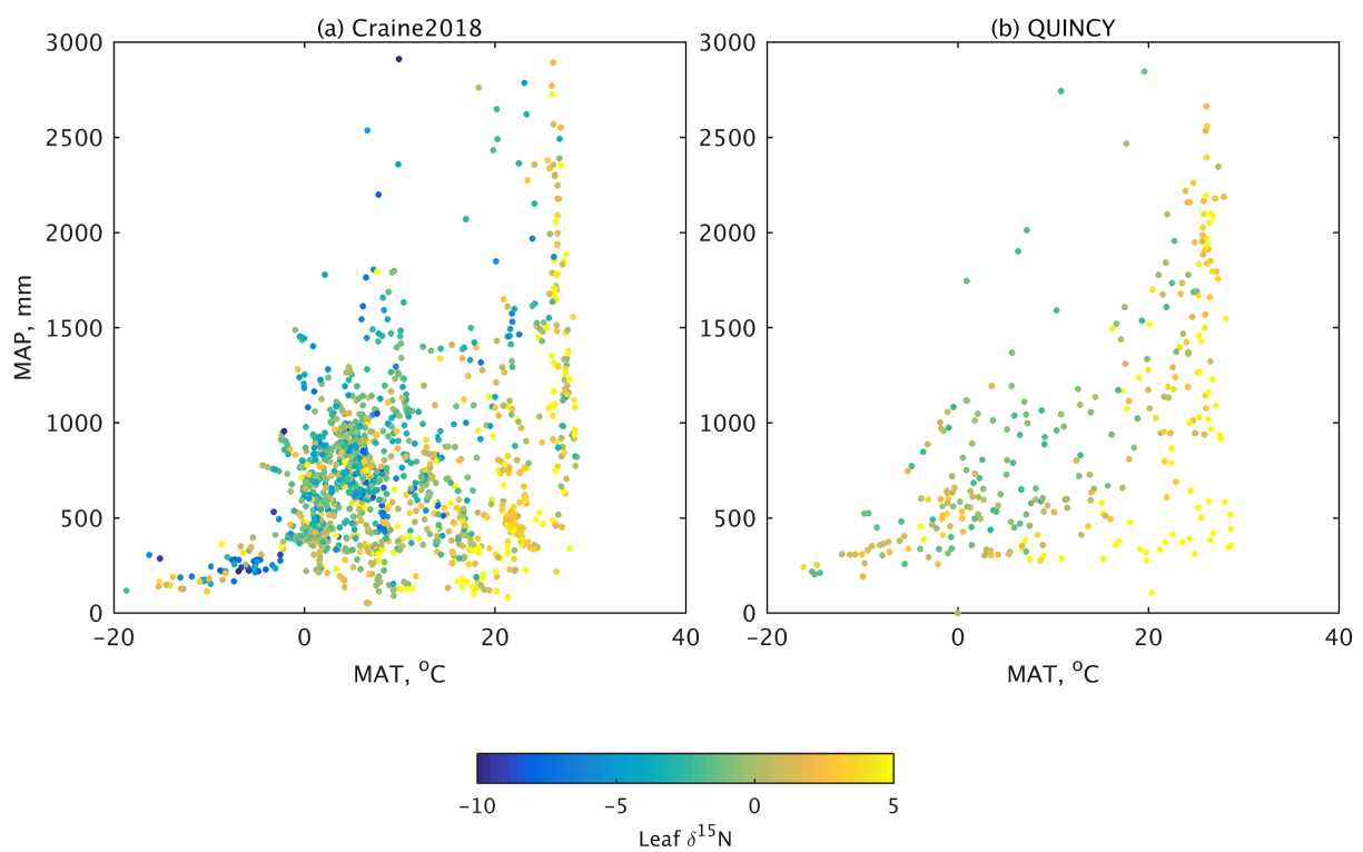
Figure S2 - Distribution of absolute values of leaf \delta^{15}\text{N} across climate regions for (a) the Craine 2018 dataset and (b) the QUINCY model.
