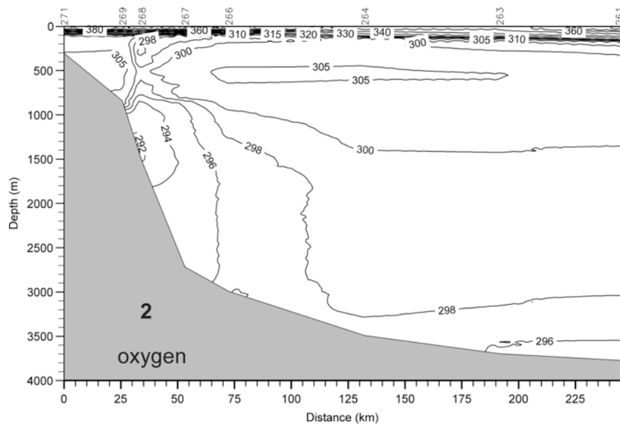
Fig. 4.1.3c: Distribution of oxygen ( \mu\text{mol/kg} ) along section 2 (see Fig. 4.1.1 for location)
