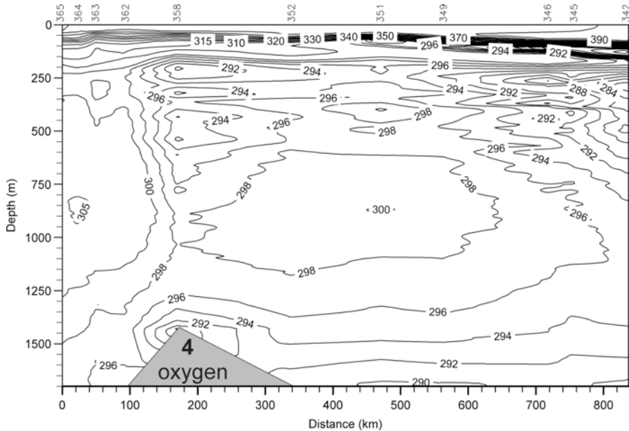
Fig. 4.1.5c: Distribution of oxygen ( \mu\text{mol/kg} ) along section 4 (see Fig. 4.1.1 for location)
