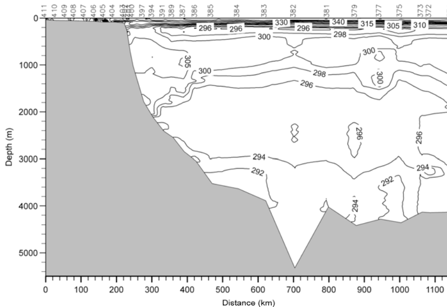
Fig. 4.1.6c: : Distribution of oxygen ( \mu\text{mol/kg} ) along section 5 (see Fig. 4.1.1 for location)
