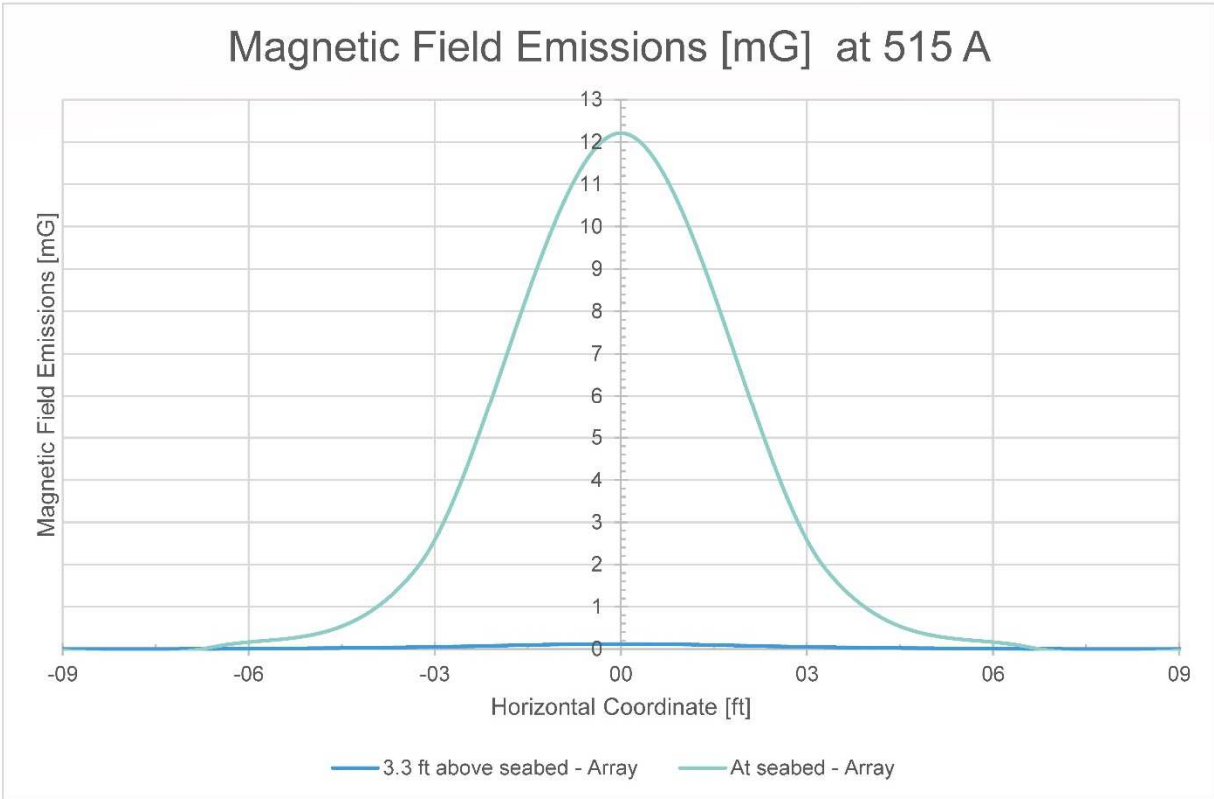
Figure 2.2.5-6 - Magnetic field emissions of the Ocean Wind array cables (515 Ampere [A]) related to distance at the seabed and 1 m above the seabed.
