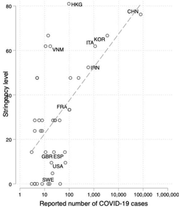
Figure 4: Stringency-Risk Ratio
