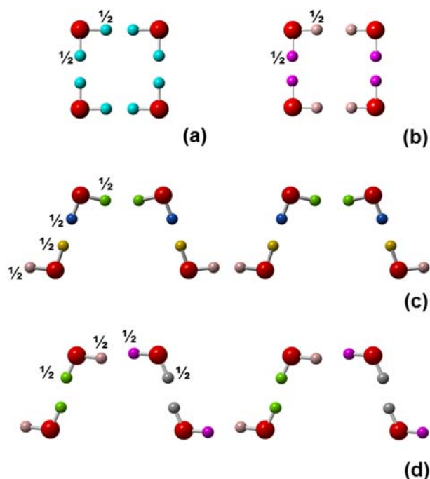
FIG. 25. Hydrogen bonding topologies of hydroxide perovskites determined by single-crystal XRD. Isolated 4-membered rings in (a) söhngteite \text{Ga}(\text{OH})_3 ( P4_2/nmc ) and (b) burtite ( Pn\bar{3} ). Crankshafts in (c) söhngteite \text{Ga}(\text{OH})_3 and (d) stottite \text{FeGe}(\text{OH})_6 ( P4_2/n ). All H sites are half-occupied in the averaged structure determined by diffraction methods. The number of non-equivalent OH groups in söhngteite (five) and stottite (six) have been confirmed by Raman spectroscopy. In the ring of söhngteite the pairs of H sites are mirror-related, whereas they are non-equivalent in stottite which being a double-perovskite lacks mirror symmetry.
