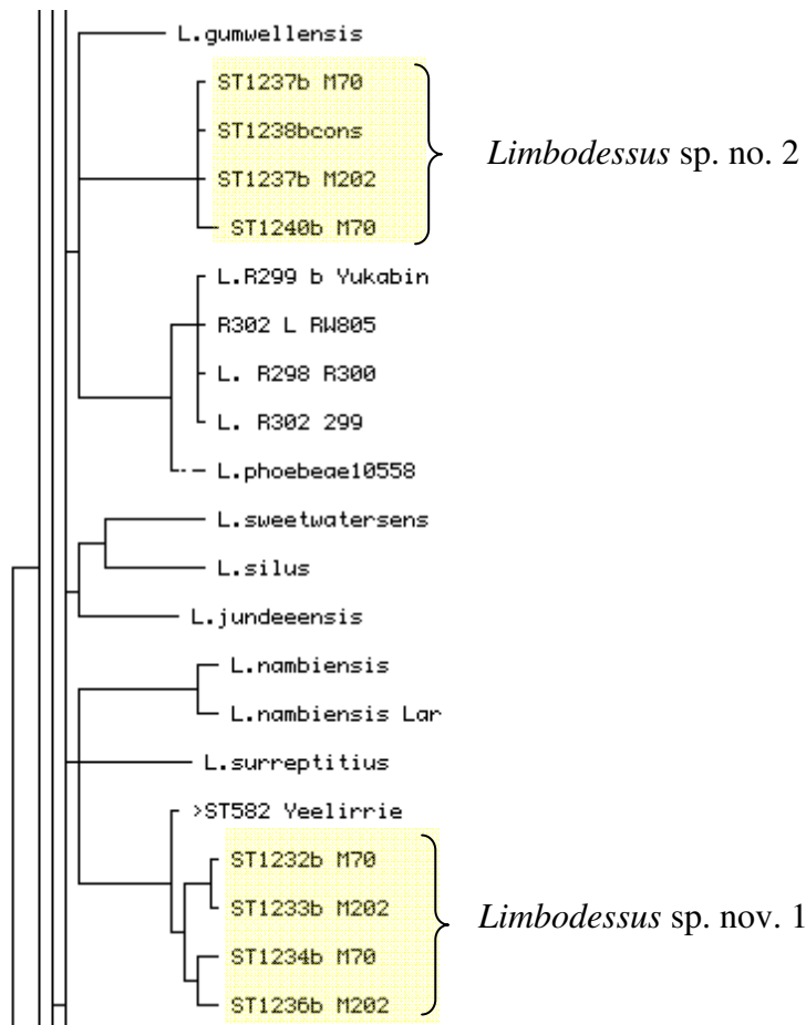
Figure 3. Partial neighbourjoining phylogram of Limbodessus (Dytiscidae).
