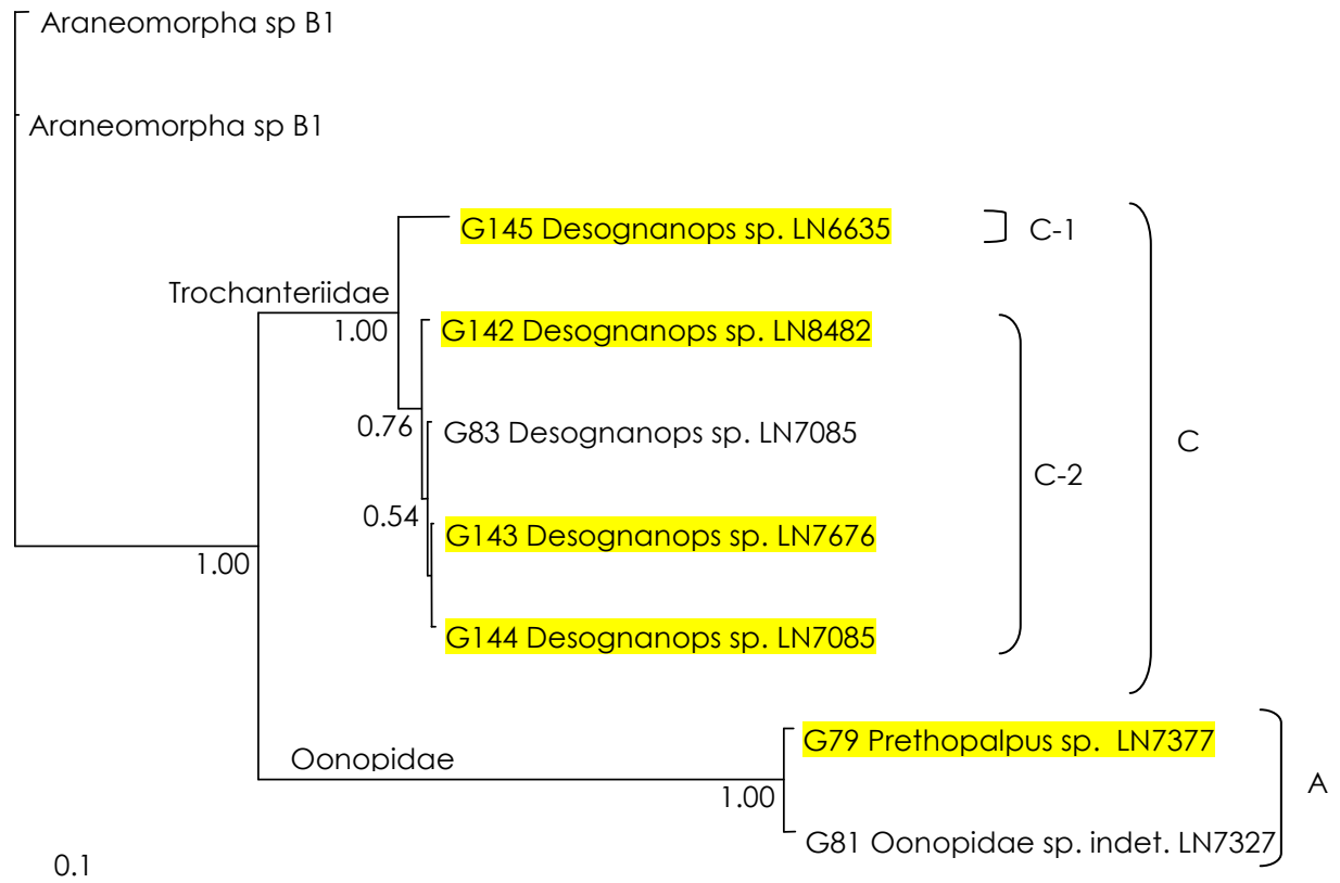
Figure 2. Bayesian analysis of 12s haplotypes of Yeelirrie araneomorphs. Lineages are labelled as in text and Tables. Numbers on nodes correspond to posterior probabilities. New Yeelirrie specimens are highlighted in yellow.
