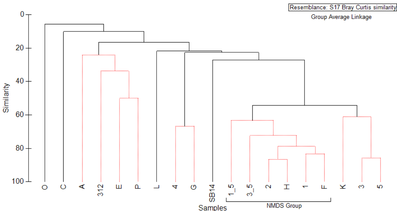
Figure 6-6: Cluster analysis of stygofauna assemblages, comparisons between drill lines. The SIMPROF test indicates those drill lines that do not contain significantly different assemblages, shown by the red lines.
