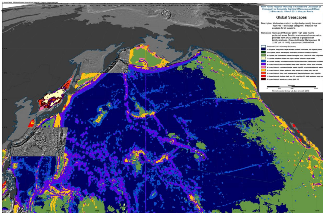
Figure 4.6-1 Global Seascapes
