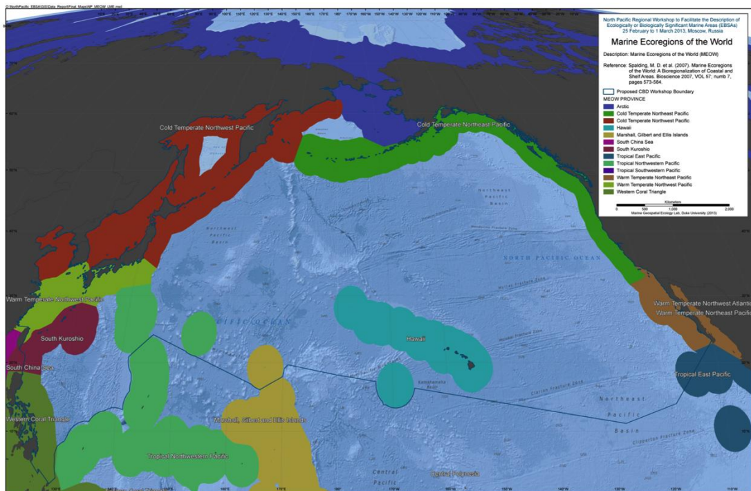
Figure 2.2-1 MEOW Provinces
