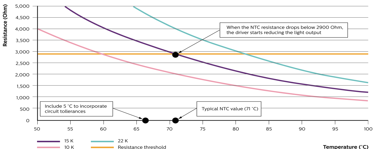
NTC resistance as function of temperature
