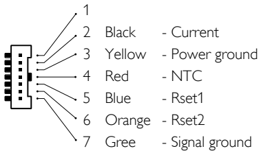
JST connector (driver side) pin layout
