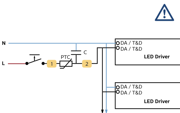
Schematic of Touch and Dim behaviour
