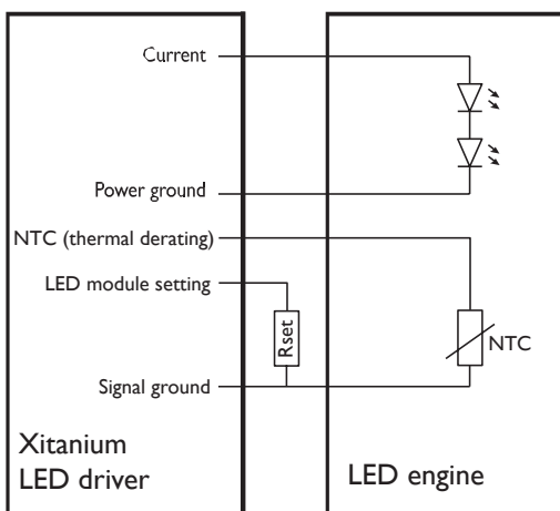
Schematically representation of the driver's output interfaces
