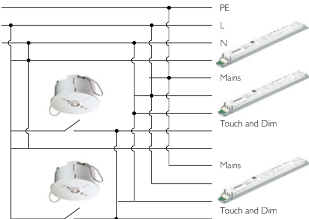
Connecting a sensor to the Dali input to utilize Corridor Mode
