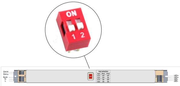
DipSwitch on driver
