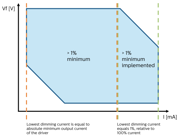
Minimum dimming output current
