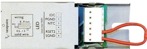
Example of an insulated Rset
