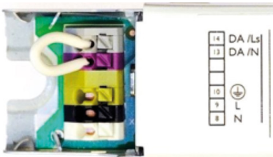
Example of a shorted DALI interface
