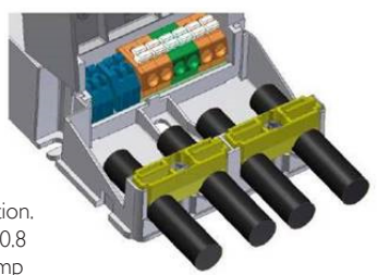
Strain relief blocks for the /m driver for independent application
