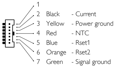
JST connector (driver side) pin layout 75 W & 110 W
