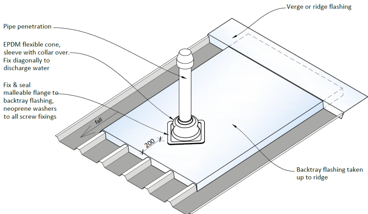
Figure 10-2 Typical Roof Pipe Penetration
