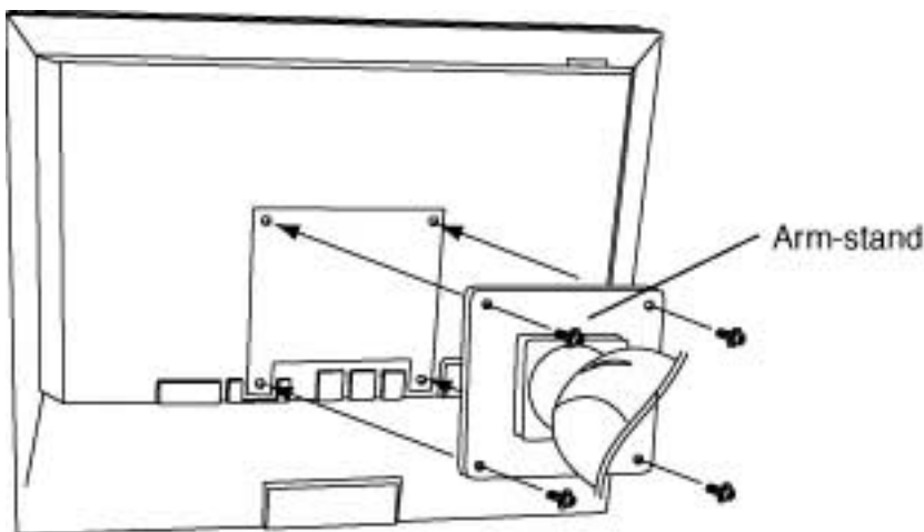
M4 Mounting Screws: M4 x 15 (mm) BZn/Fe
