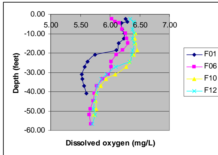
Figure 3. Oxygen Profiles – Fernandina ODMDS, August 2005
