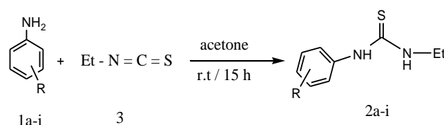
Scheme 1. Synthesis of thioureas 2a-i from aromatic amines 1a-i
